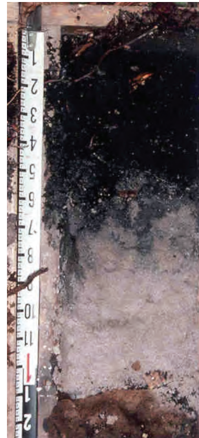
Figure 20. In this soil, the splotchy pattern below the dark surface is due to mobilization and translocation of organic matter. Scale is in inches.
