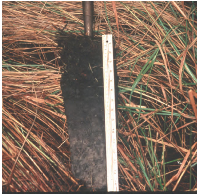
Figure 15. The mucky modified sandy layer is approximately 3 in. (7.5 cm) thick. Scale in inches on the right side of ruler.
