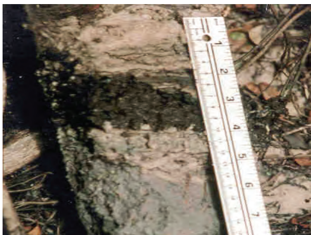
Figure 10. Stratified layers in loamy material.
