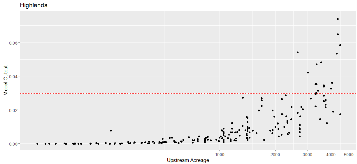
Figure 11: Scatterplot of upstream acreage vs. model output (Highlands)
