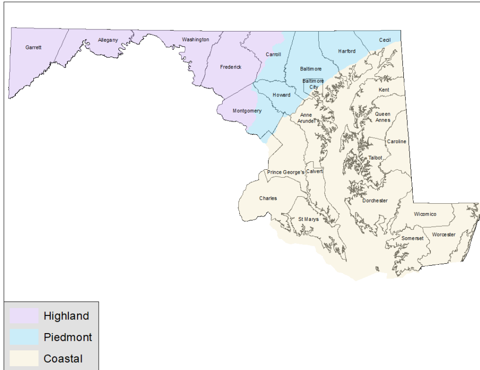
Figure 2: Maryland Ecoregions
