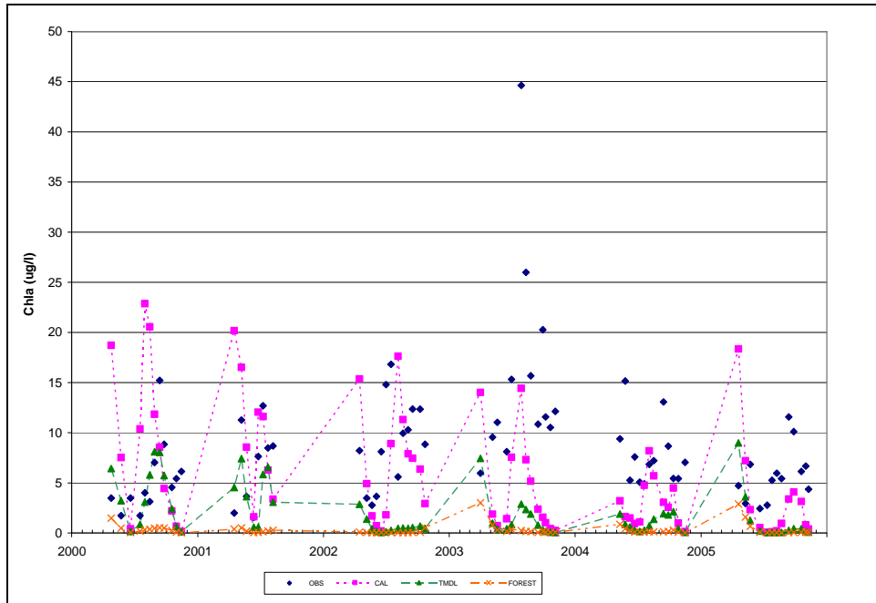
Figure E-2: Maximum Chla, Observed Data and All Scenarios, NPA0059, Liberty Reservoir
