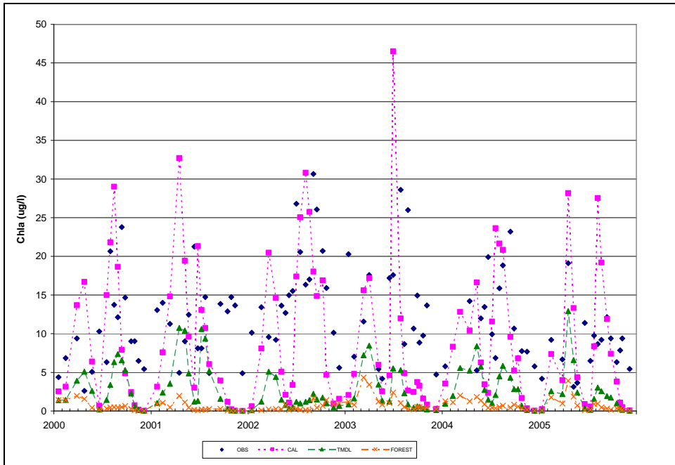
Figure E-4: Maximum Chla, Observed Data and All Scenarios, NPA0105, Liberty Reservoir
