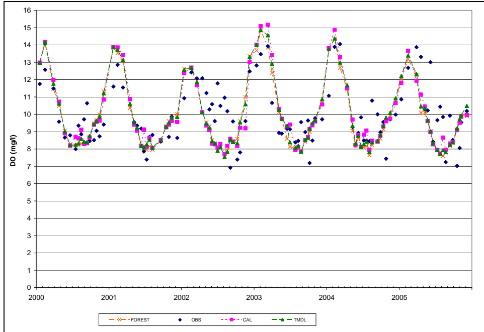
Figure E-7: Surface DO, Observed Data and All Scenarios, NPA0105, Liberty Reservoir
