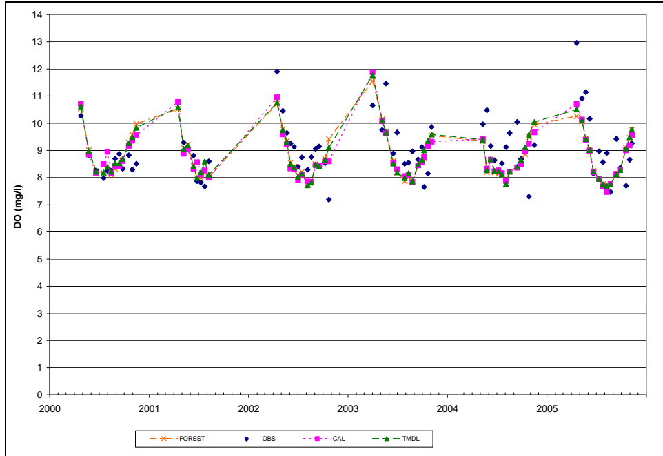
Figure E-5: Surface DO, Observed Data and All Scenarios, NPA0059, Liberty Reservoir
