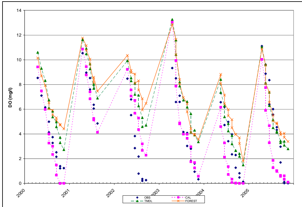
Figure E-8: Bottom DO, Observed Data and All Scenarios, NPA0059, Liberty Reservoir
