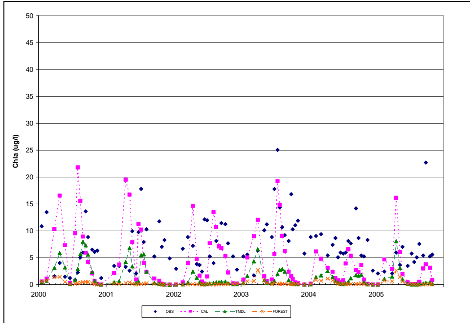
Figure E-1: Maximum Chla, Observed Data and All Scenarios, NPA0042, Liberty Reservoir
