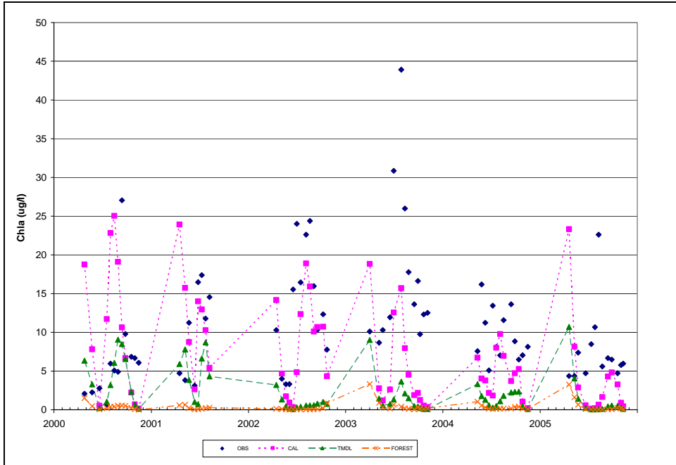
Figure E-3: Maximum Chla, Observed Data and All Scenarios, NPA0067, Liberty Reservoir
