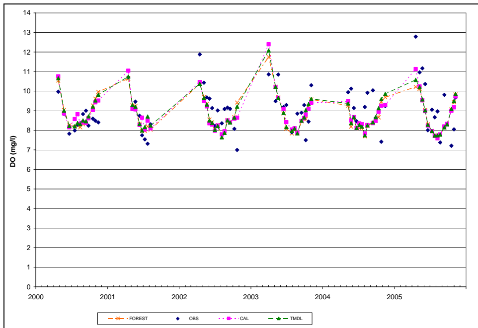
Figure E-6: Surface DO, Observed Data and All Scenarios, NPA0067, Liberty Reservoir
