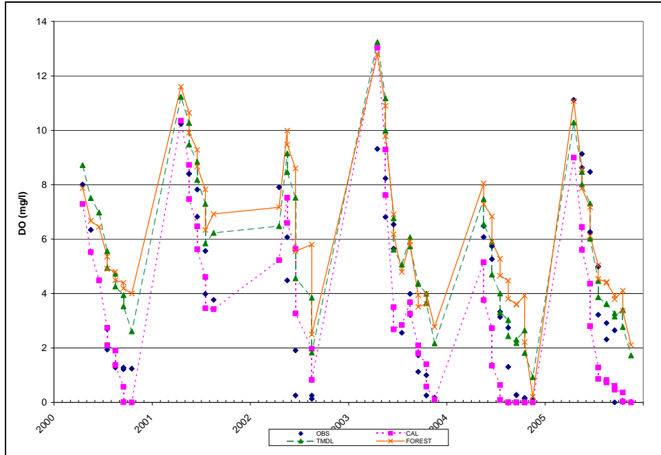
Figure E-9: Bottom DO, Observed Data and All Scenarios, NPA0067, Liberty Reservoir
