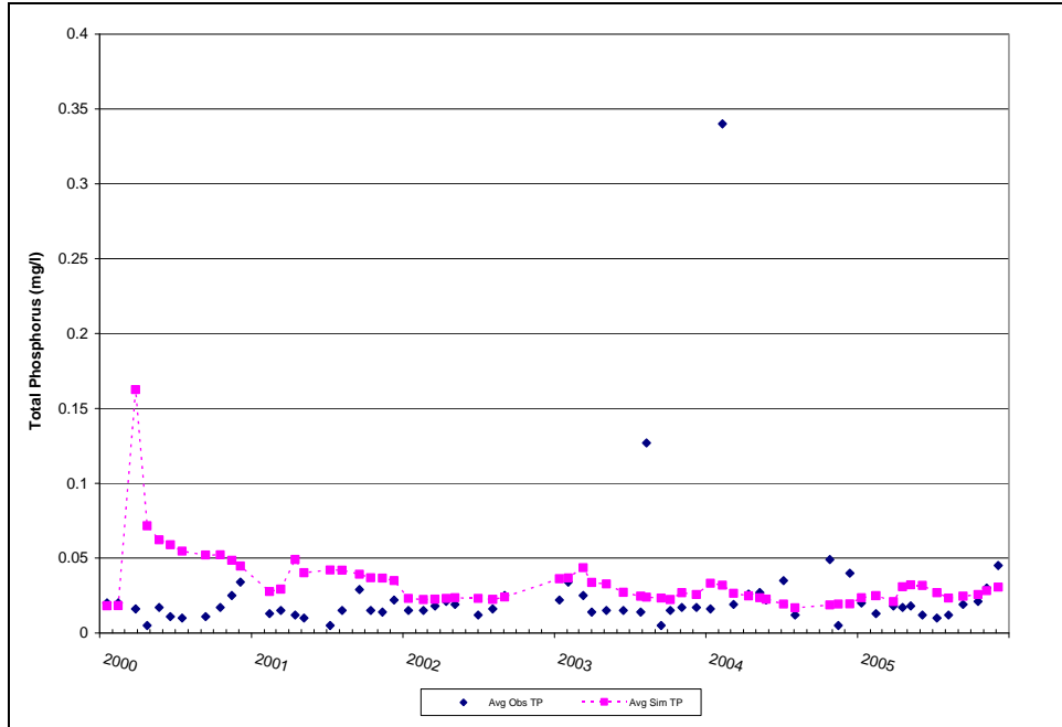
Figure D-7: Liberty Reservoir BCDPW Station NPA0042 Bottom Observed and Simulated (Calibration) TP Concentrations on Sampling Dates
