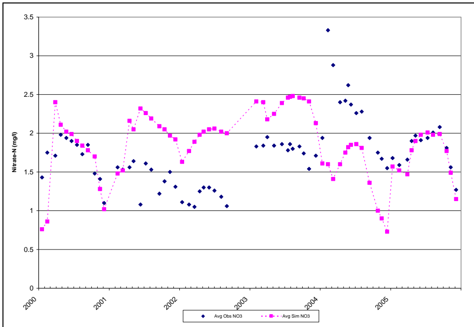
Figure D-32: Liberty Reservoir BCDPW Station NPA0042 Bottom Observed and Simulated (Calibration) NO3 Concentrations on Sampling Dates
