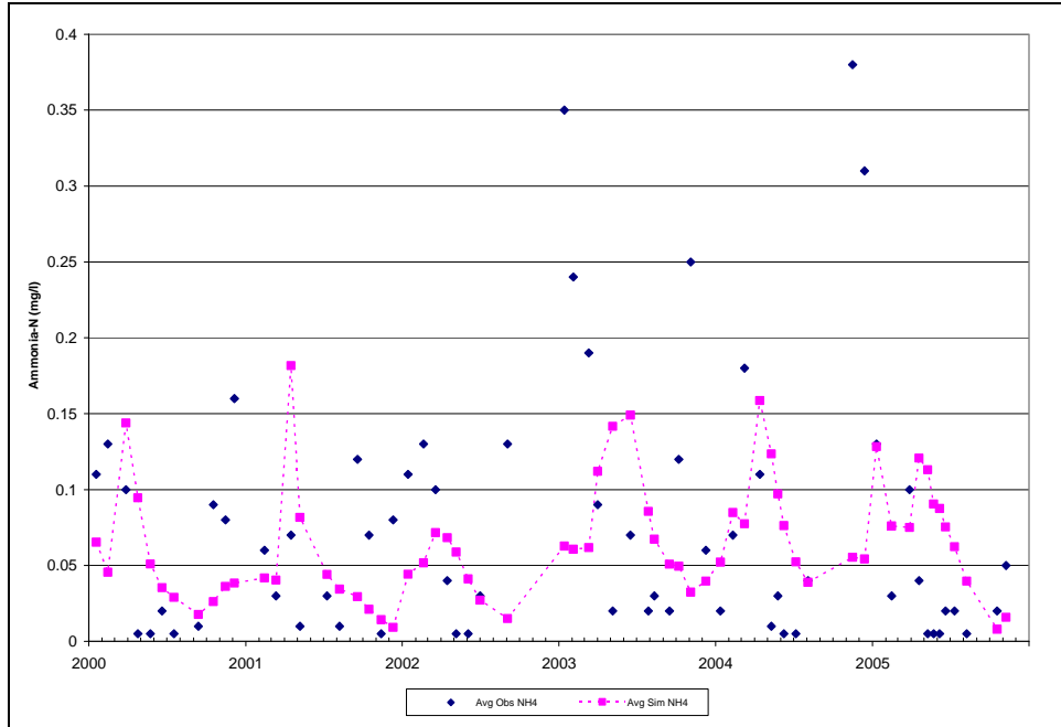
Figure D-25: Liberty Reservoir BCDPW Station NPA0042 Bottom Observed and Simulated (Calibration) NH4 Concentrations on Sampling Dates
