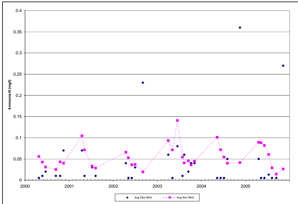
Figure D-24: Liberty Reservoir BCDPW Station NPA0059 Bottom Observed and Simulated (Calibration) NH4 Concentrations on Sampling Dates
