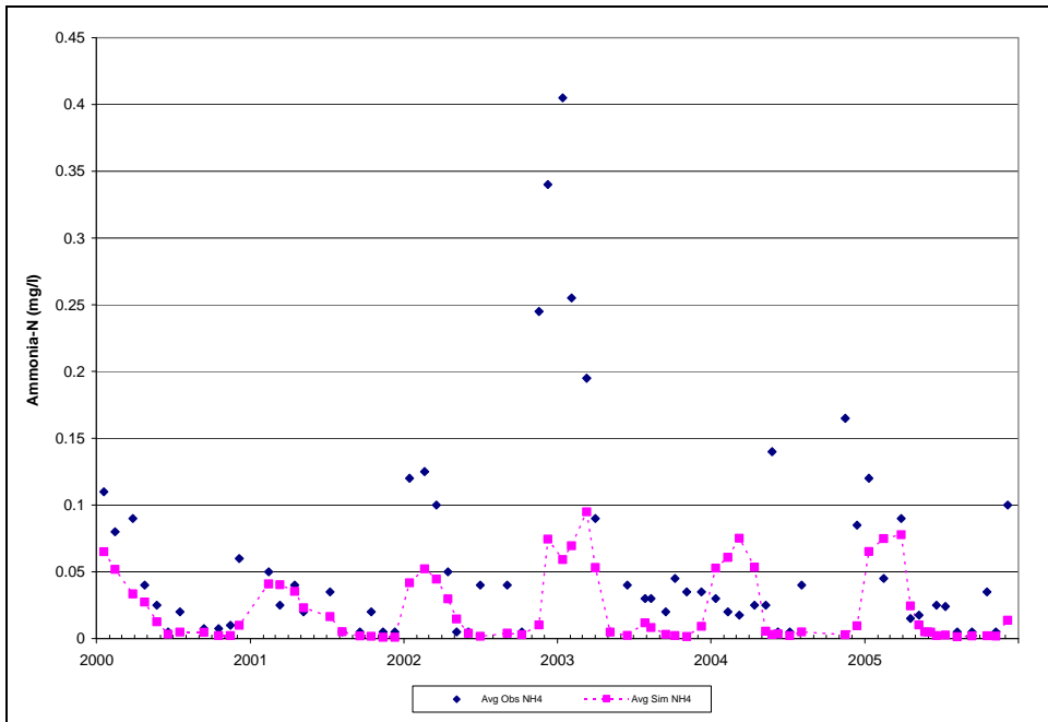
Figure D-22: Liberty Reservoir BCDPW Station NPA0042 Surface Observed and Simulated (Calibration) NH4 Concentrations on Sampling Dates
