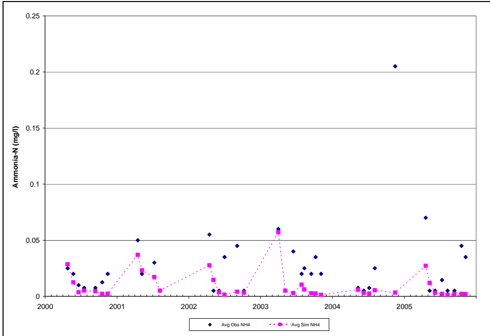
Figure D-21: Liberty Reservoir BCDPW Station NPA0059 Surface Observed and Simulated (Calibration) NH4 Concentrations on Sampling Dates
