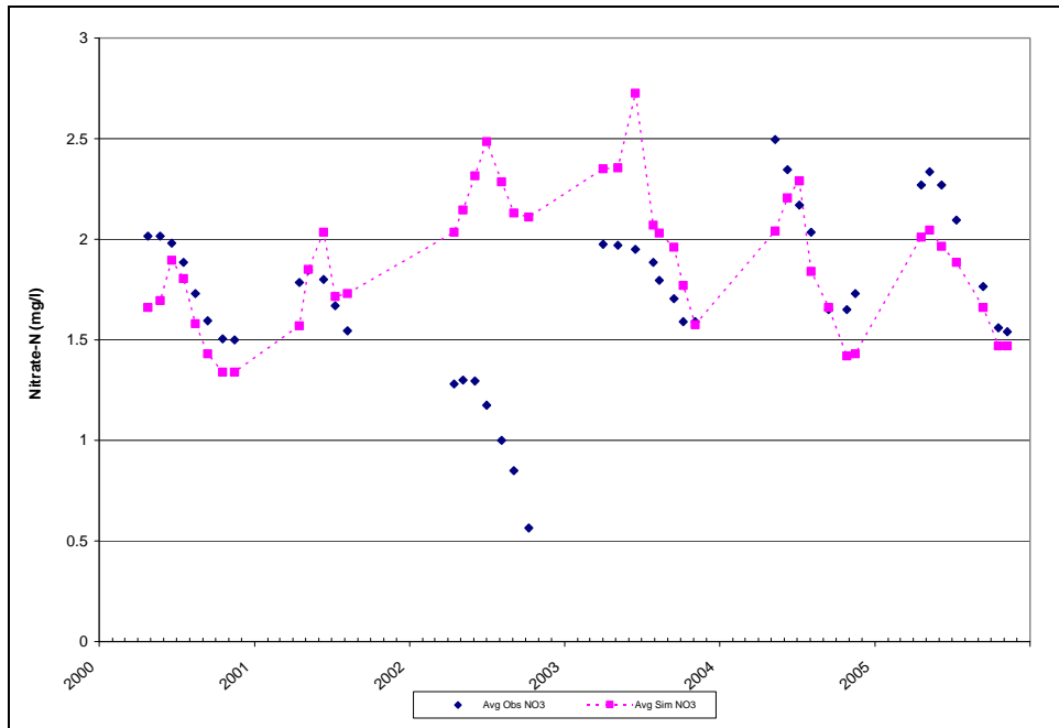
Figure D-28: Liberty Reservoir BCDPW Station NPA0059 Surface Observed and Simulated (Calibration) NO3 Concentrations on Sampling Dates
