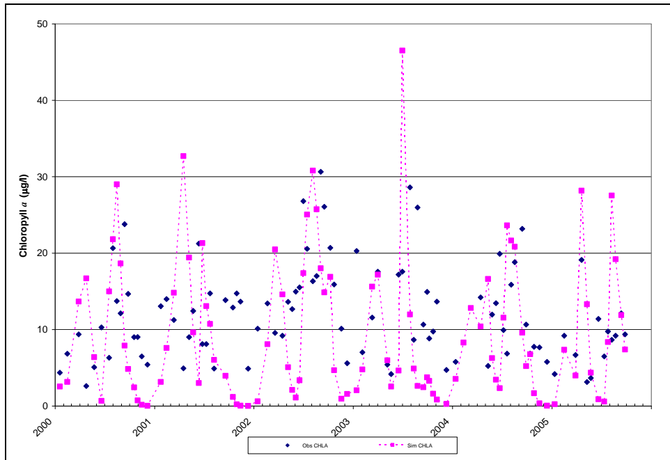
Figure D-8: Liberty Reservoir BCDPW Station NPA0105 Surface Observed and Simulated (Calibration) Chla Concentrations on Sampling Dates
