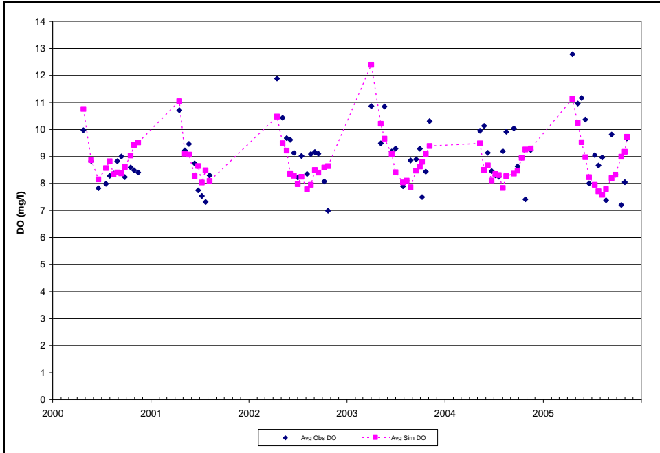
Figure D-13: Liberty Reservoir BCDPW Station NPA0067 Surface Observed and Simulated (Calibration) DO Concentrations on Sampling Dates
