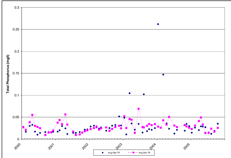
Figure D-1: Liberty Reservoir BCDPW Station NPA0105 Surface Observed and Simulated (Calibration) TP Concentrations on Sampling Dates
