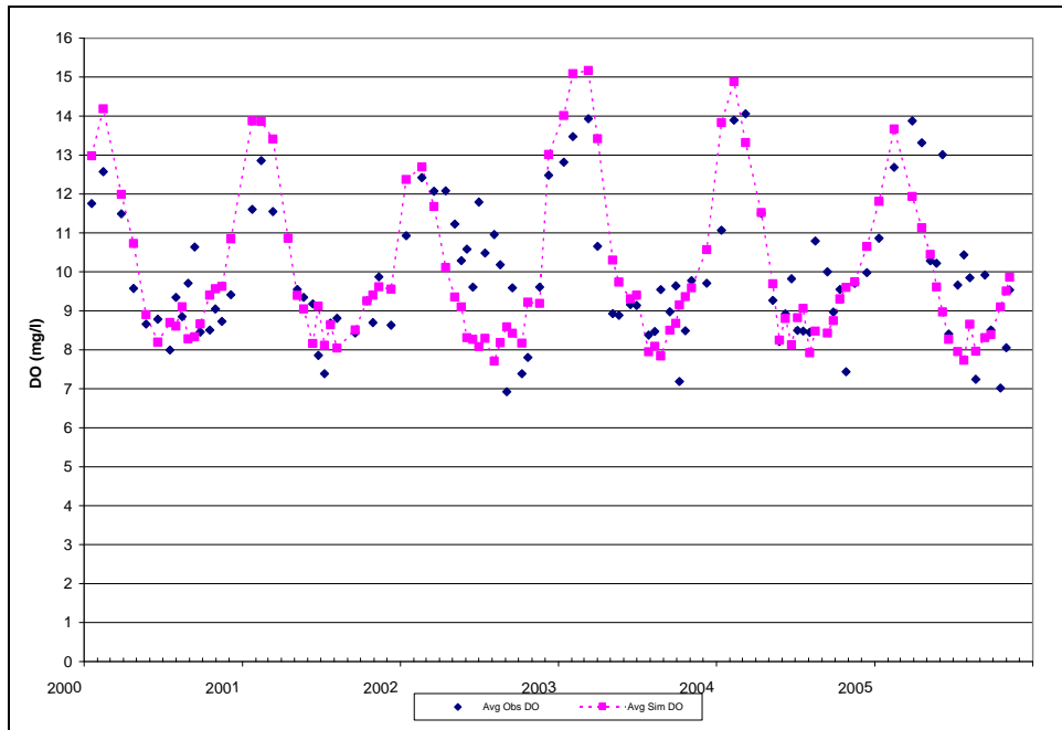
Figure D-12: Liberty Reservoir BCDPW Station NPA0105 Surface Observed and Simulated (Calibration) DO Concentrations on Sampling Dates
