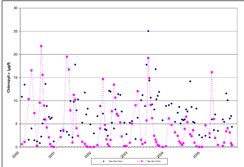
Figure D-11: Liberty Reservoir BCDPW Station NPA0042 Surface Observed and Simulated (Calibration) Chla Concentrations on Sampling Dates
