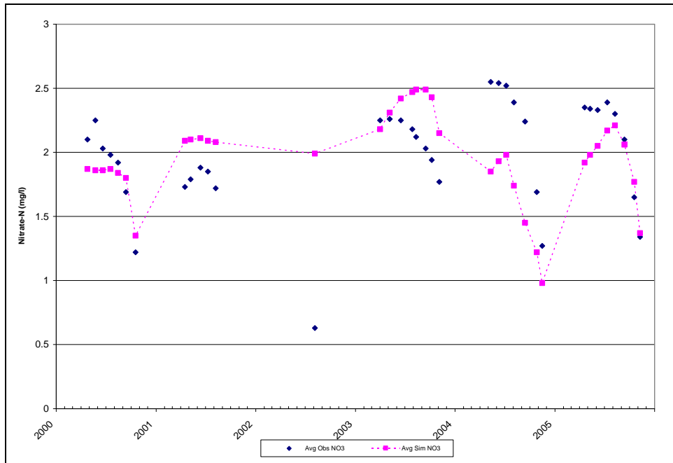
Figure D-30: Liberty Reservoir BCDPW Station NPA0067 Bottom Observed and Simulated (Calibration) NO3 Concentrations on Sampling Dates
