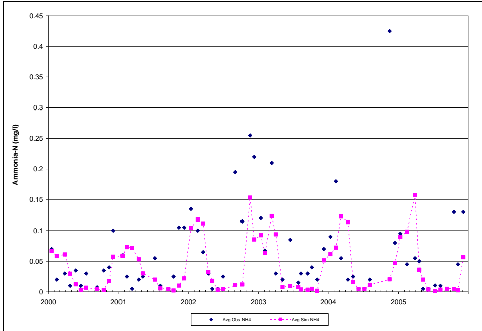
Figure D-19: Liberty Reservoir BCDPW Station NPA0105 Surface Observed and Simulated (Calibration) NH4 Concentrations on Sampling Dates
