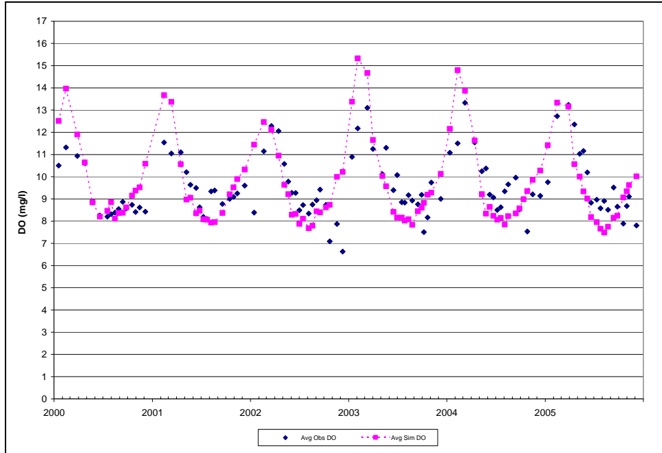
Figure D-15: Liberty Reservoir BCDPW Station NPA0042 Surface Observed and Simulated (Calibration) DO Concentrations on Sampling Dates
