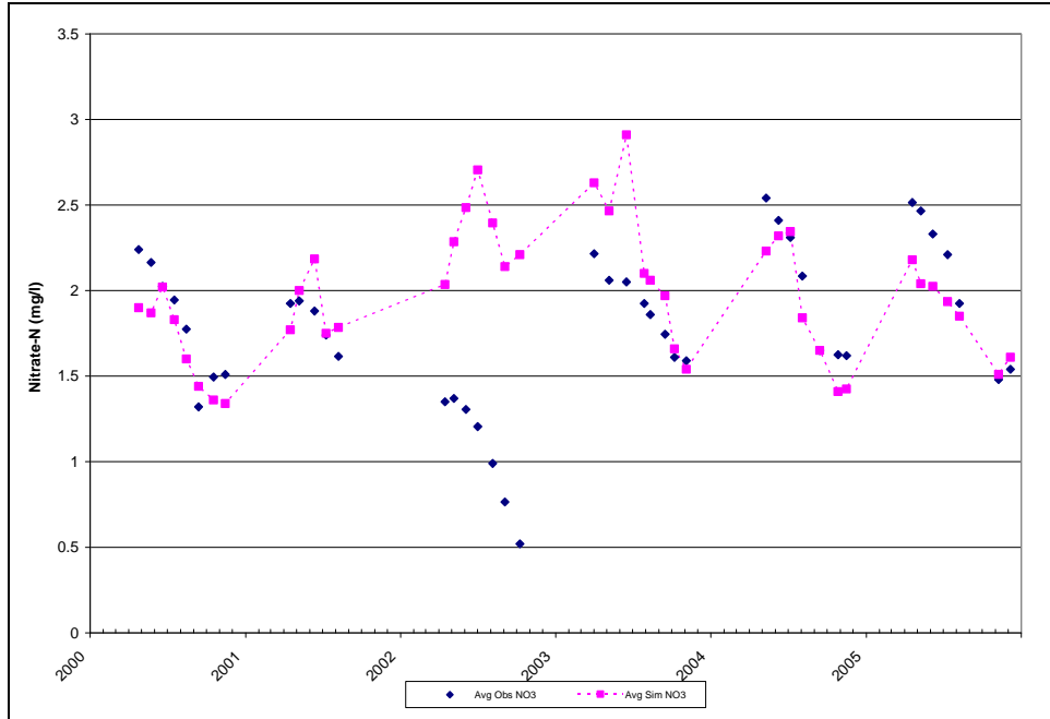
Figure D-27: Liberty Reservoir BCDPW Station NPA0067 Surface Observed and Simulated (Calibration) NO3 Concentrations on Sampling Dates
