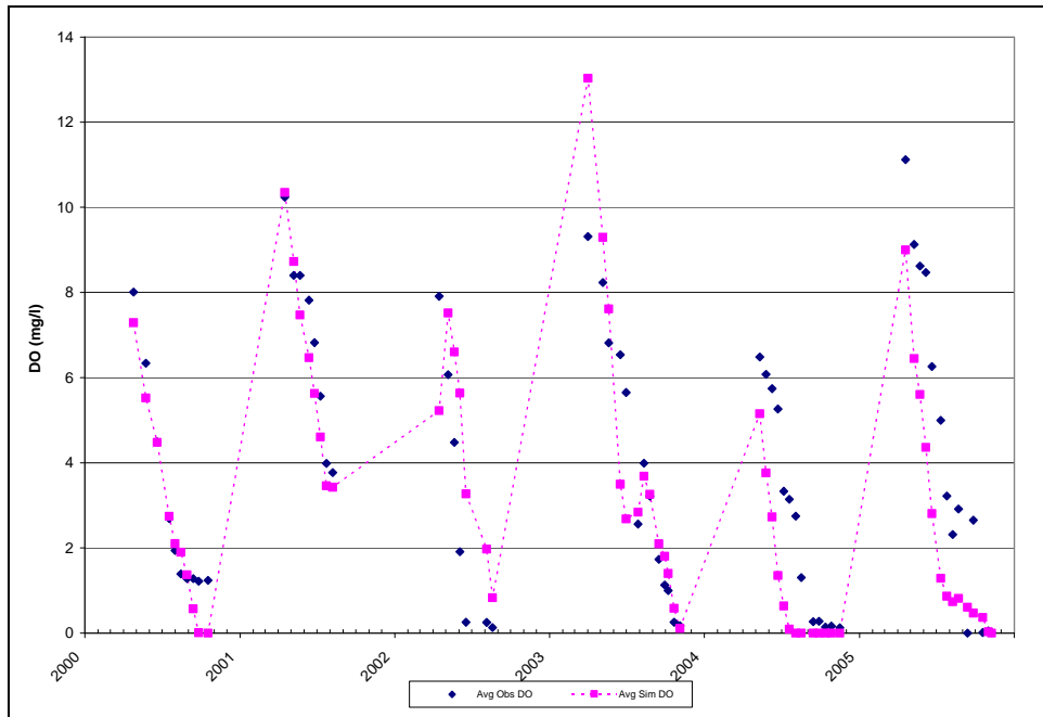
Figure D-16: Liberty Reservoir BCDPW Station NPA0067 Bottom Observed and Simulated (Calibration) DO Concentrations on Sampling Dates
