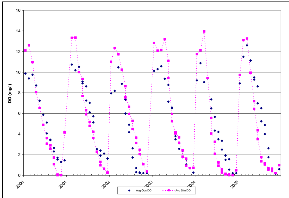
Figure D-18: Liberty Reservoir BCDPW Station NPA0042 Bottom Observed and Simulated (Calibration) DO Concentrations on Sampling Dates
