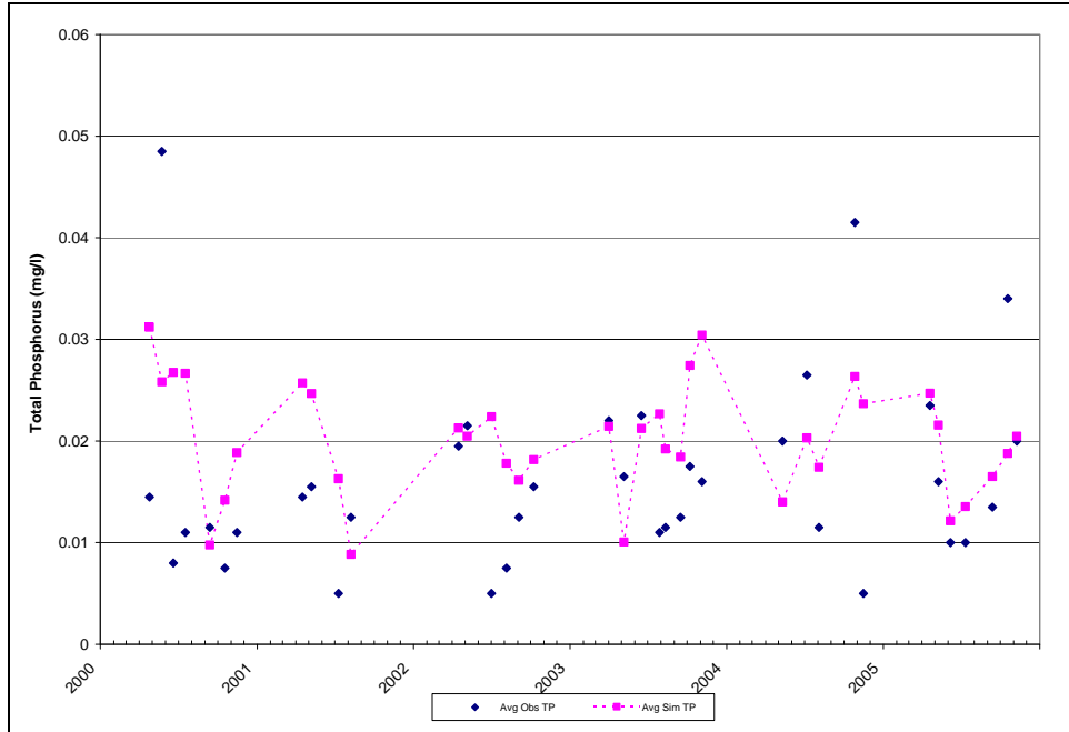
Figure D-3: Liberty Reservoir BCDPW Station NPA0059 Surface Observed and Simulated (Calibration) TP Concentrations on Sampling Dates
