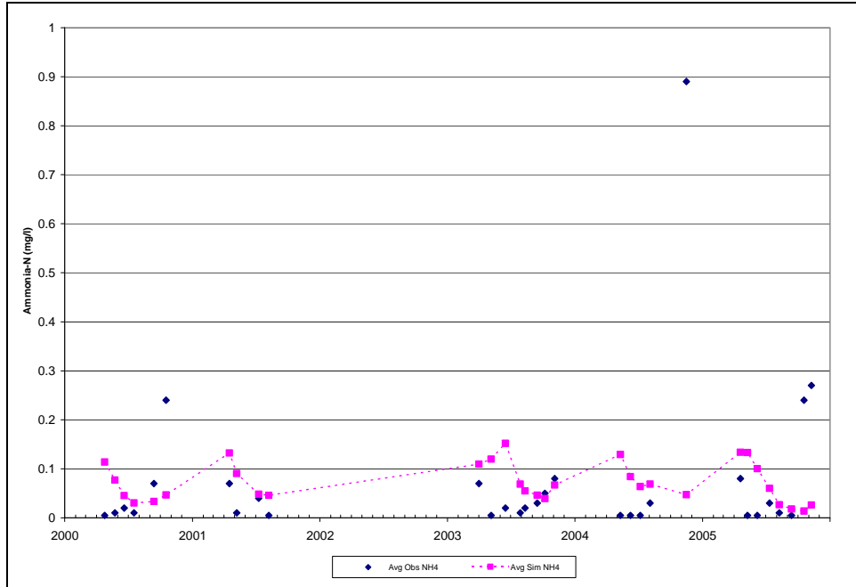
Figure D-23: Liberty Reservoir BCDPW Station NPA0067 Bottom Observed and Simulated (Calibration) NH4 Concentrations on Sampling Dates
