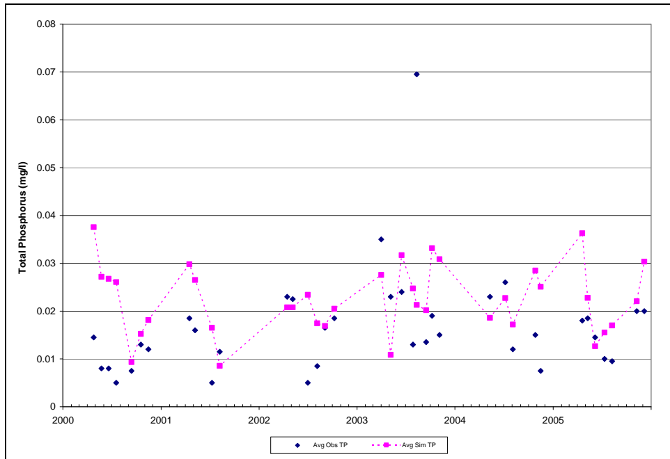
Figure D-2: Liberty Reservoir BCDPW Station NPA0067 Surface Observed and Simulated (Calibration) TP Concentrations on Sampling Dates
