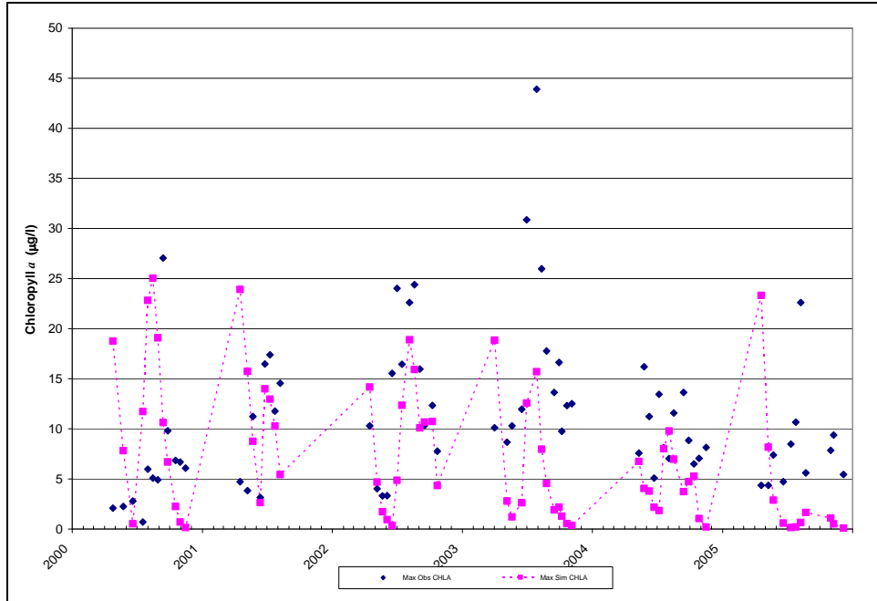
Figure D-9: Liberty Reservoir BCDPW Station NPA0067 Surface Observed and Simulated (Calibration) Chla Concentrations on Sampling Dates
