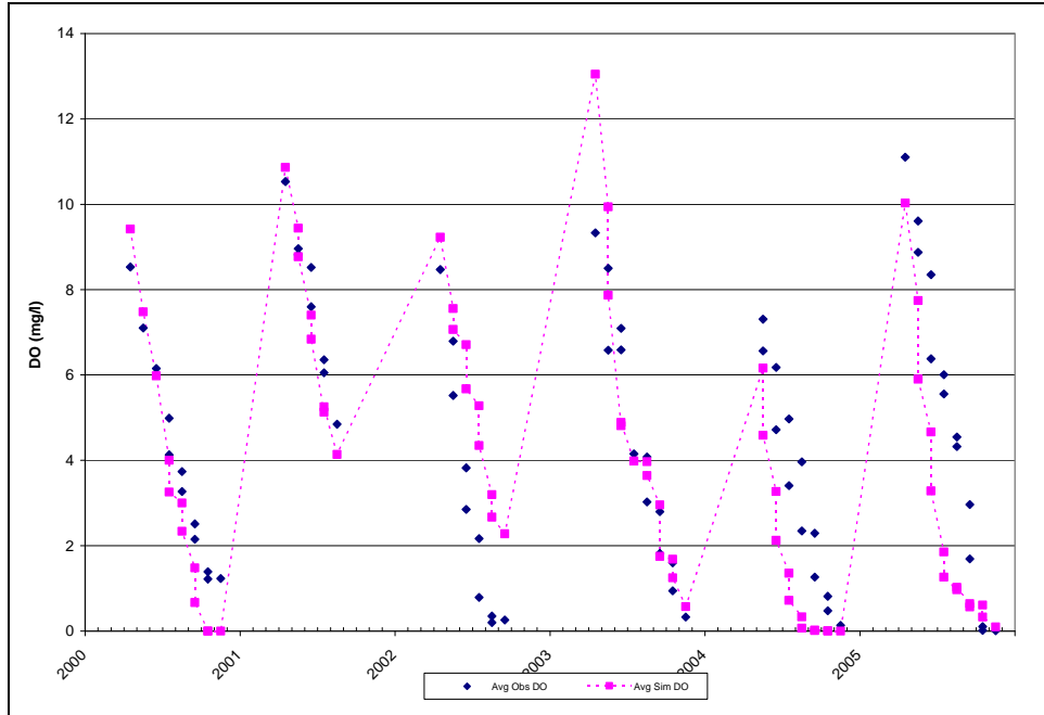
Figure D-17: Liberty Reservoir BCDPW Station NPA0059 Bottom Observed and Simulated (Calibration) DO Concentrations on Sampling Dates
