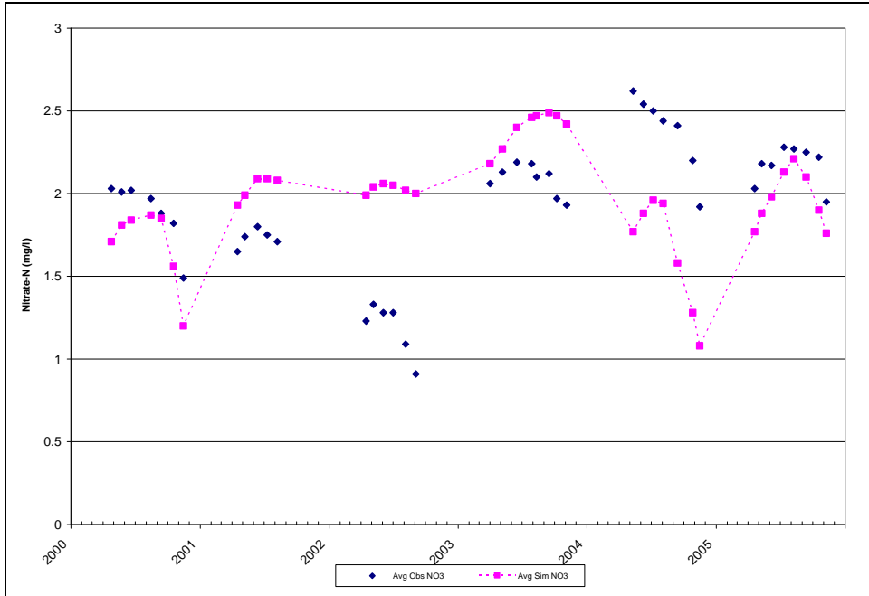
Figure D-31: Liberty Reservoir BCDPW Station NPA0059 Bottom Observed and Simulated (Calibration) NO3 Concentrations on Sampling Dates
