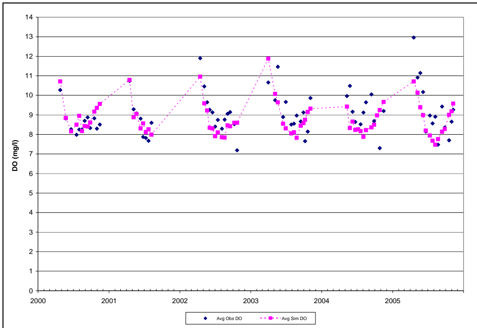
Figure D-14: Liberty Reservoir BCDPW Station NPA0059 Surface Observed and Simulated (Calibration) DO Concentrations on Sampling Dates
