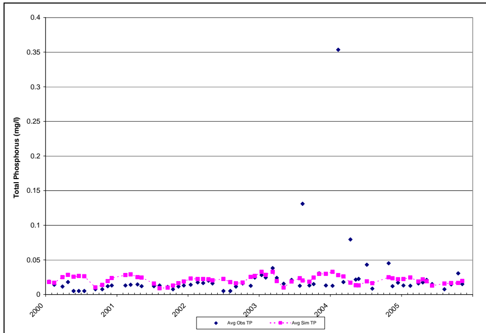
Figure D-4: Liberty Reservoir BCDPW Station NPA0042 Surface Observed and Simulated (Calibration) TP Concentrations on Sampling Dates
