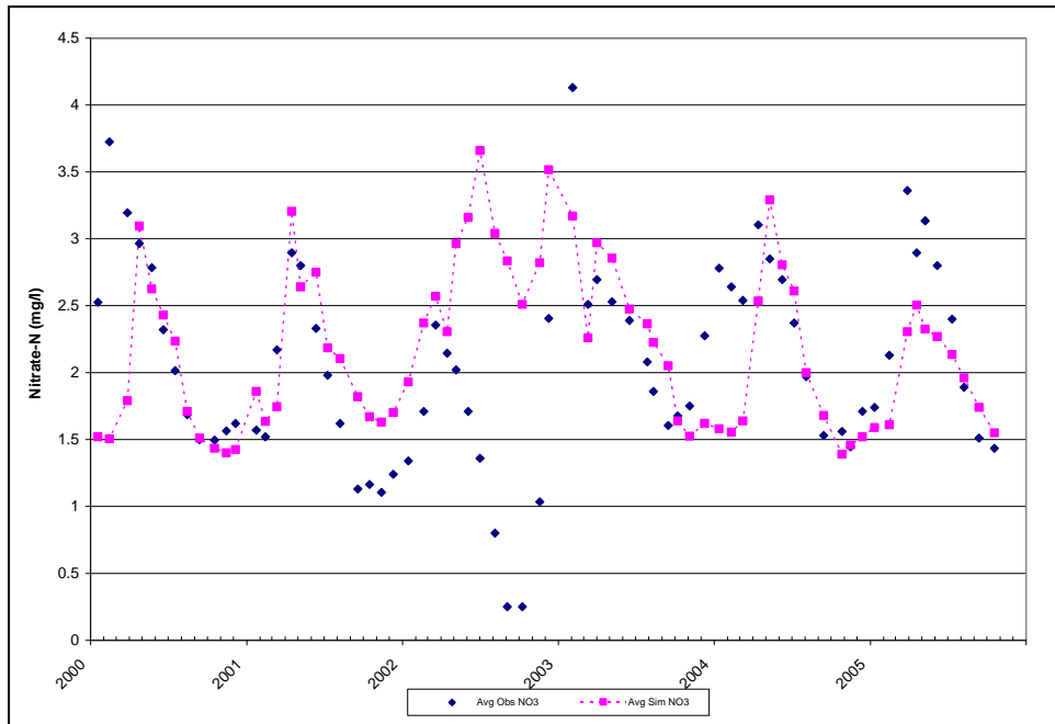
Figure D-26: Liberty Reservoir BCDPW Station NPA0105 Surface Observed and Simulated (Calibration) NO3 Concentrations on Sampling Dates
