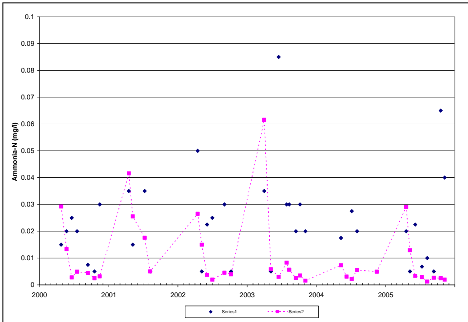
Figure D-20: Liberty Reservoir BCDPW Station NPA0067 Surface Observed and Simulated (Calibration) NH4 Concentrations on Sampling Dates
