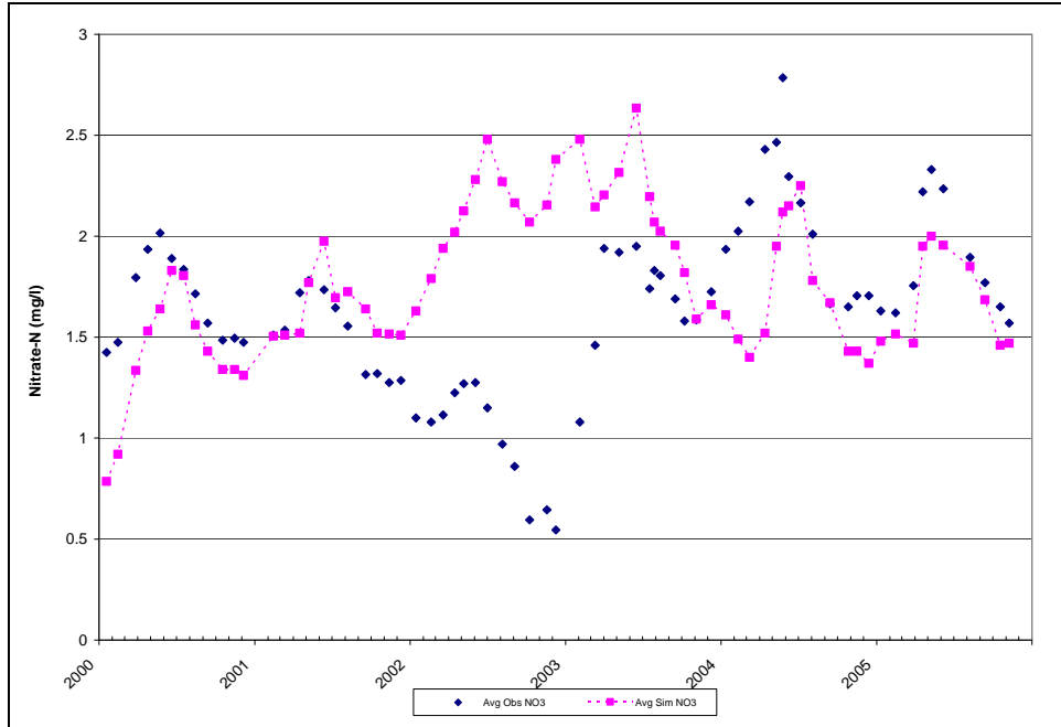
Figure D-29: Liberty Reservoir BCDPW Station NPA0042 Surface Observed and Simulated (Calibration) NO3 Concentrations on Sampling Dates
