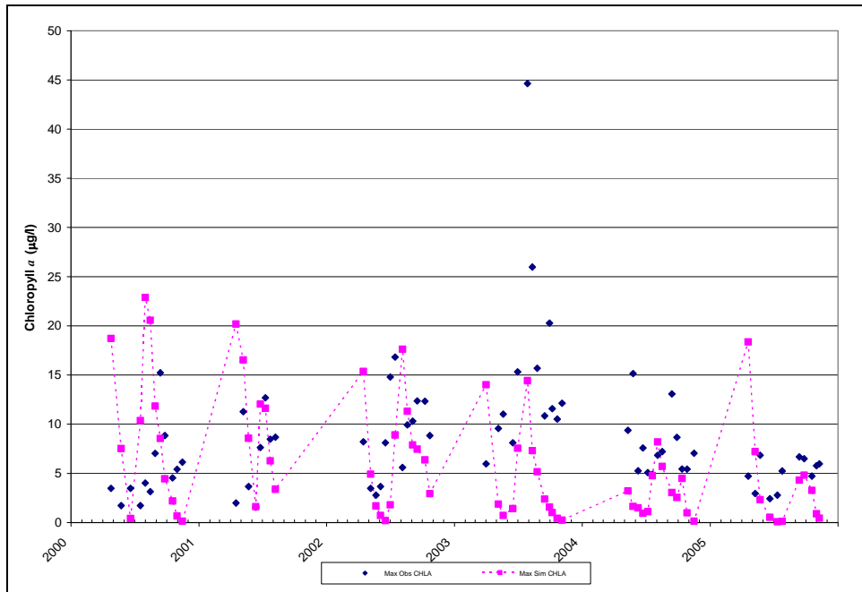
Figure D-10: Liberty Reservoir BCDPW Station NPA0059 Surface Observed and Simulated (Calibration) Chla Concentrations on Sampling Dates
