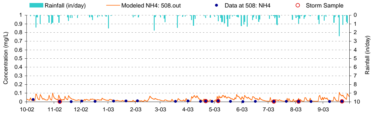
Figure I-2. Ammonium validation plot for Jennings Run (WM-30/JEN0036)
