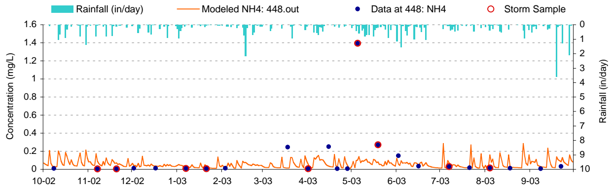
Figure I-1. Ammonium calibration plot for Georges Creek (WM-124/GEO0143)
