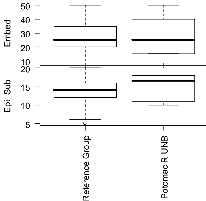
Figure 4: The Upper North Branch Potomac River Embeddedness and Epifaunal Substrate Compared to Reference Sites
