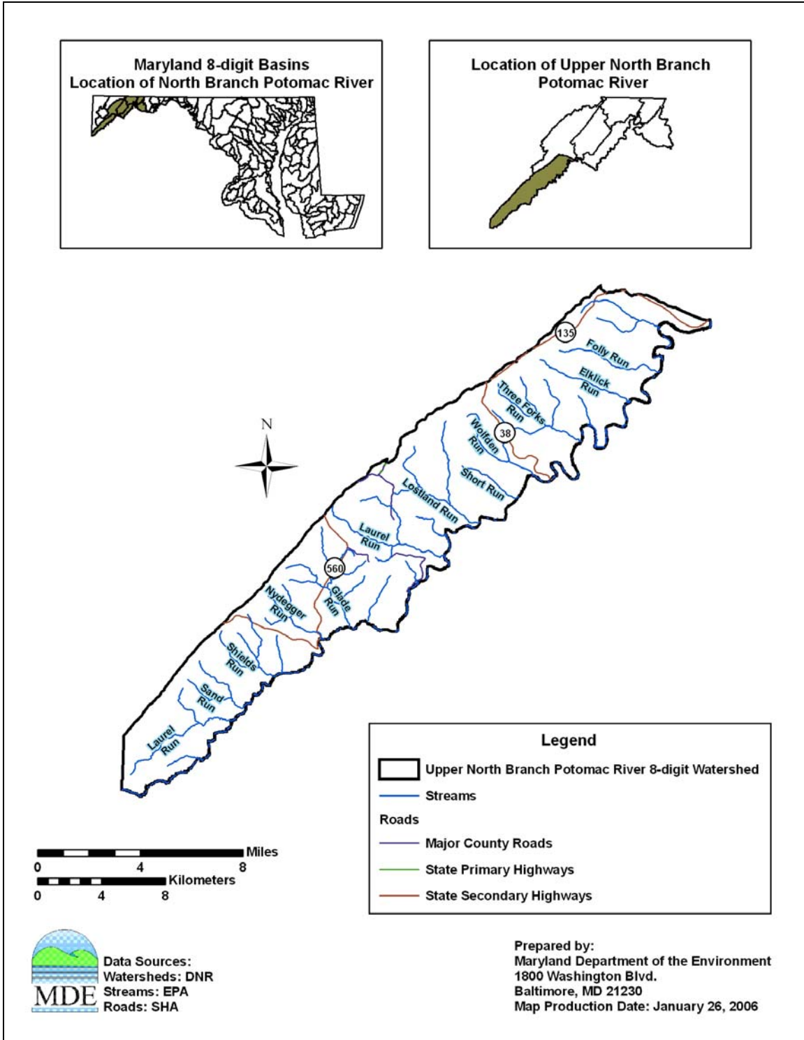
Figure 1: Location Map of the Maryland portion of the Upper North Branch Potomac River Watershed
