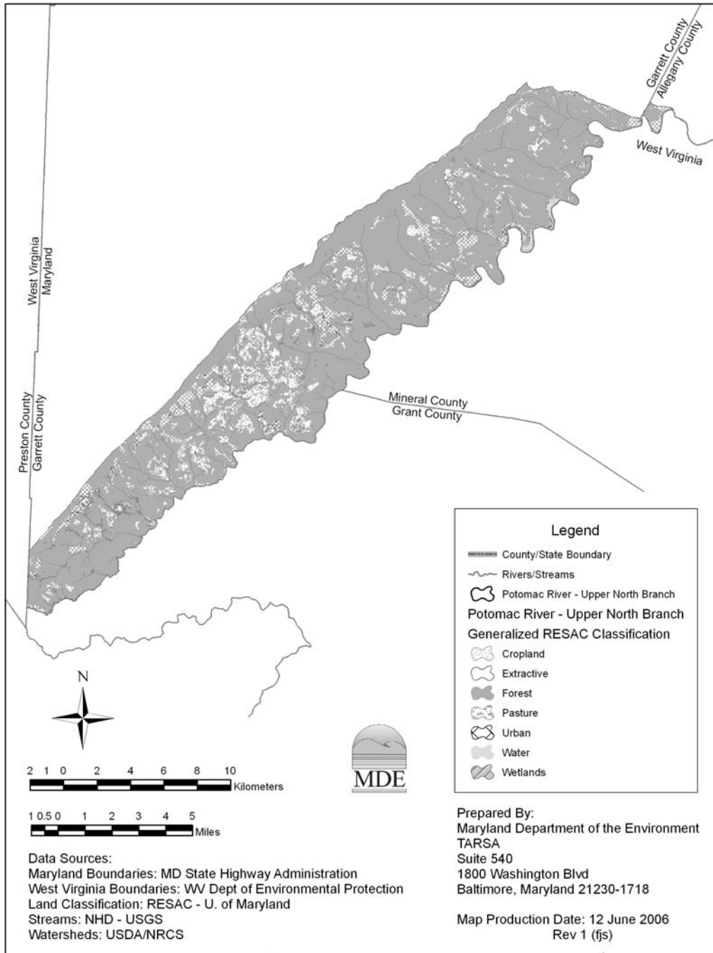
Figure 2: Land Use of the Upper North Branch Potomac River Watershed
