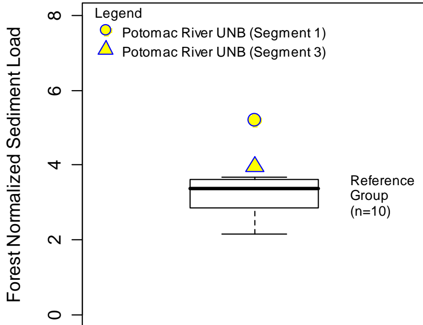
Figure 6: The Upper North Branch Potomac River Forest Normalized Sediment Load Compared to Reference Watershed Group
