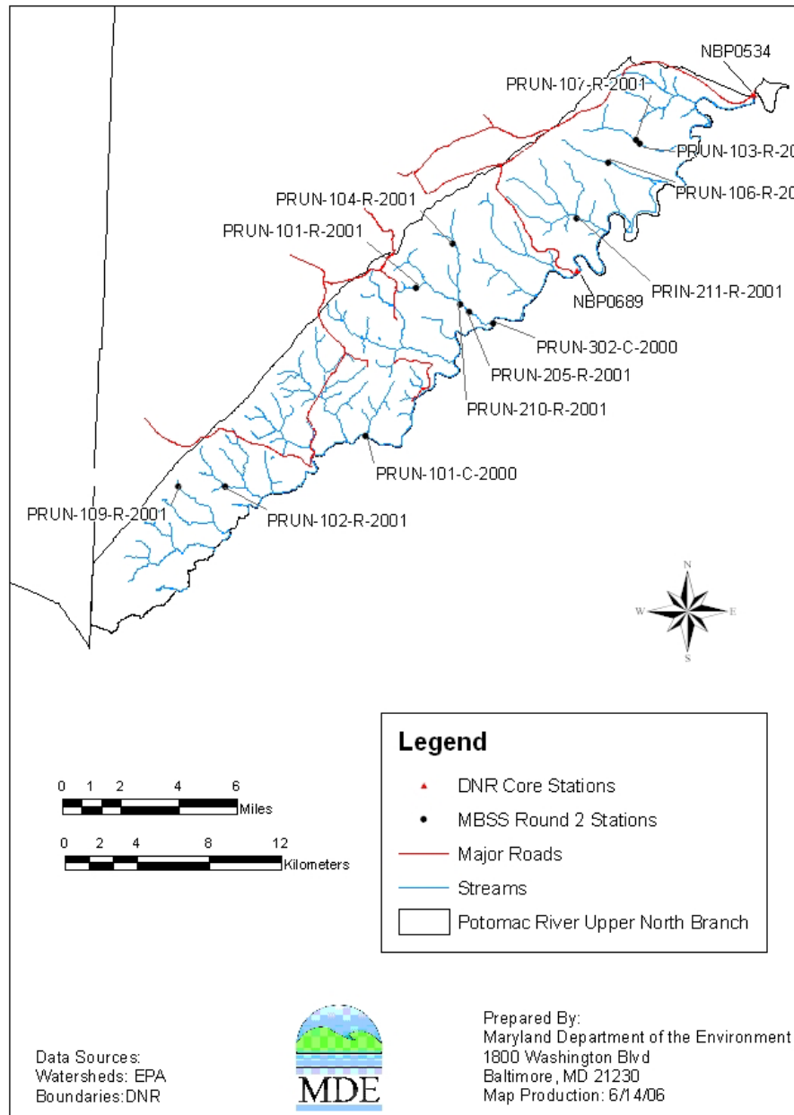
Figure 3: MBSS and DNR Core Stations in the Upper North Branch Potomac River Watershed
