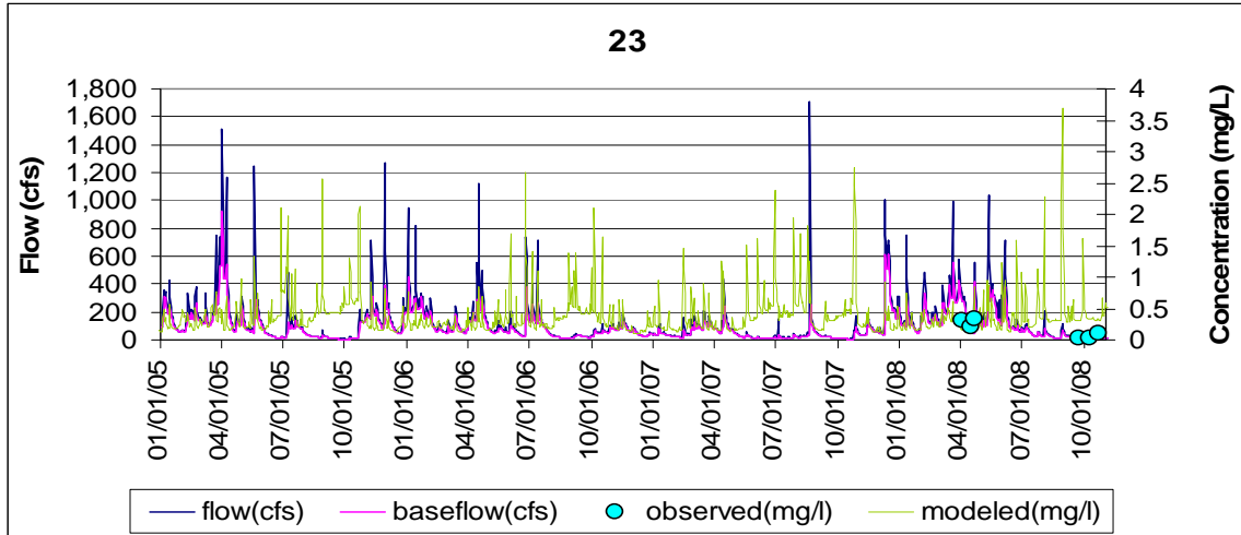
Figure D-1. Calibration at station Potomac 1
