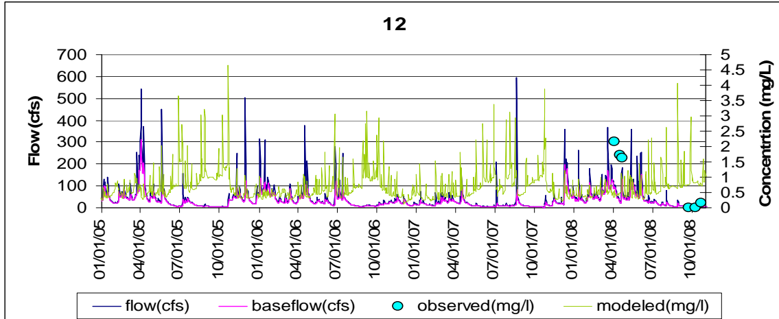
Figure D-13. Validation at station Site 9
