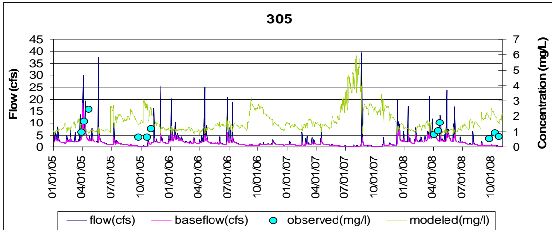
Figure D-14. Validation at station ULF0003
