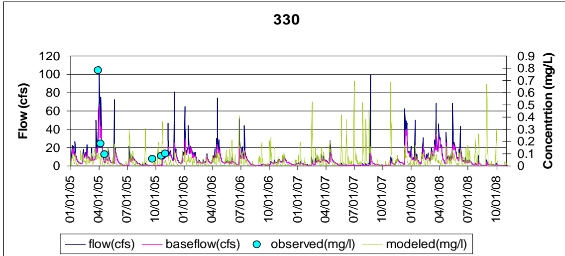
Figure D-16. Validation at station NPL0001
