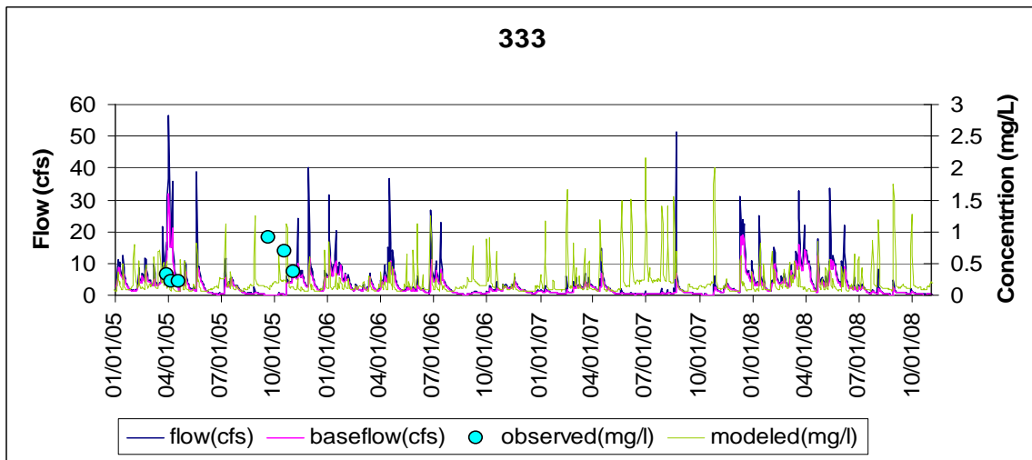
Figure D-20. Validation at station SPL0016
