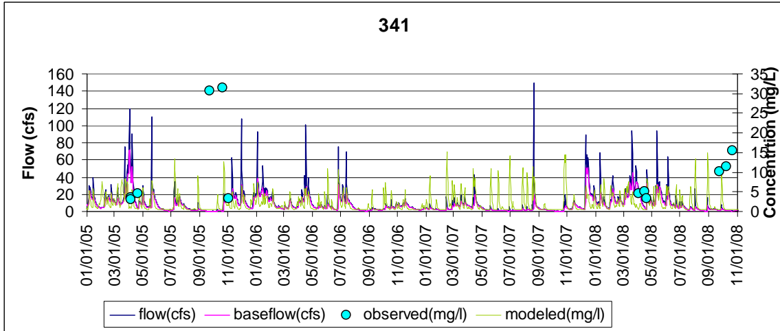
Figure D-4. Calibration at station TFR0016
