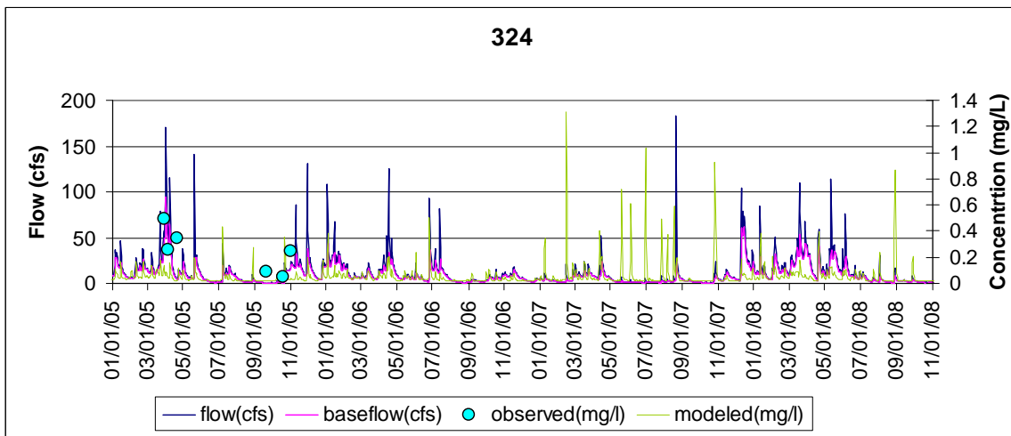
Figure D-8. Calibration at station LUR0017
