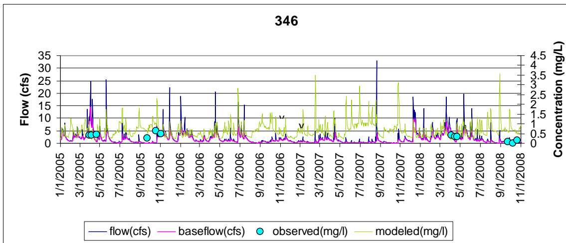
Figure D-5. Calibration at station EKL0003
