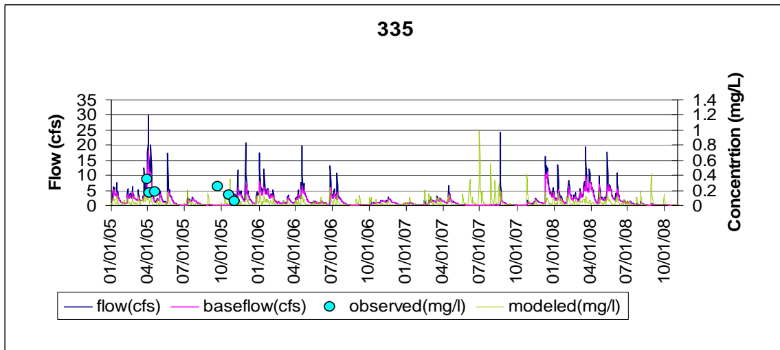
Figure D-17. Validation at station SHO0016
