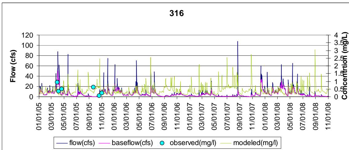
Figure D-3. Calibration at station NYD0004
