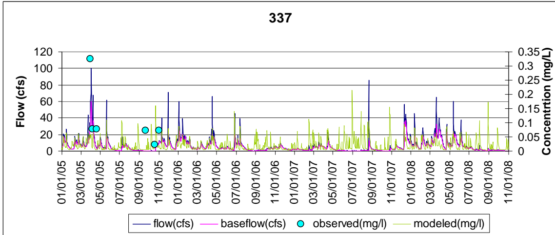
Figure D-10. Calibration at station WOL0004
