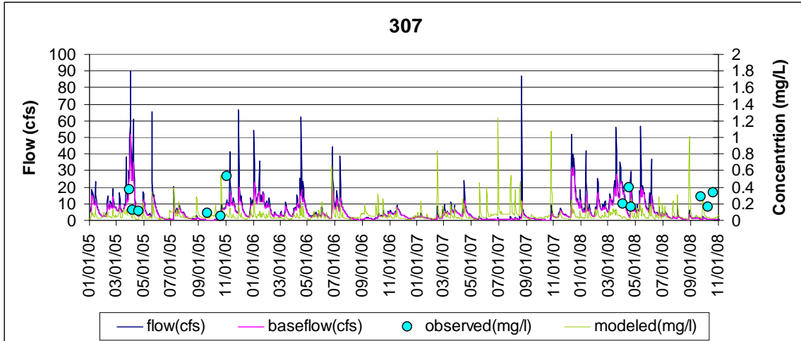
Figure D-7. Calibration at station SAD0004
