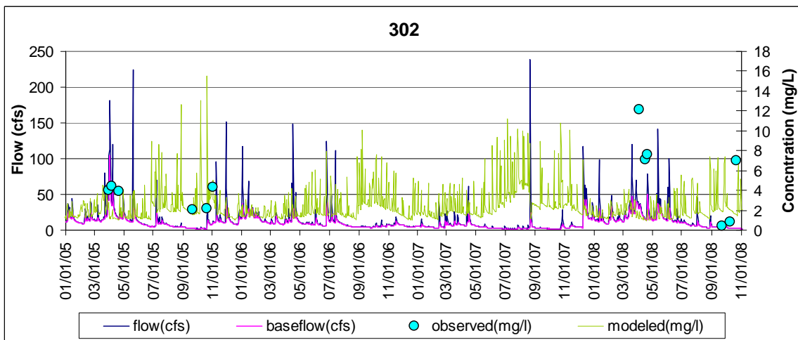
Figure D-6. Calibration at station LNB0014
