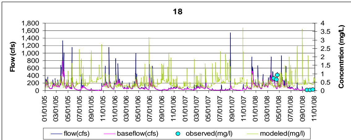
Figure D-2. Calibration at station Site 17
