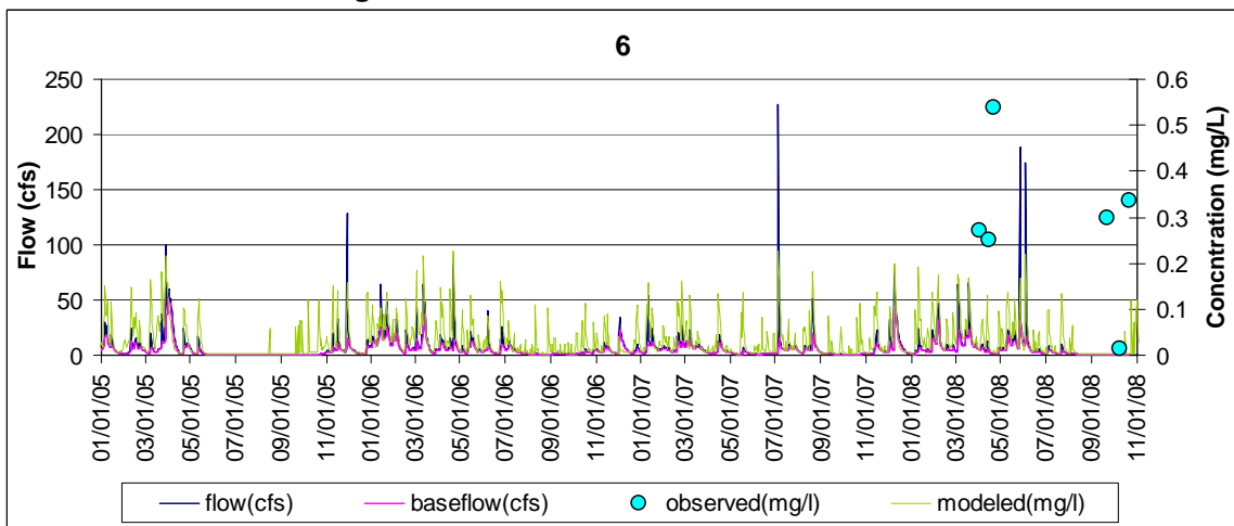
Figure D-11. Calibration at station TFR0021
