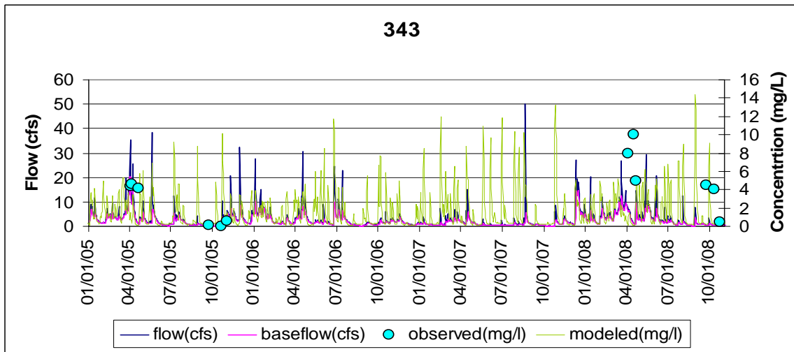
Figure D-21. Validation at station RTF0005
