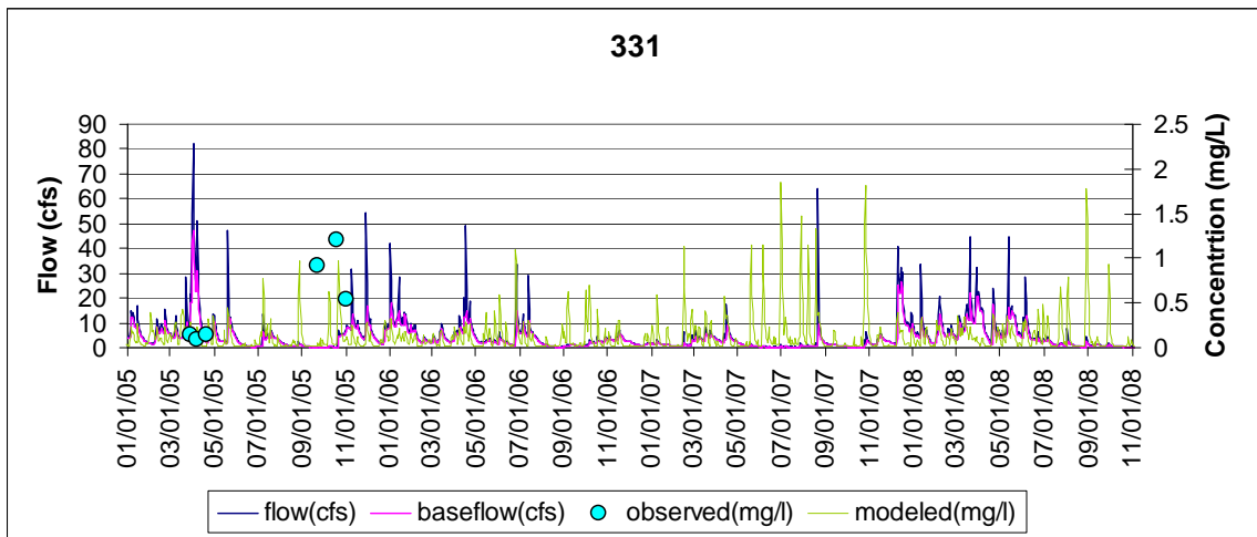
Figure D-9. Calibration at station NPL0018
