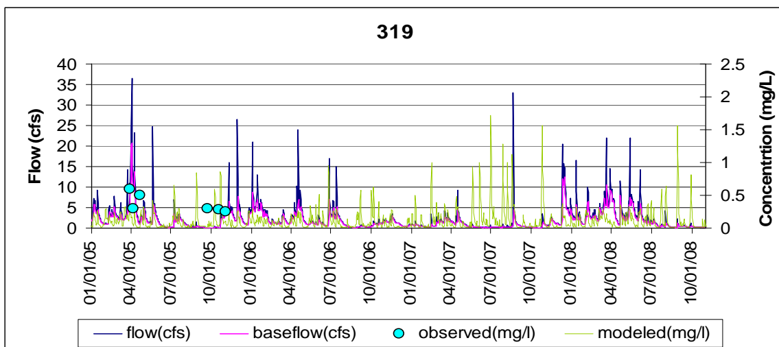
Figure D-15. Validation at station GLR0031
