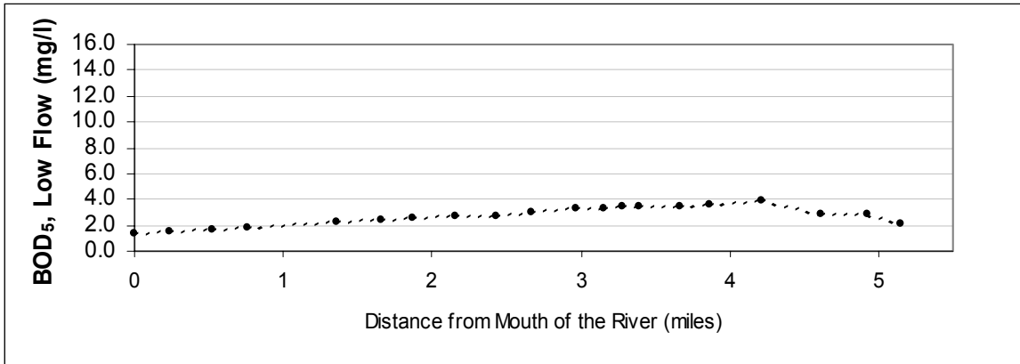
Figure A26: BOD vs. River Mile for the Baseline Conditions Low Flow Scenario
