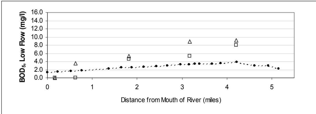
Figure A10: BOD 5 vs. River Mile for the Calibration of the Model (Low flow)
