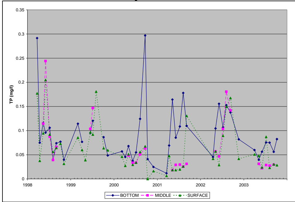
Figure A.13. Observed Total Phosphorus Concentrations at TR3, 1998-2003, Triadelphia Reservoir
