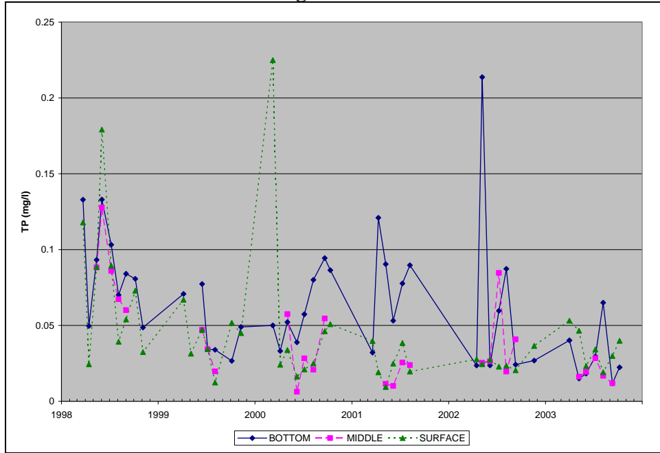
Figure A.15. Observed Total Phosphorus Concentrations at RG2, 1998-2003, Rocky Gorge Reservoir
