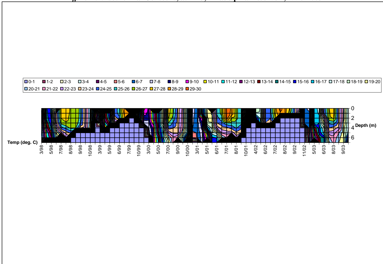
Figure A.2. Isothermal Contours, at TR3, Triadelphia Reservoir, 1998-2003
