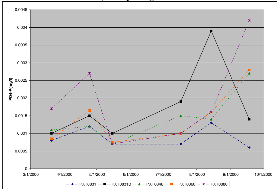
Figure A.26. Observed Phosphate-P Concentrations at MDE Sampling Stations, 2000, Rocky Gorge Reservoir
