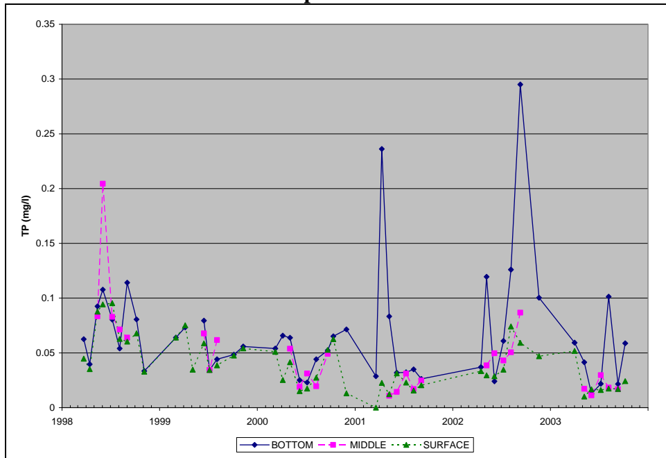
Figure A.11. Observed Total Phosphorus Concentrations at TR1, 1998-2003, Triadelphia Reservoir
