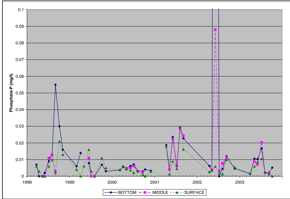
Figure A.19. Observed Phosphate-P Concentrations at TR1, 1998-2003, Triadelphia Reservoir
