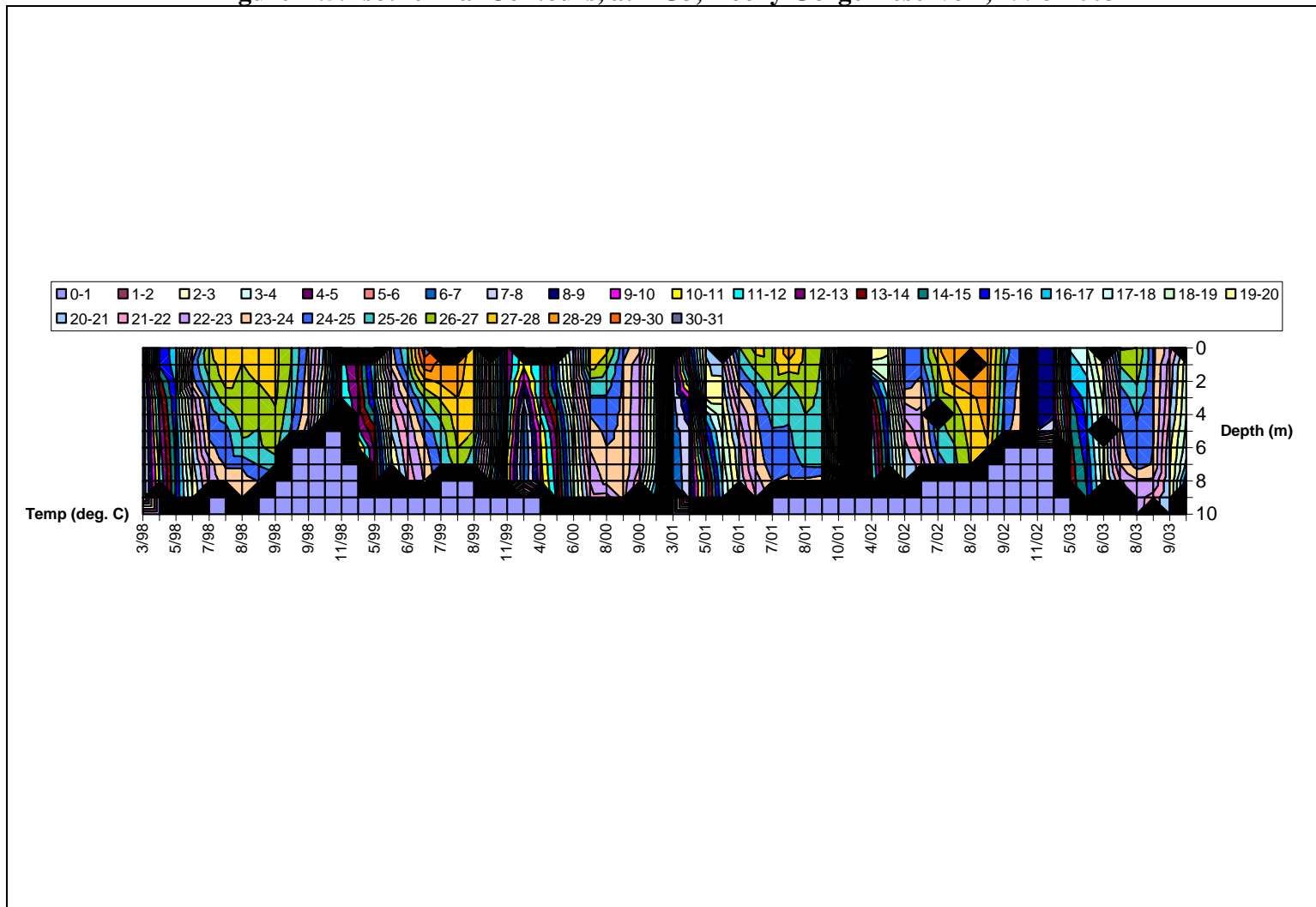
Figure A.5. Isothermal Contours, at RG3, Rocky Gorge Reservoir, 1998-2003
