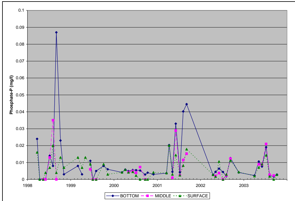
Figure A.20. Observed Phosphate-P Concentrations at TR2, 1998-2003, Triadelphia Reservoir
