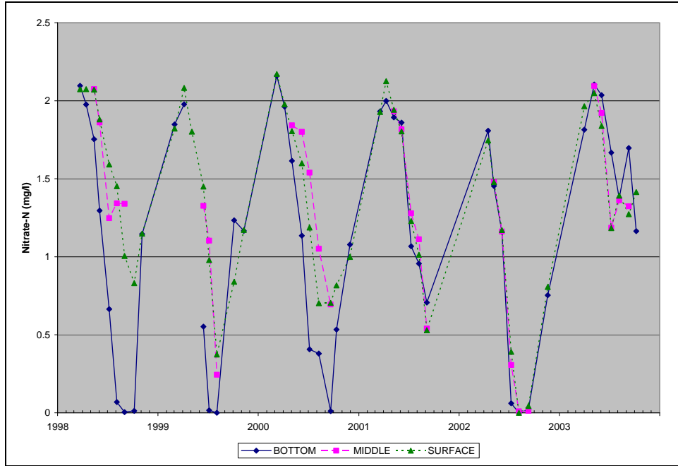
Figure A.35. Observed Nitrate-N Concentrations at TR1, 1998-2003, Triadelphia Reservoir
