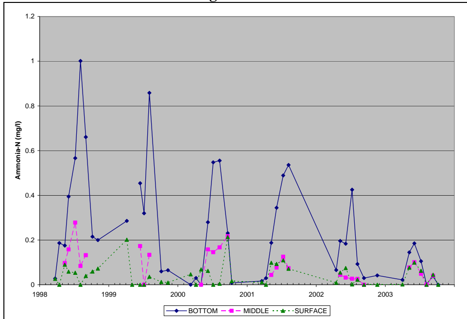
Figure A.30. Observed Ammonia-N Concentrations at RG1, 1998-2003, Rocky Gorge Reservoir
