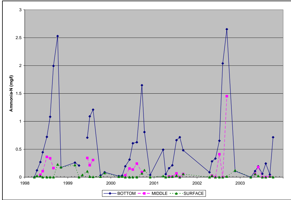
Figure A.27. Observed Ammonia-N Concentrations at TR1, 1998-2003, Triadelphia Reservoir
