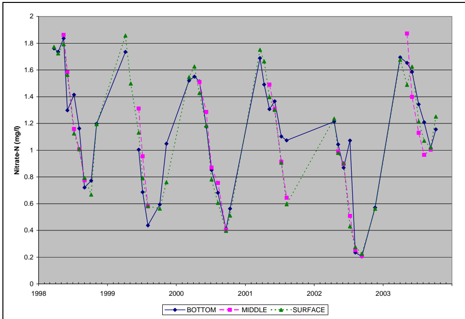
Figure A.40. Observed Nitrate-N Concentrations at RG3, 1998-2003, Rocky Gorge Reservoir
