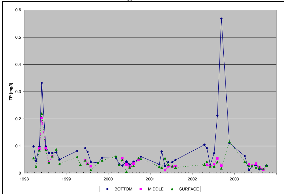
Figure A.16. Observed Total Phosphorus Concentrations at RG3, 1998-2003, Rocky Gorge Reservoir
