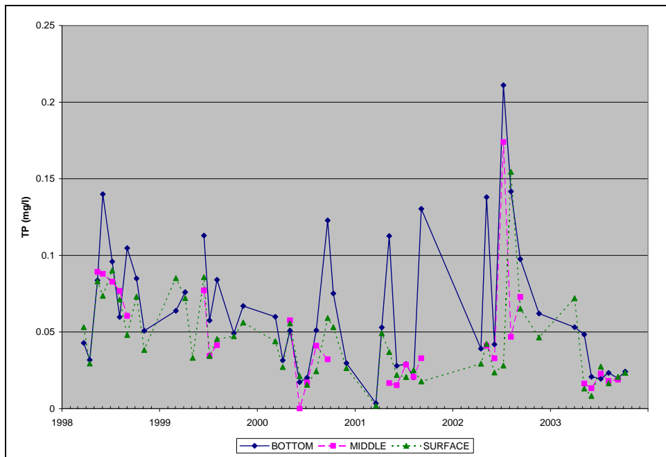
Figure A.12. Observed Total Phosphorus Concentrations at TR2, 1998-2003, Triadelphia Reservoir
