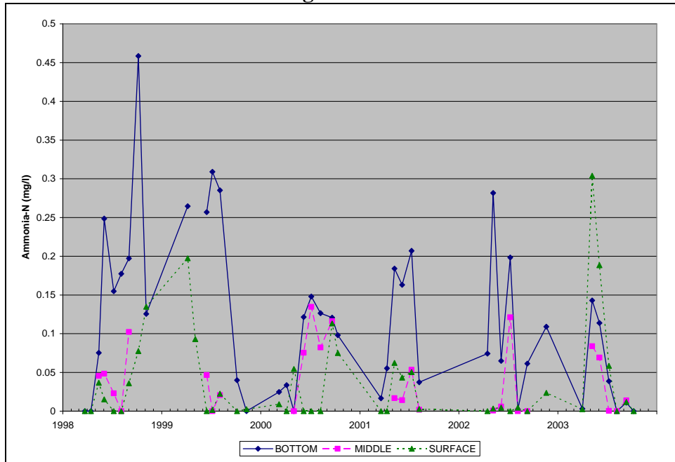
Figure A.32. Observed Ammonia-N Concentrations at RG3, 1998-2003, Rocky Gorge Reservoir
