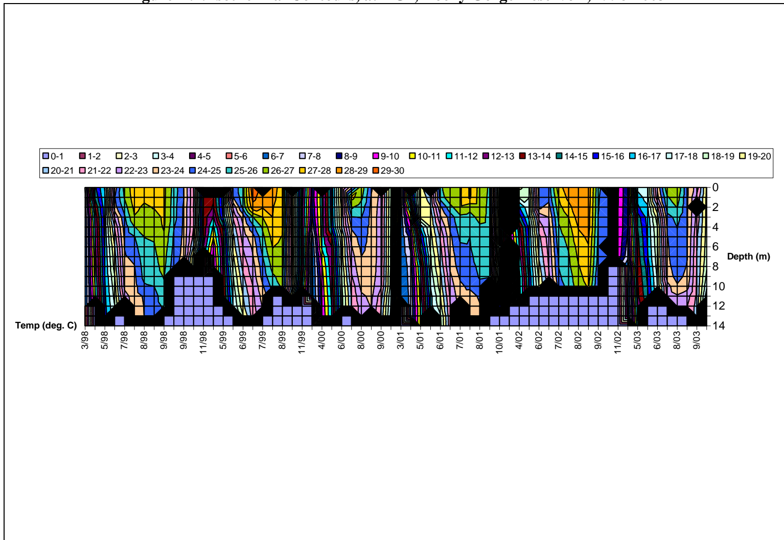
Figure A.4. Isothermal Contours, at RG2, Rocky Gorge Reservoir, 1998-2003
