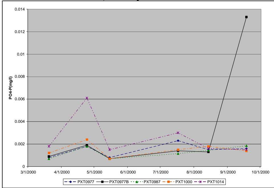
Figure A.25. Observed Phosphate-P Concentrations at MDE Sampling Stations, 2000, Triadelphia Reservoir
