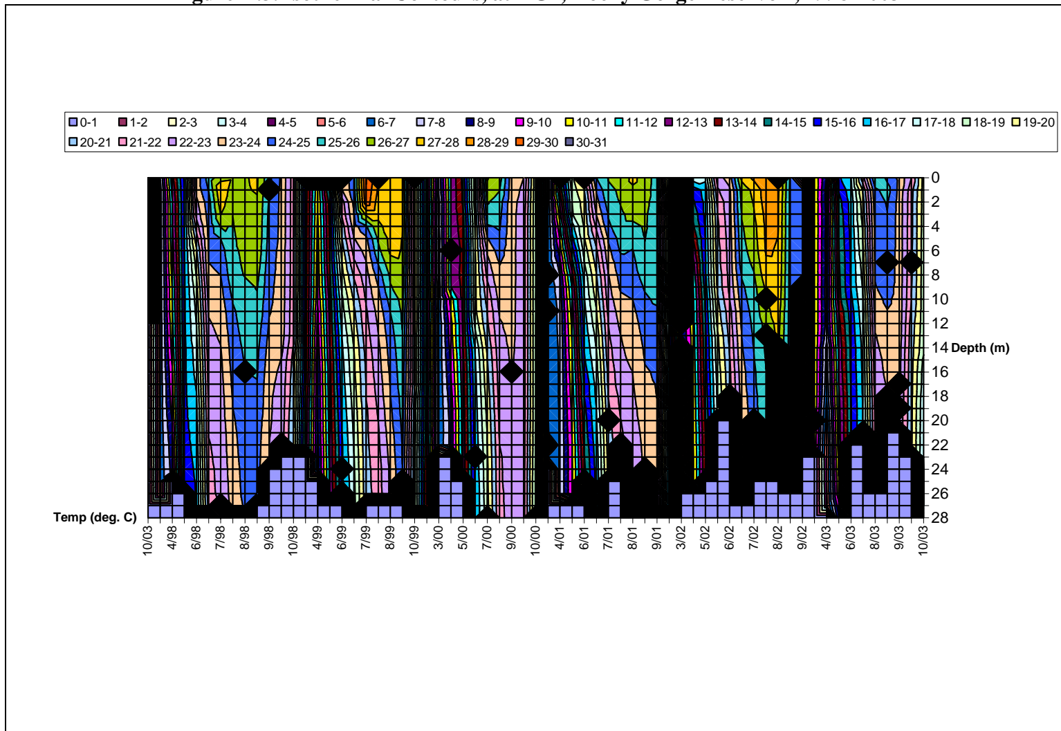
Figure A.3. Isothermal Contours, at RG1, Rocky Gorge Reservoir, 1998-2003
