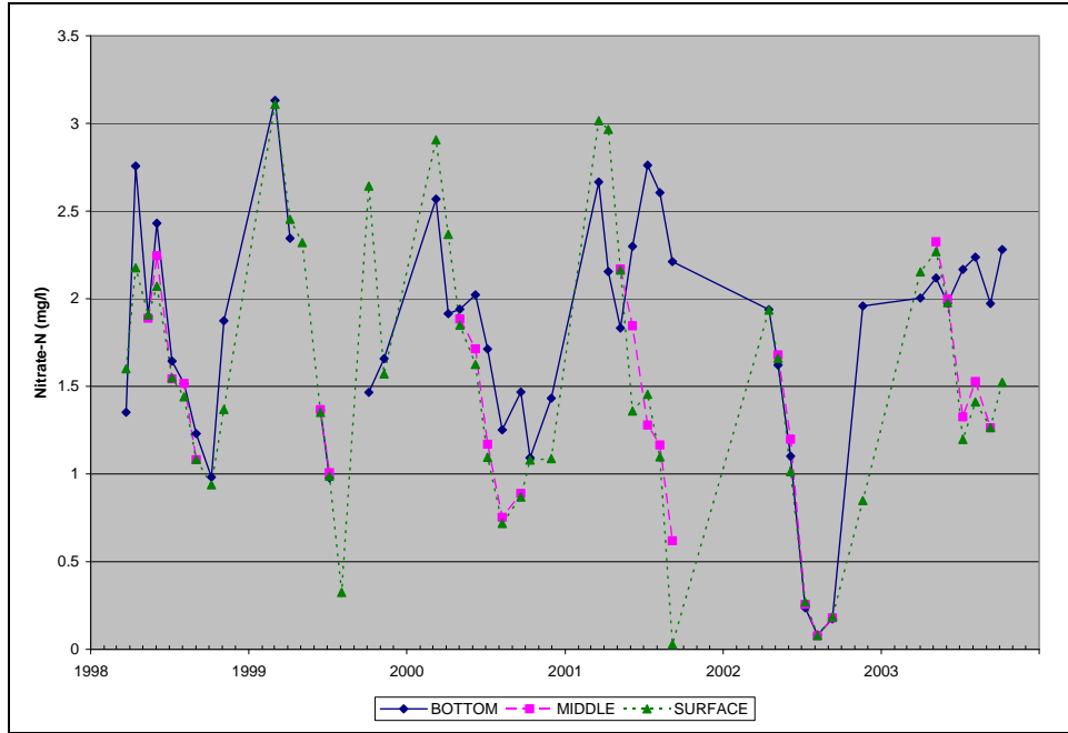
Figure A.37. Observed Nitrate-N Concentrations at TR3, 1998-2003, Triadelphia Reservoir
