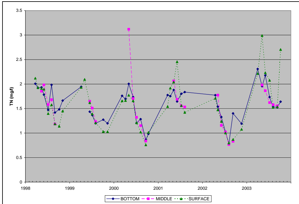
Figure A.46. Observed TN Concentrations at RG1, 1998-2003, Rocky Gorge Reservoir
