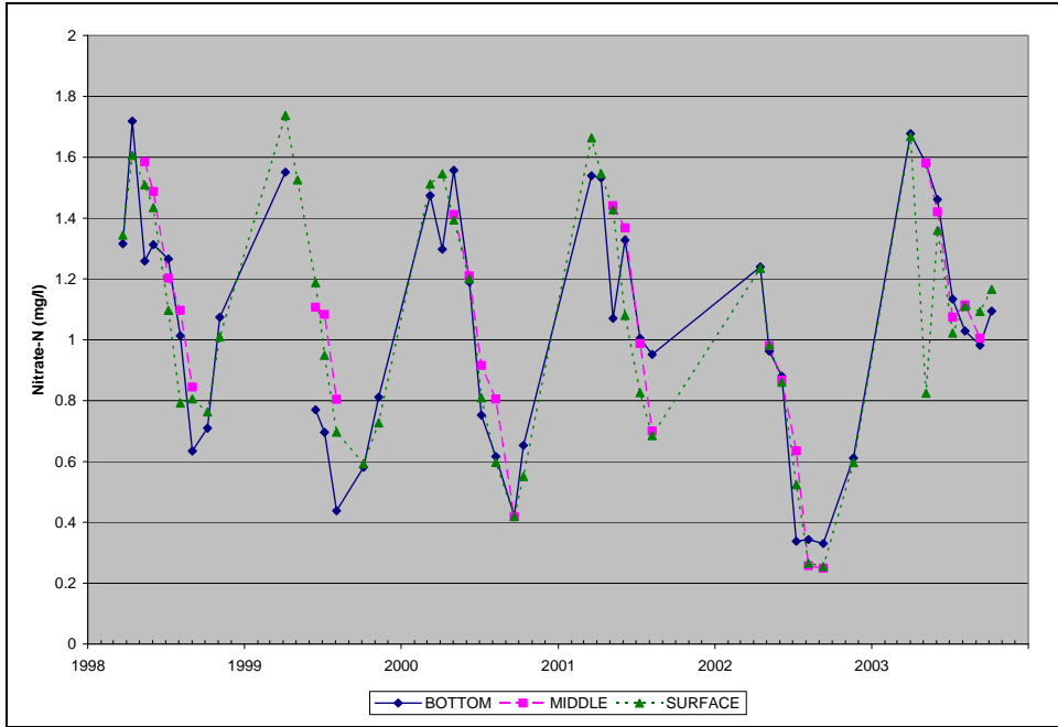
Figure A.39. Observed Nitrate-N Concentrations at RG2, 1998-2003, Rocky Gorge Reservoir
