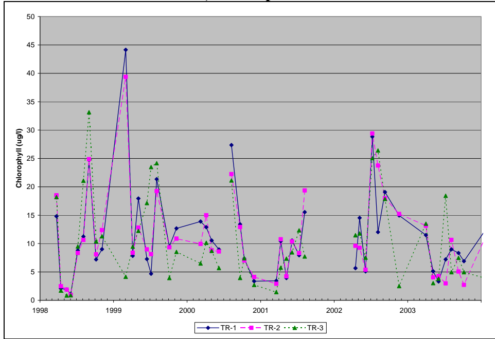
Figure A.51. Observed Chlorophyll a Concentrations at WSSC Sampling Stations, 1998-2003, Triadelphia Reservoir
