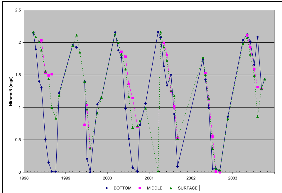
Figure A.36. Observed Nitrate-N Concentrations at TR2, 1998-2003, Triadelphia Reservoir
