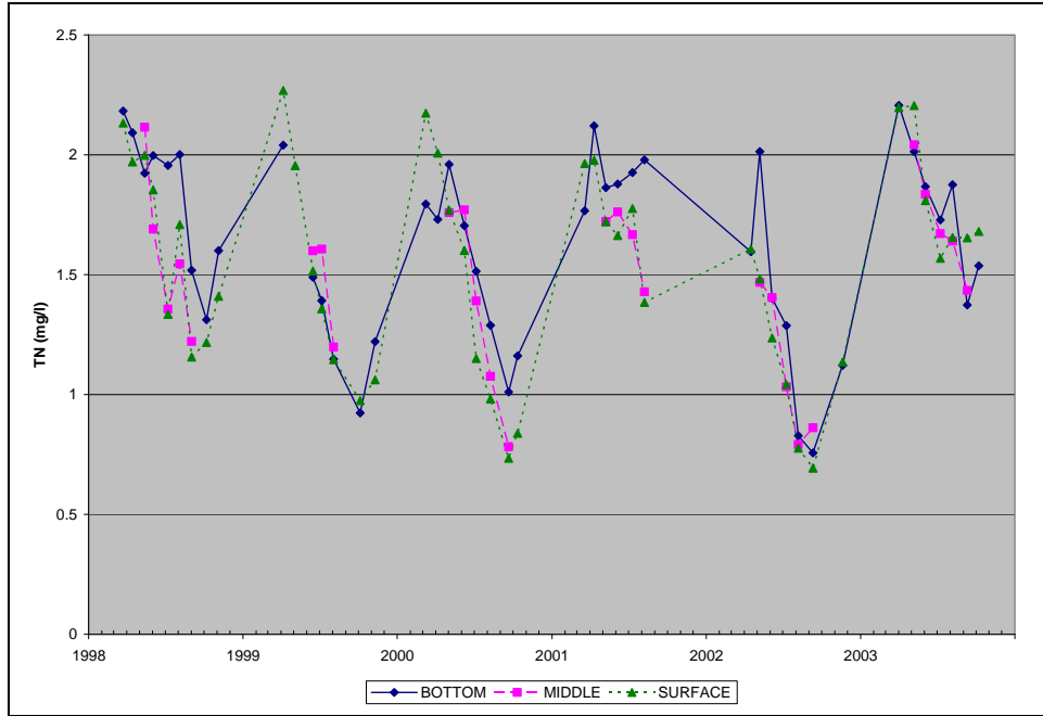
Figure A.47. Observed TN Concentrations at RG2, 1998-2003, Rocky Gorge Reservoir
