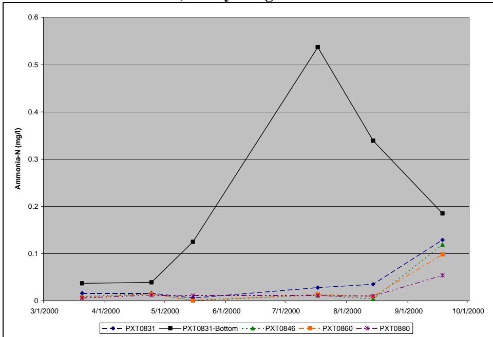
Figure A.34. Observed Ammonia-N Concentrations at MDE Sampling Stations, 2000, Rocky Gorge Reservoir
