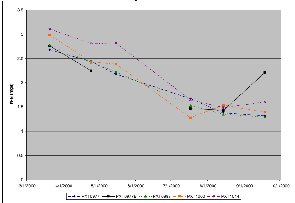
Figure A.49. Observed TN Concentrations at MDE Sampling Stations, 2000, Triadelphia Reservoir
