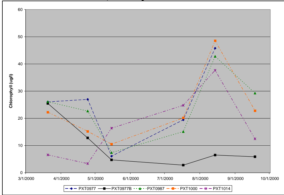
Figure A.53. Observed Chlorophyll a Concentrations at MDE Sampling Stations, 2000, Triadelphia Reservoir
