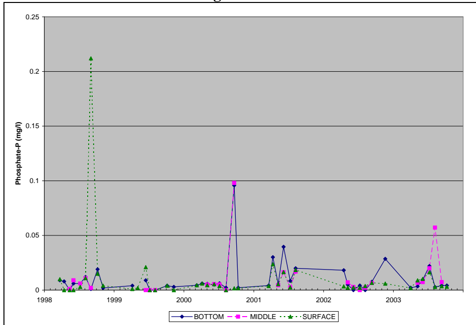
Figure A.24. Observed Phosphate-P Concentrations at RG3, 1998-2003, Rocky Gorge Reservoir
