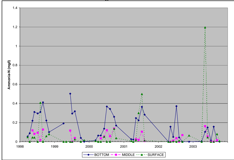
Figure A.31. Observed Ammonia-N Concentrations at RG2, 1998-2003, Rocky Gorge Reservoir
