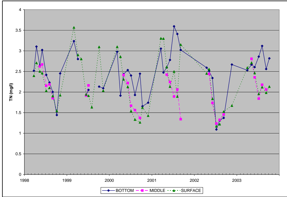
Figure A.45. Observed TN Concentrations at TR3, 1998-2003, Triadelphia Reservoir
