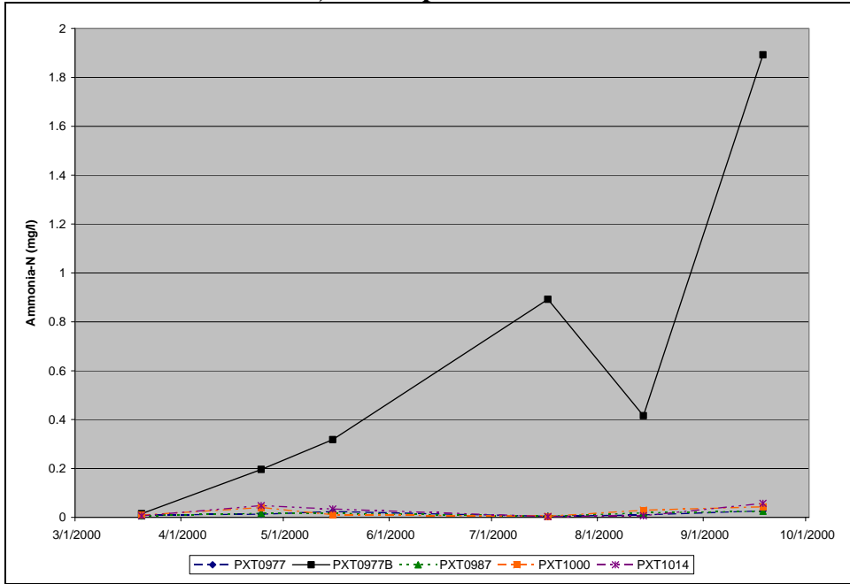
Figure A.33. Observed Ammonia-N Concentrations at MDE Sampling Stations, 2000, Triadelphia Reservoir
