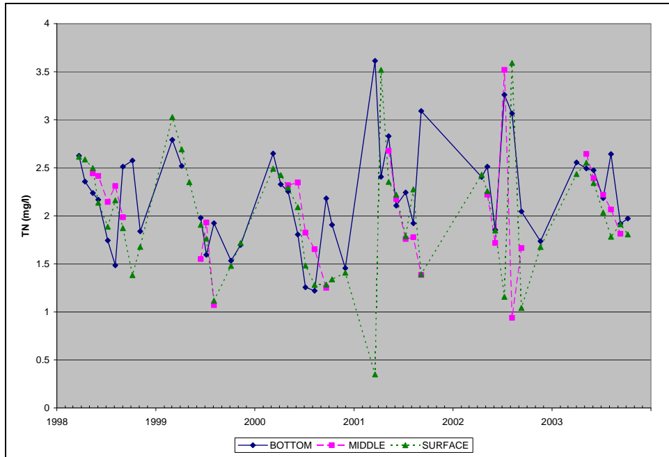
Figure A.44. Observed TN Concentrations at TR2, 1998-2003, Triadelphia Reservoir
