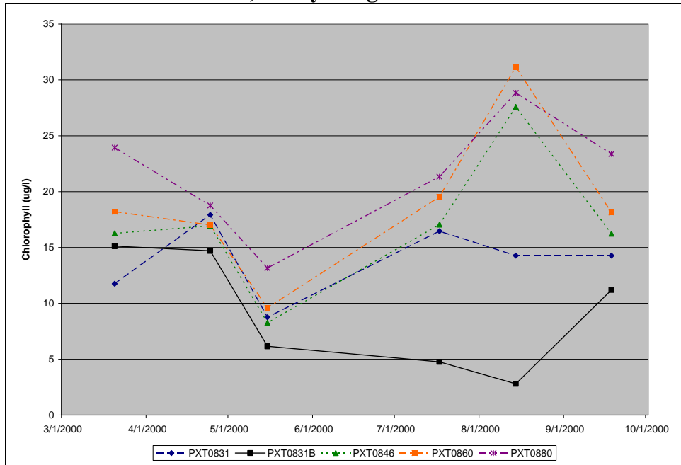
Figure A.54. Observed Chlorophyll a Concentrations at MDE Sampling Stations, 2000, Rocky Gorge Reservoir
