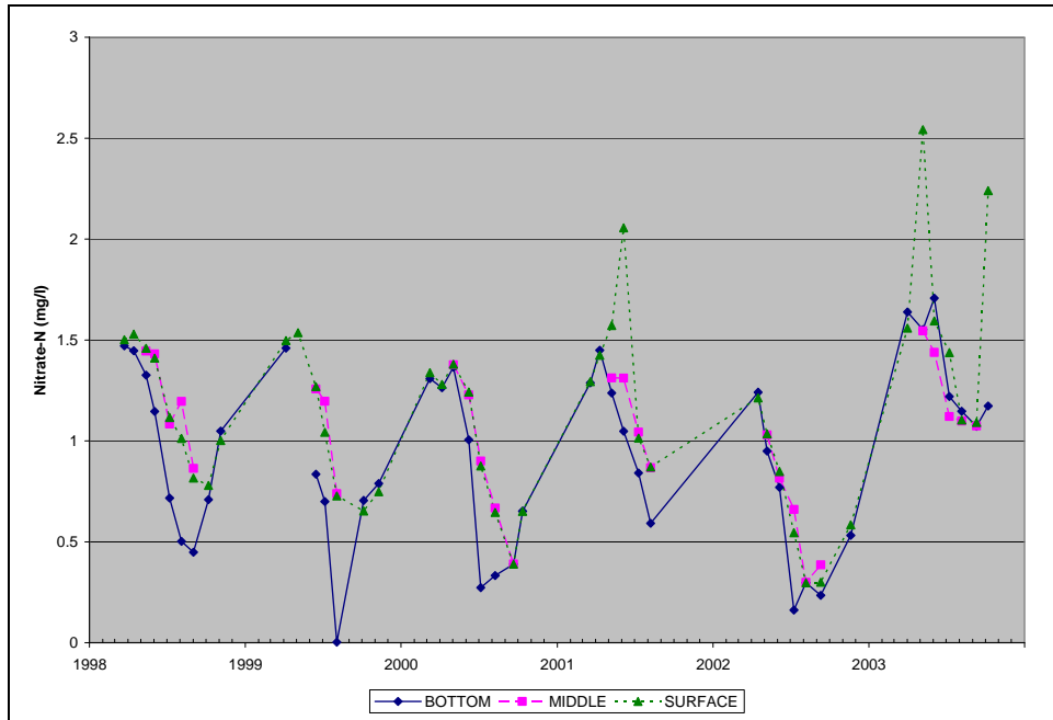
Figure A.38. Observed Nitrate-N Concentrations at RG1, 1998-2003, Rocky Gorge Reservoir
