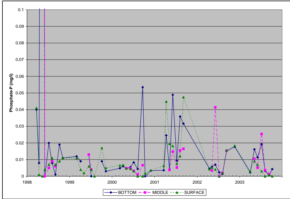
Figure A.21. Observed Phosphate-P Concentrations at TR3, 1998-2003, Triadelphia Reservoir
