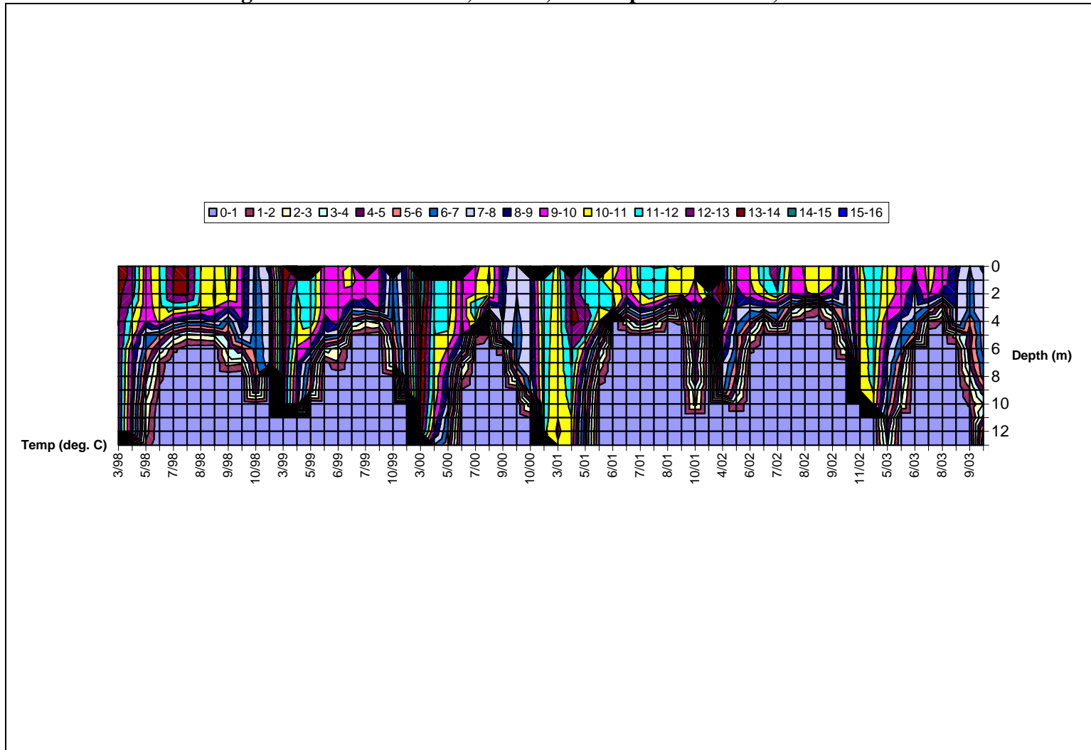
Figure A.6. DO Contours, at TR2, Triadelphia Reservoir, 1998-2003
