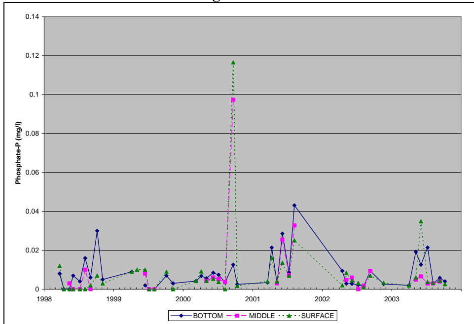
Figure A.22. Observed Phosphate-P Concentrations at RG1, 1998-2003, Rocky Gorge Reservoir
