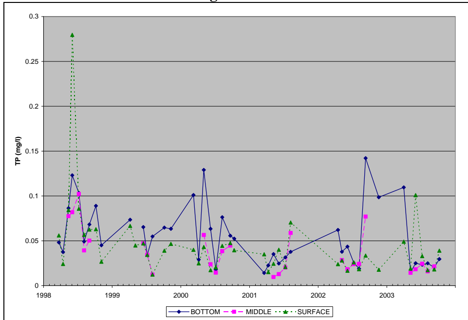
Figure A.14. Observed Total Phosphorus Concentrations at RG1, 1998-2003, Rocky Gorge Reservoir
