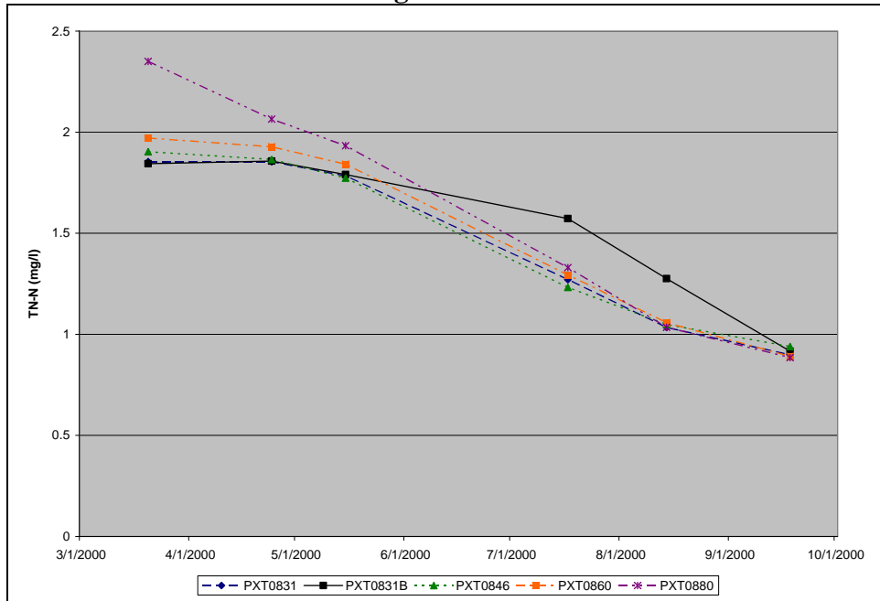
Figure A.50. Observed TN Concentrations at MDE Sampling Stations, 2000, Rocky Gorge Reservoir
