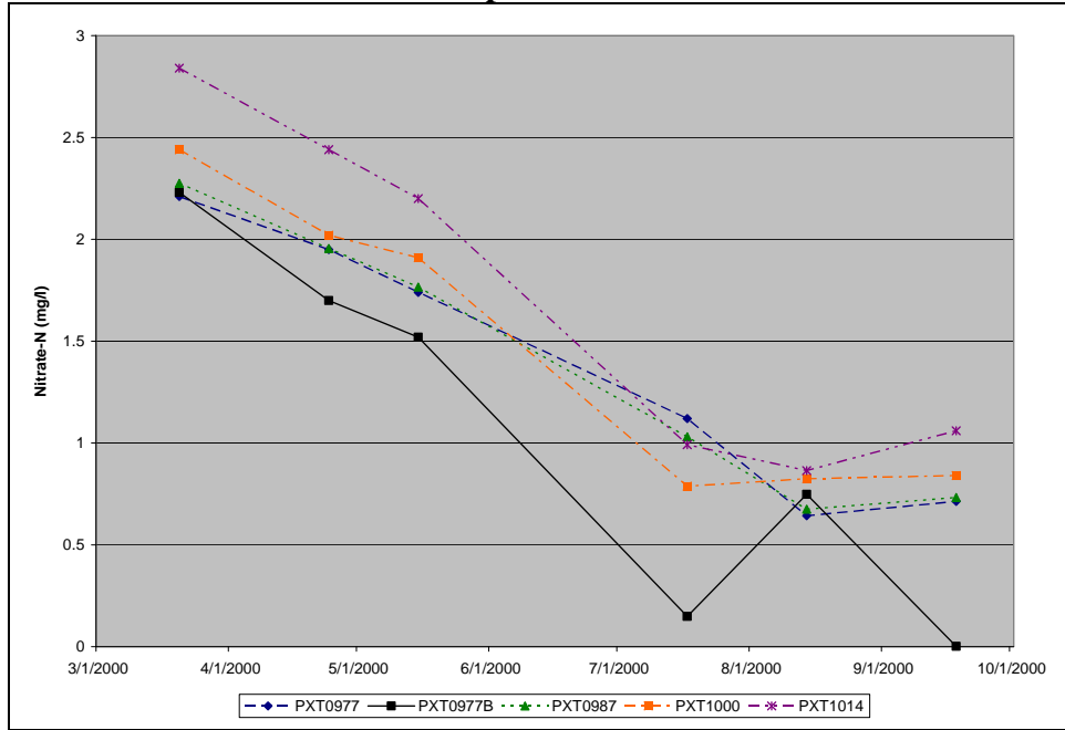
Figure A.41. Observed Nitrate-N Concentrations at MDE Sampling Stations, 2000, Triadelphia Reservoir
