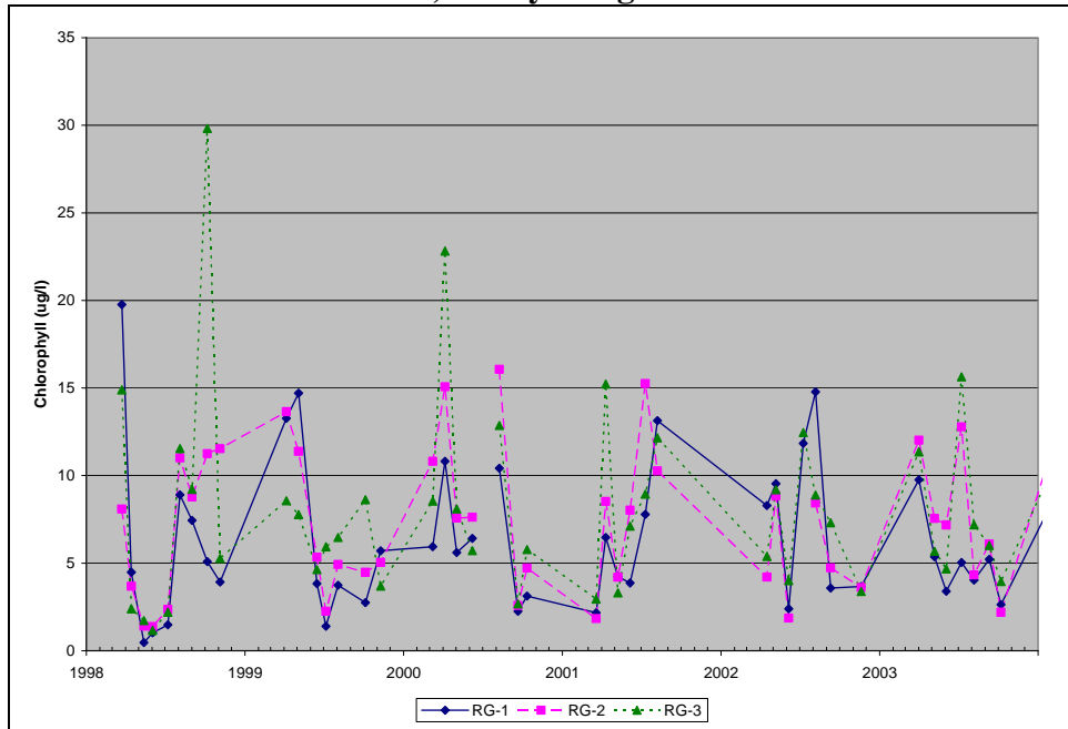
Figure A.52. Observed Chlorophyll a Concentrations at WSSC Sampling Stations, 1998-2003, Rocky Gorge Reservoir
