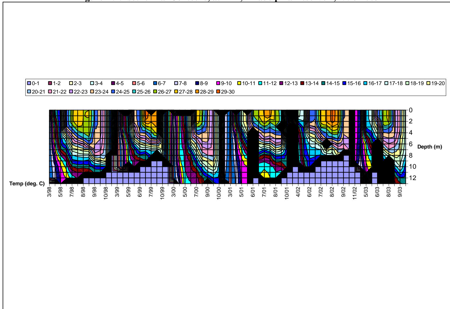
Figure A.1. Isothermal Contours, at TR2, Triadelphia Reservoir, 1998-2003
