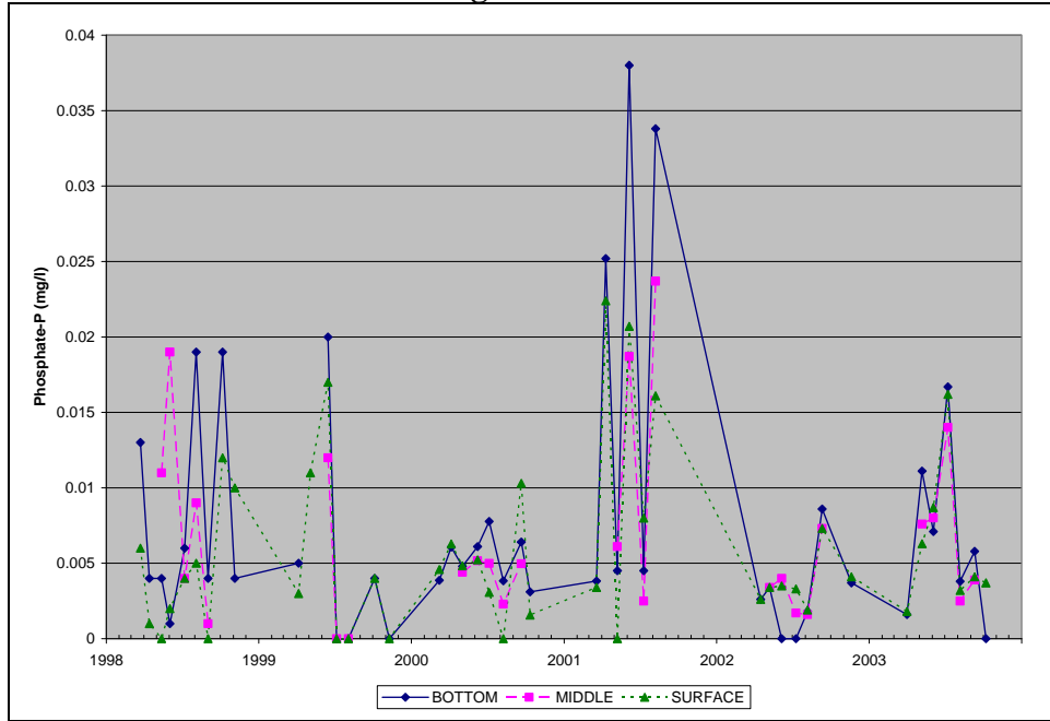
Figure A.23. Observed Phosphate-P Concentrations at RG2, 1998-2003, Rocky Gorge Reservoir
