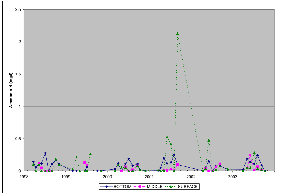
Figure A.29. Observed Ammonia-N Concentrations at TR3, 1998-2003, Triadelphia Reservoir
