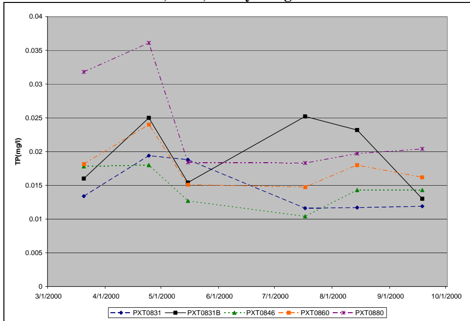
Figure A.18. Observed Total Phosphorus Concentrations at MDE Sampling Stations, 2000, Rocky Gorge Reservoir
