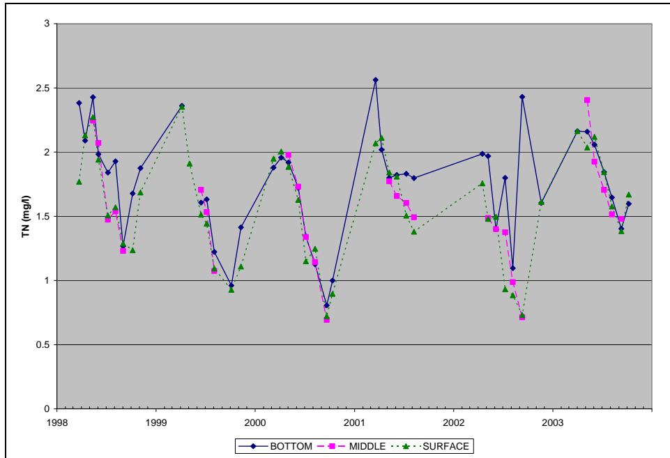
Figure A.48. Observed TN Concentrations at RG3, 1998-2003, Rocky Gorge Reservoir
