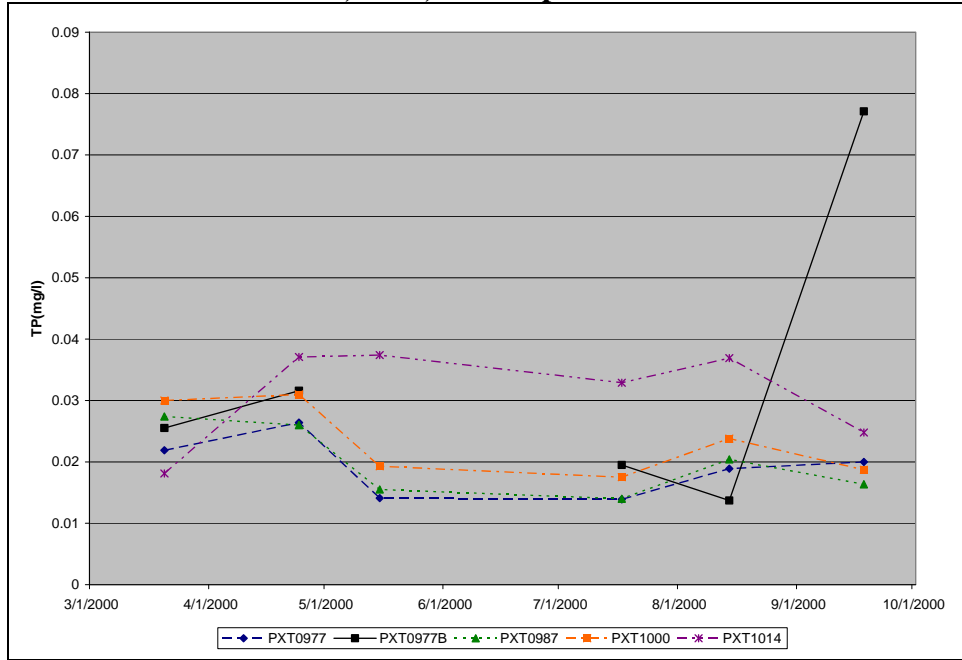
Figure A.17. Observed Total Phosphorus Concentrations at MDE Sampling Stations, 2000, Triadelphia Reservoir
