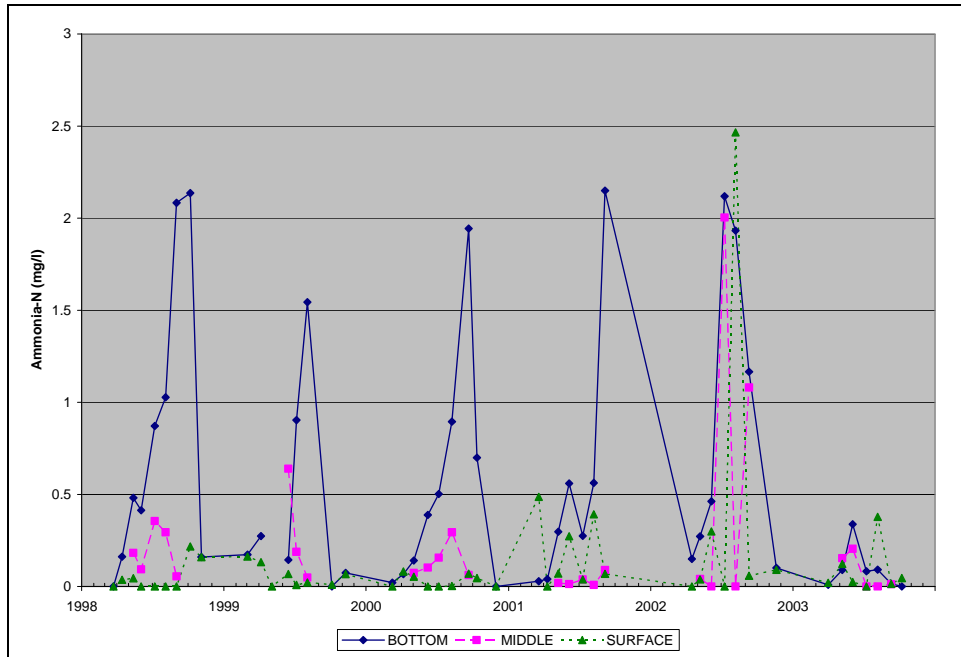
Figure A.28. Observed Ammonia-N Concentrations at TR2, 1998-2003, Triadelphia Reservoir
