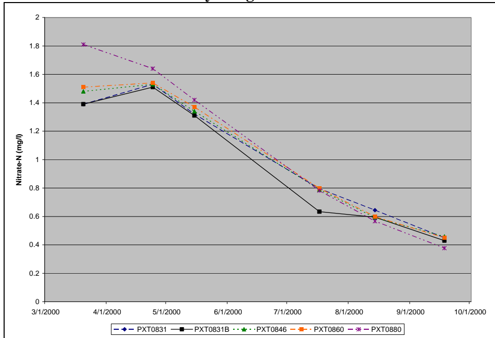
Figure A.42. Observed Nitrate-N Concentrations at MDE Sampling Stations, 2000, Rocky Gorge Reservoir
