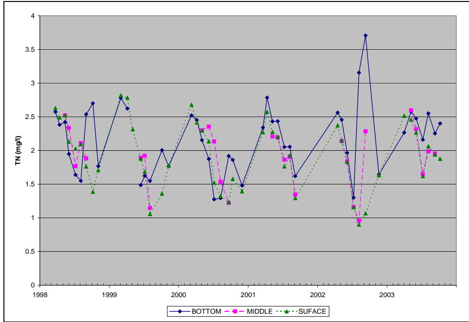
Figure A.43. Observed TN Concentrations at TR1, 1998-2003, Triadelphia Reservoir
