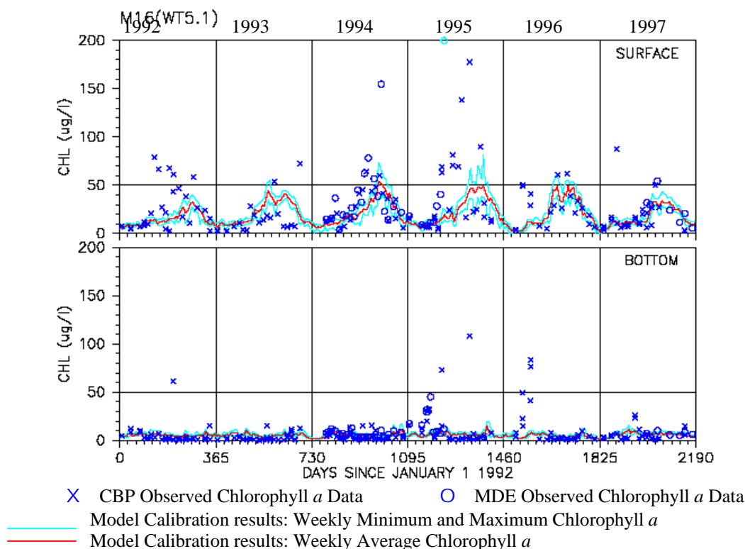
Figure 9: Time Series of Model Calibration Results of Chl a in Harbor Station WT5.1
