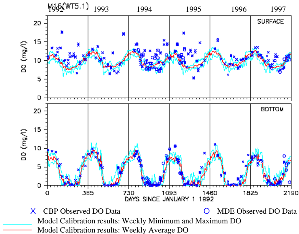
Figure 8: Time Series of Model Calibration Results of DO in Harbor Station WT5.1
