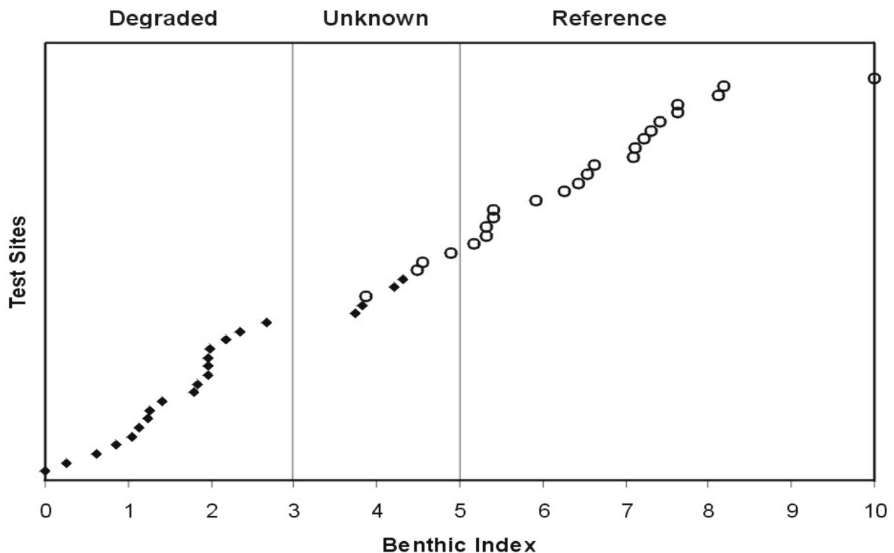
Figure 3-9. Distribution of benthic index values for the test sites where \blacklozenge = degraded sites and \circ = undegraded sites determined by a priori criteria for dissolved oxygen, sediment chemistry, and sediment toxicity. The cutoff value for degraded sites determined by the benthic index is 3.0 and 5.0 is the cutoff value for undegraded sites determined by the benthic index.
