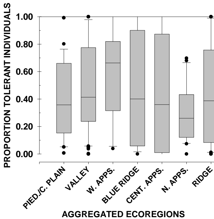
Figure 4-7. Examples of evaluating possible differences in metric expectations across MAHA subdivided by two levels of ecoregion aggregation. (A) number of water column species, a metric based on species richness; (B) proportion of individuals of tolerant species, a metric based on the proportion of individuals collected.
