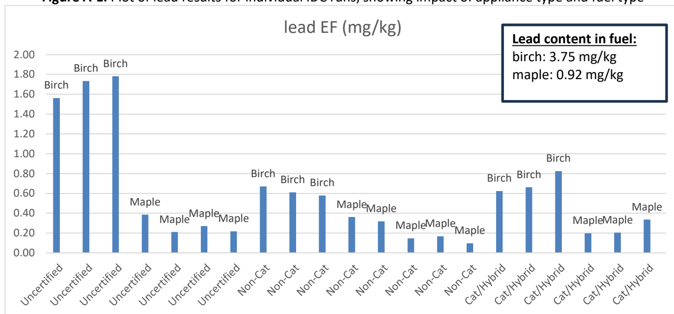
Figure A-1. Plot of lead results for individual IDC runs, showing impact of appliance type and fuel type
