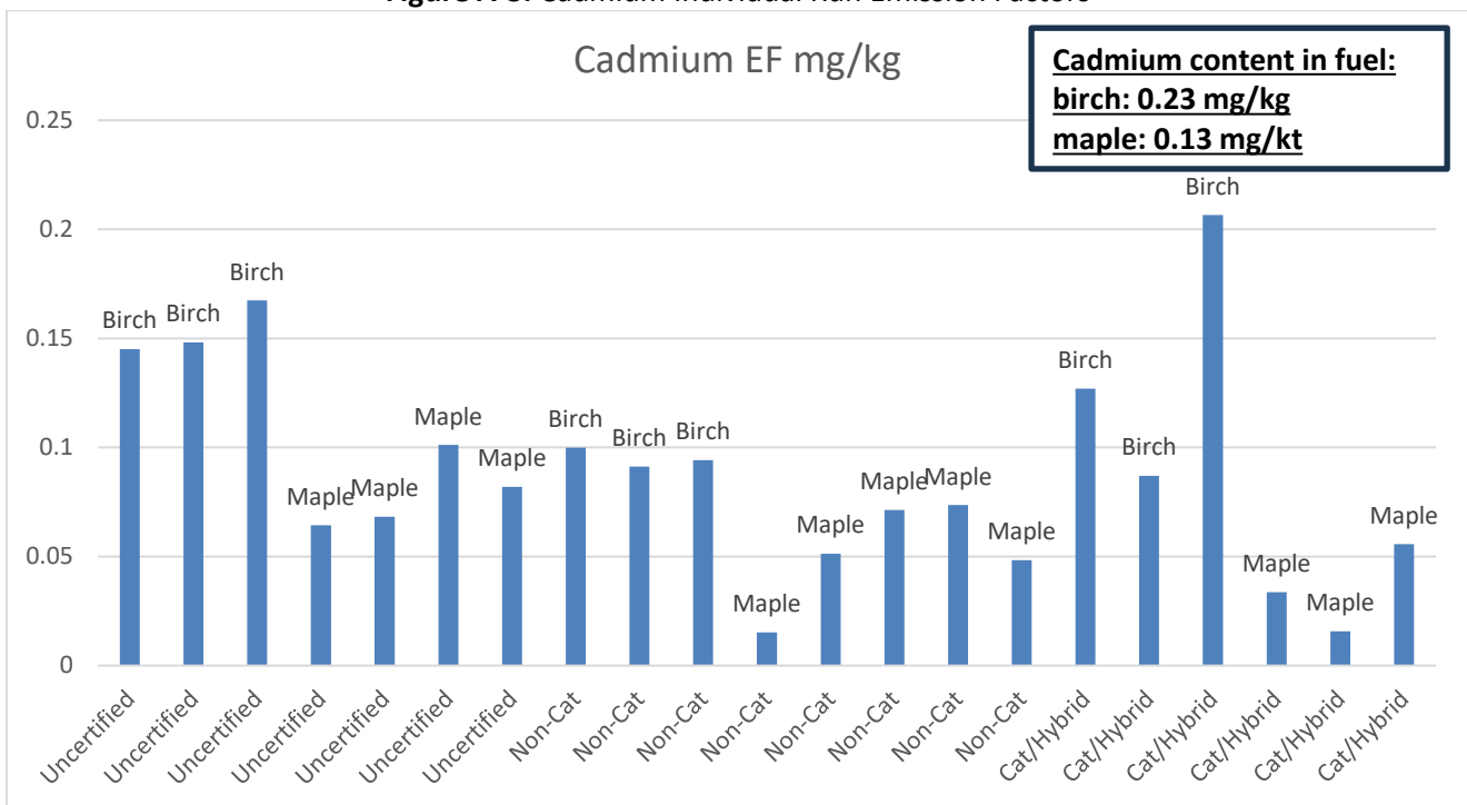
Figure A-3. Cadmium Individual Run Emission Factors
