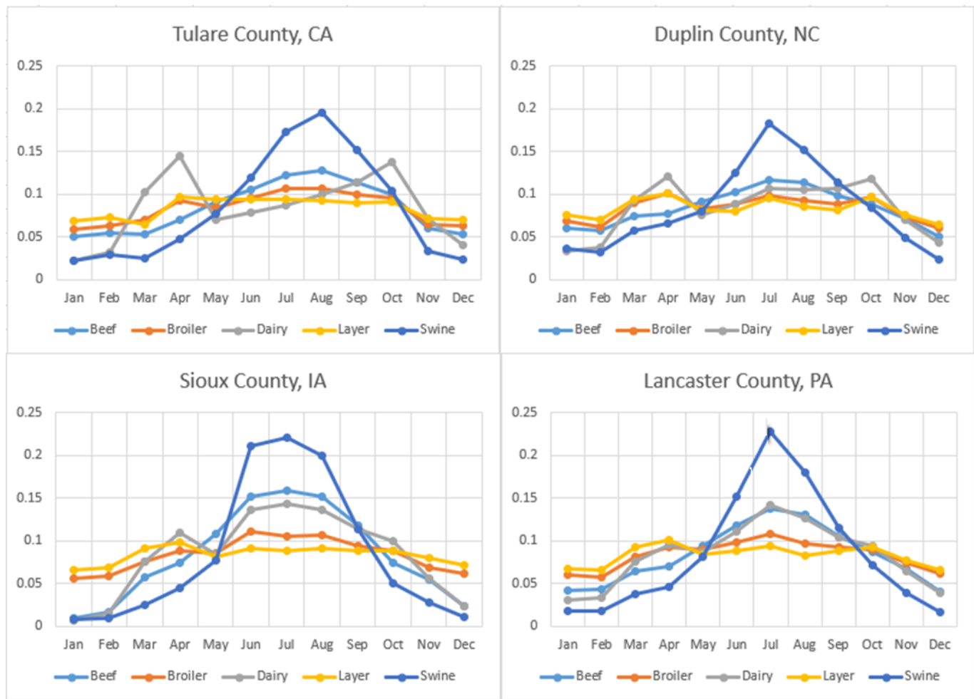
Figure 3-16. Example of animal NH 3 emissions temporal allocation approach (daily total emissions)
