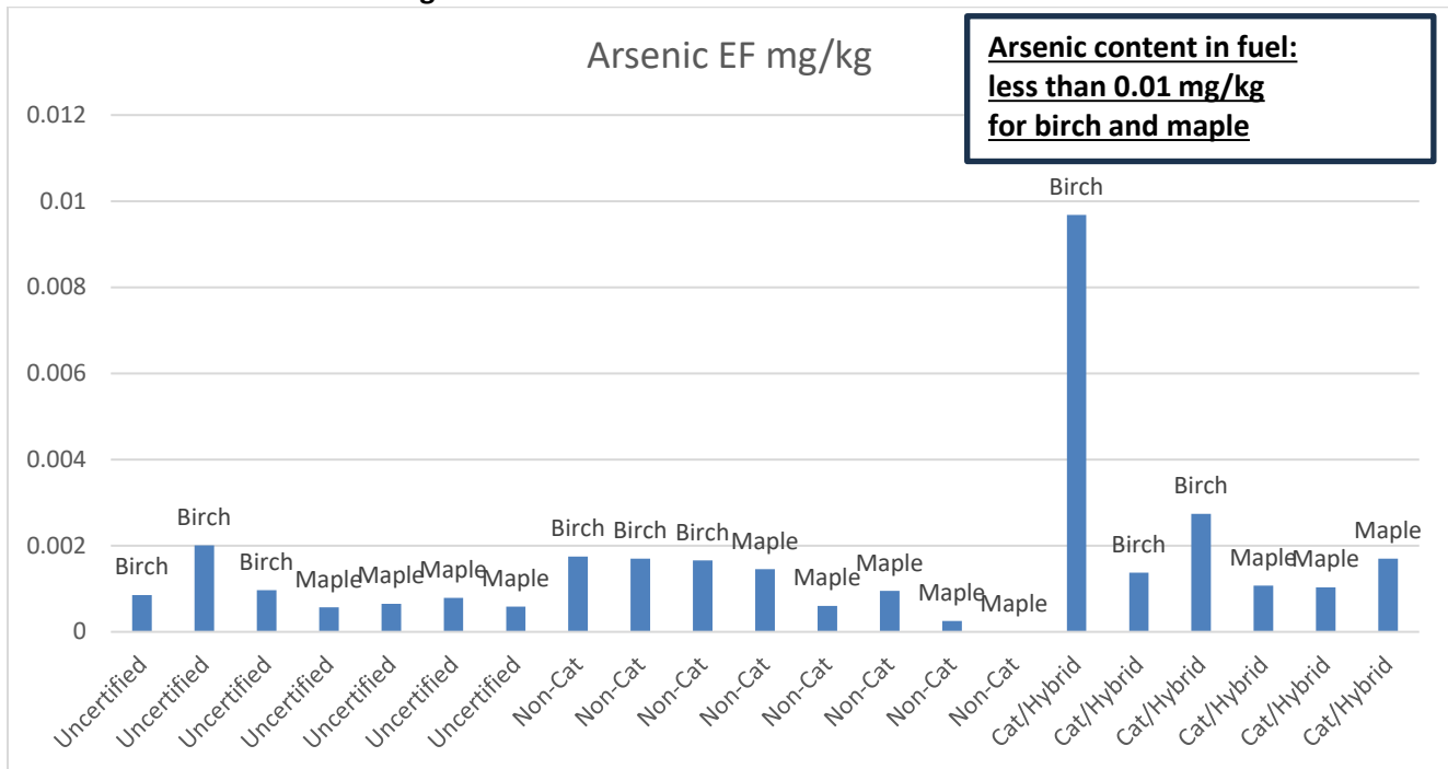
Figure A-5. Arsenic Individual Run Emission Factors
