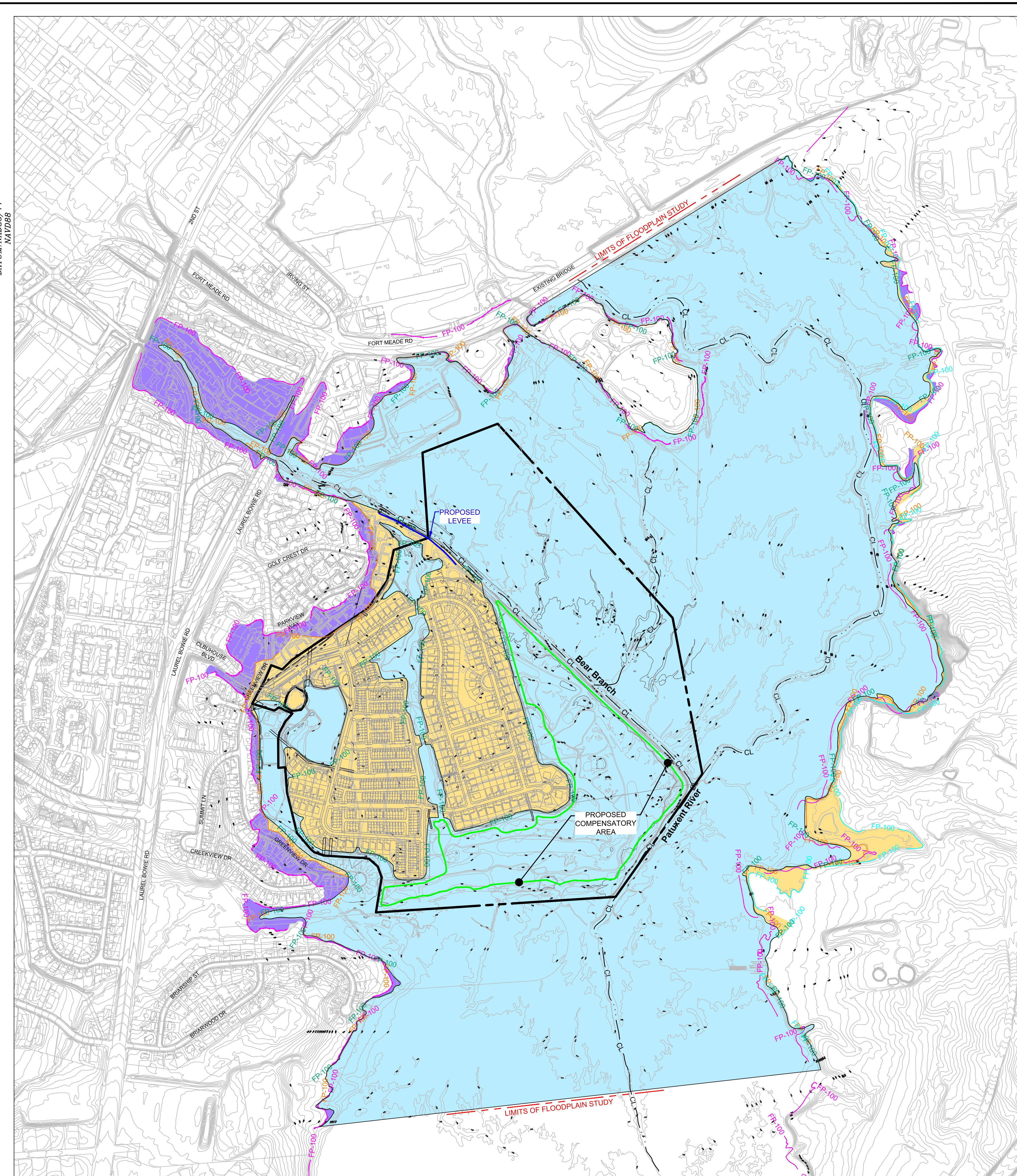
PROPOSED 100 YEAR FLOOD AREA OVER EXISTING 100 YEAR FLOOD AREA TO SHOW PROPOSED REDUCTION
