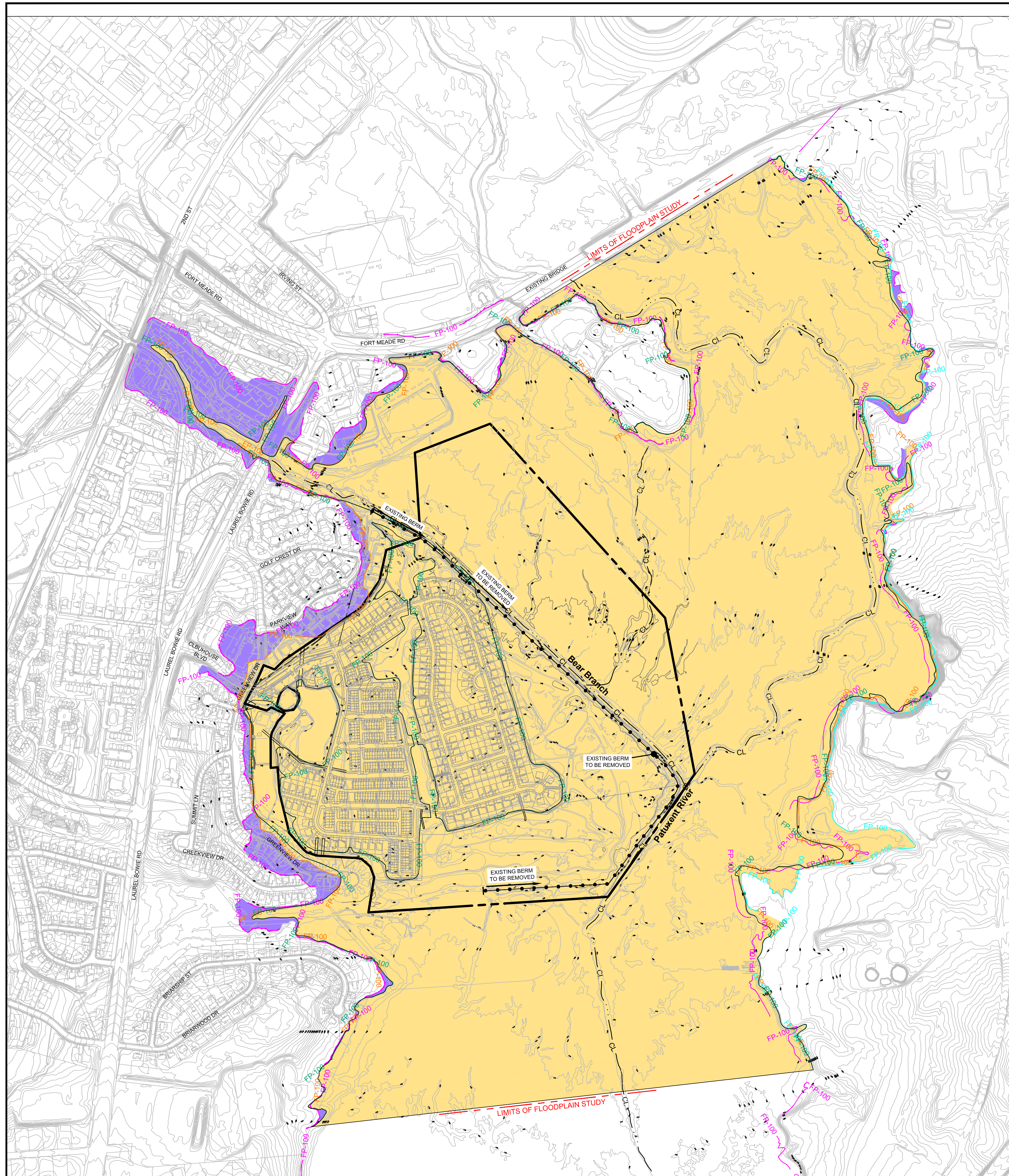
EXISTING 100 YEAR FLOOD AREA
