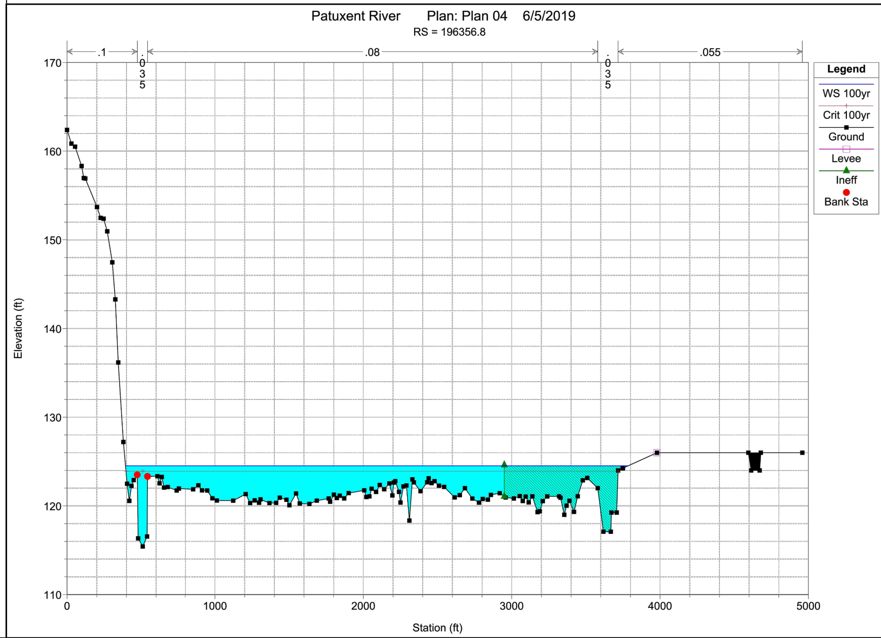
CROSS-SECTION 196356.8
