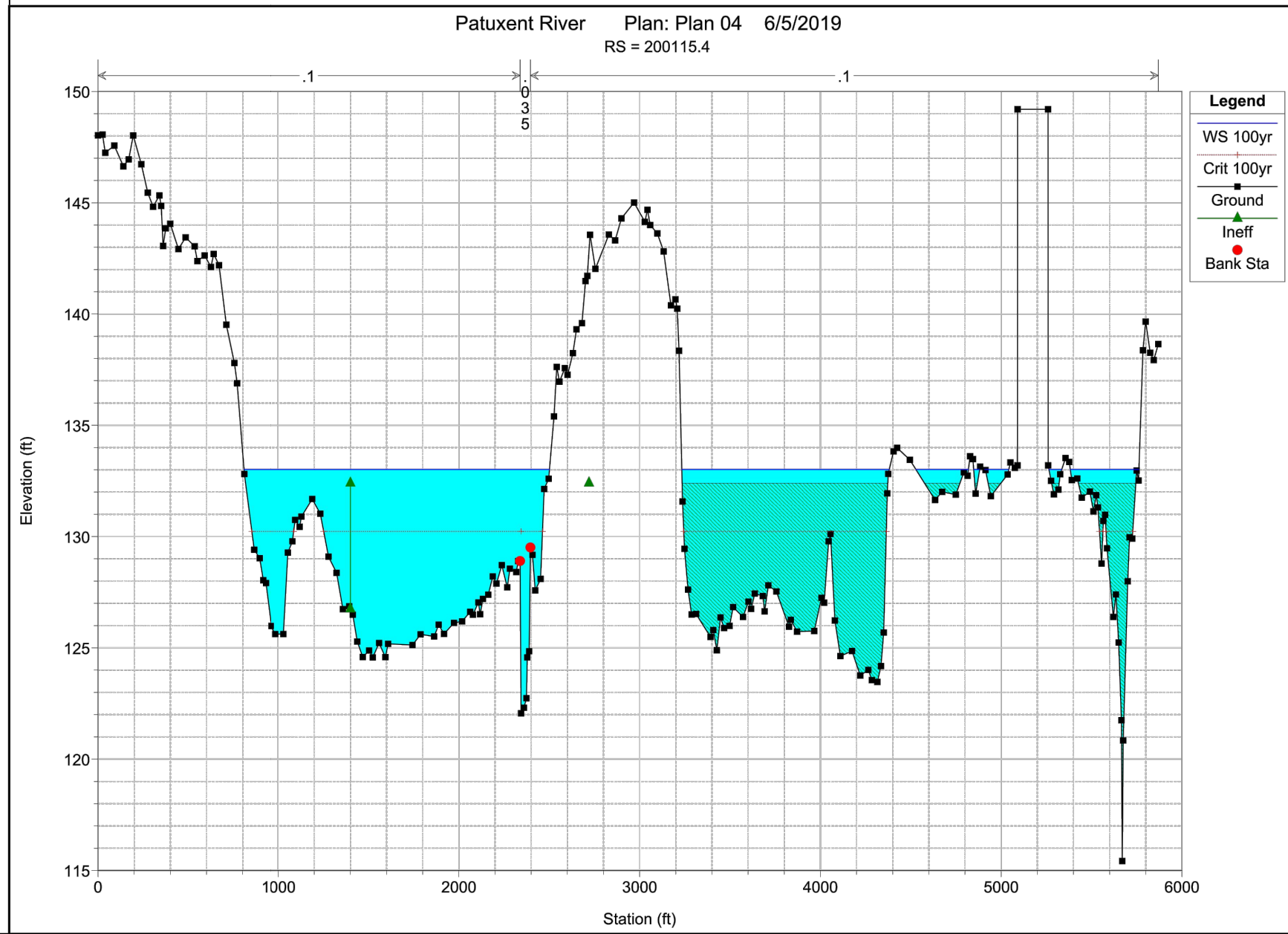
CROSS-SECTION 200115.4
