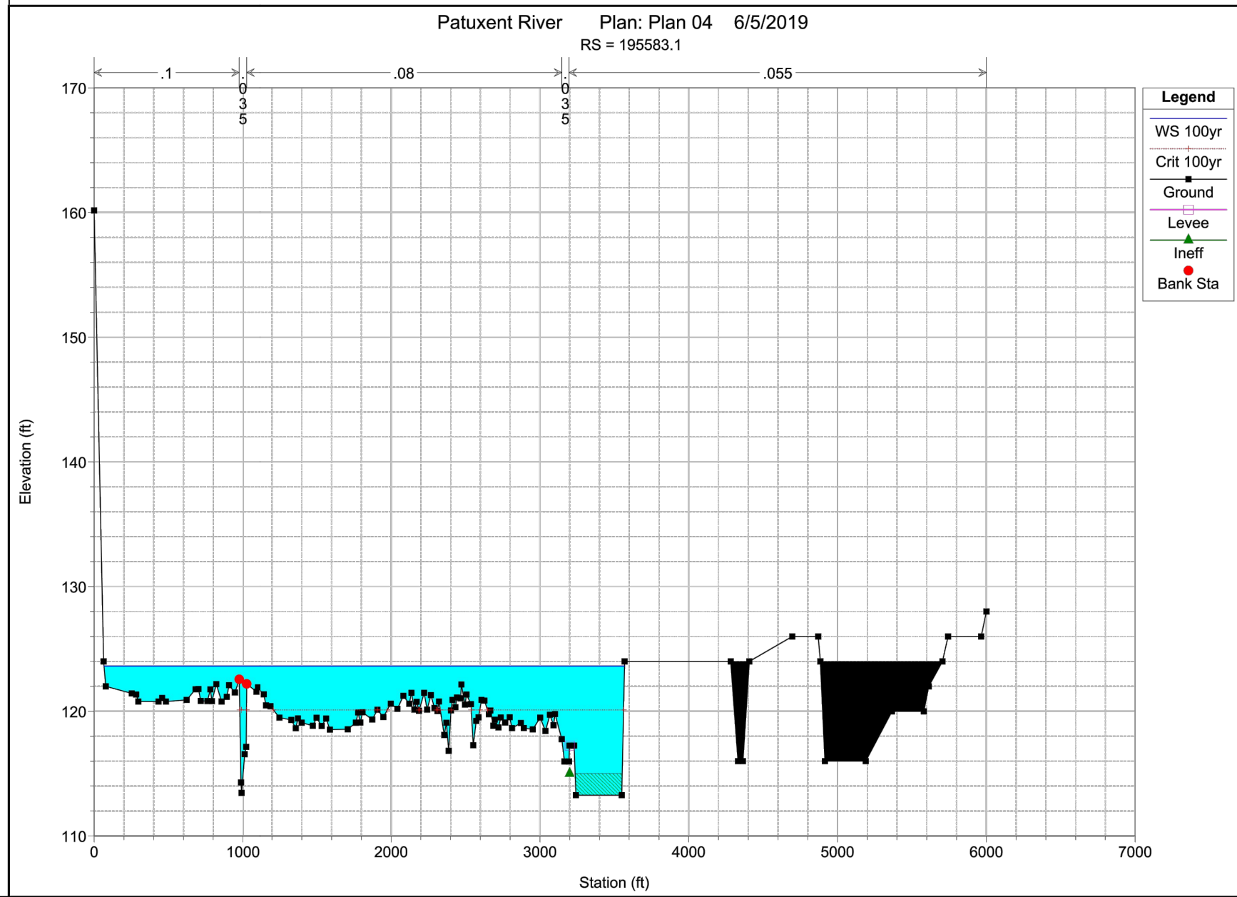
CROSS-SECTION 195583.1
