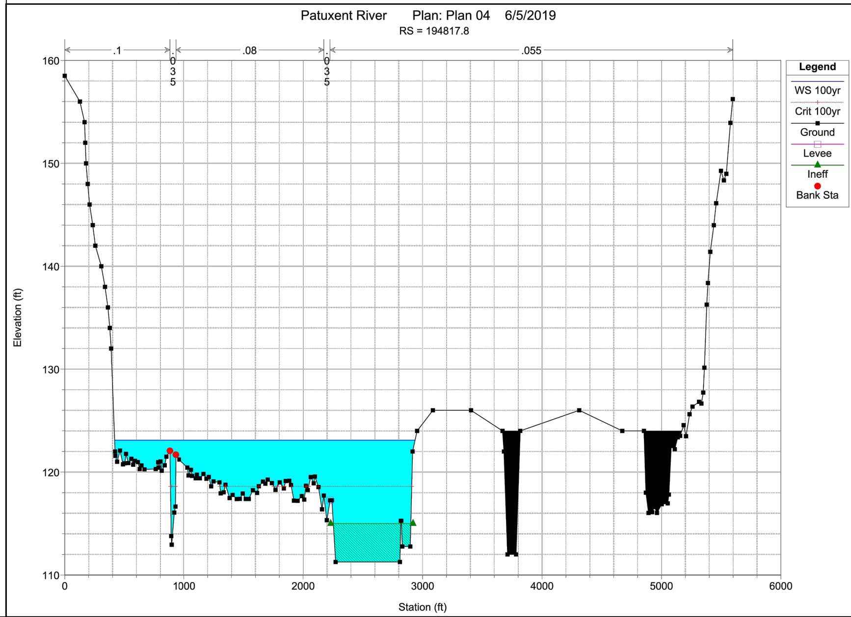
CROSS-SECTION 194817.8
