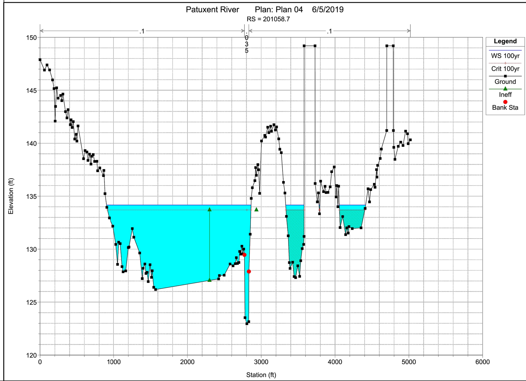
CROSS-SECTION 201058.7
