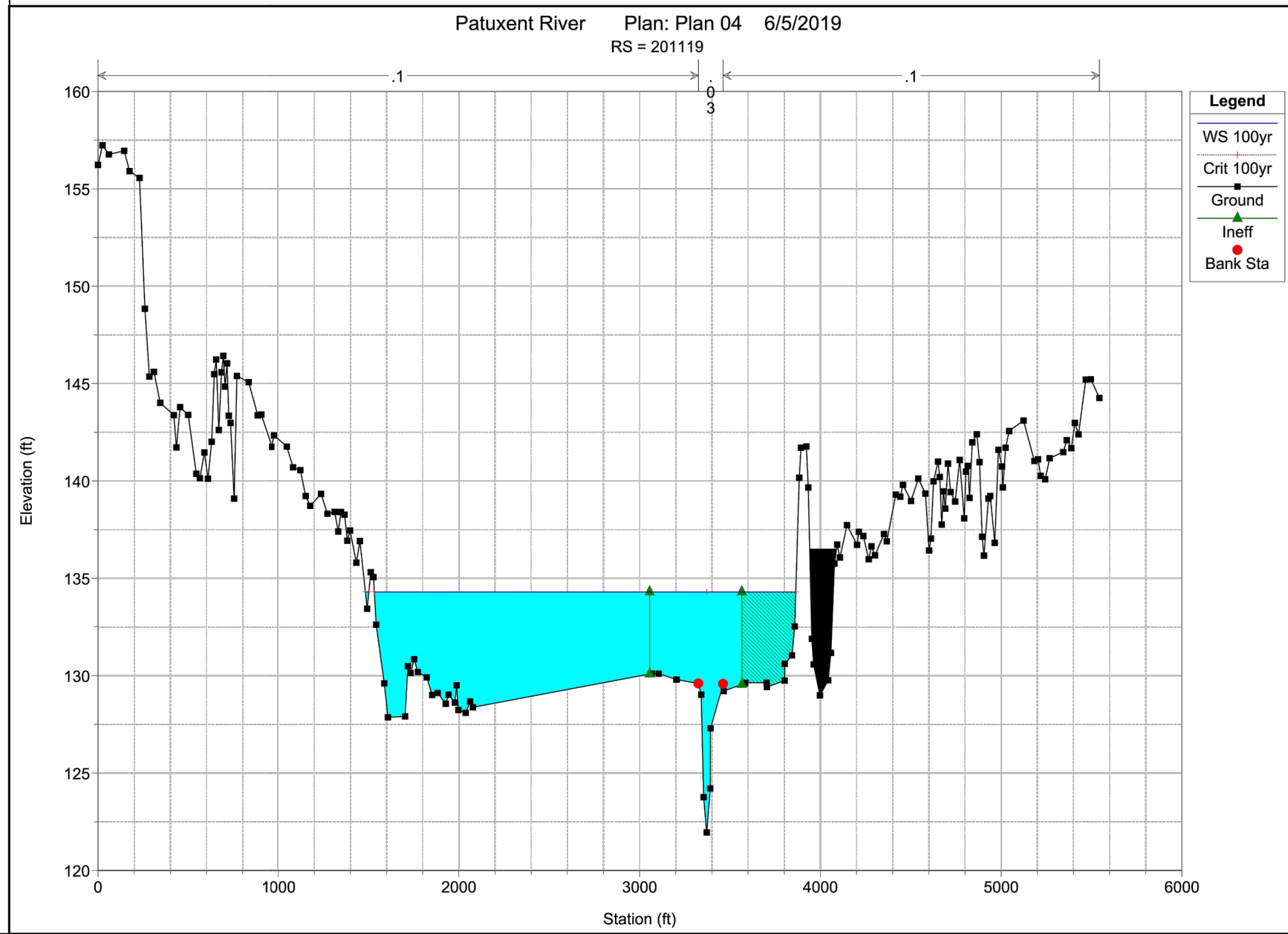
CROSS-SECTION 201119
