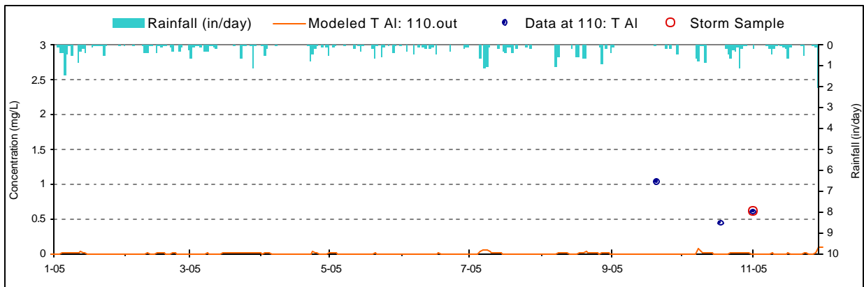
Figure F-21. Aluminum Validation plot for North Branch Laurel Run (NXB0003/BM915)
