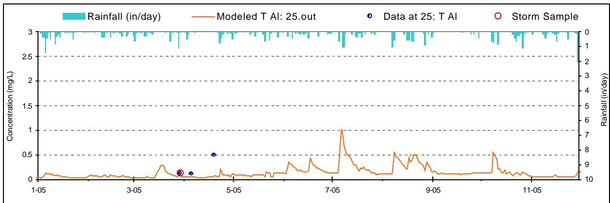
Figure F-9. Aluminum Calibration plot for UT to Bear Creek (ZWI0000/WM-21)
