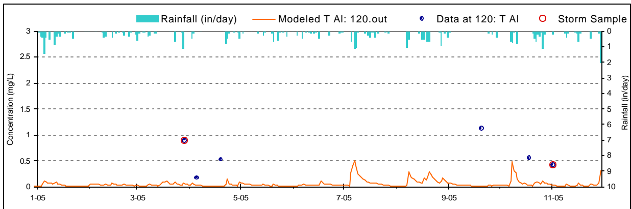
Figure F-18. Aluminum Validation plot for Laurel Run (LAU0013/WM-15)
