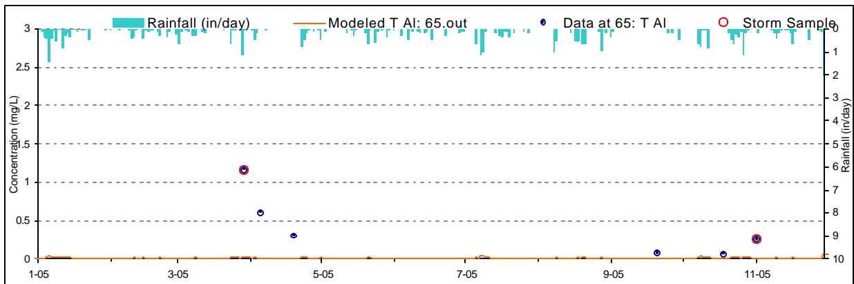
Figure F-3. Aluminum Calibration plot for Laurel Run (LRL0034/BM929)
