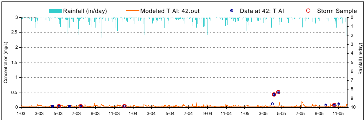
Figure F-1. Aluminum Calibration plot for Herrington Creek (HER0014/WM-8)
