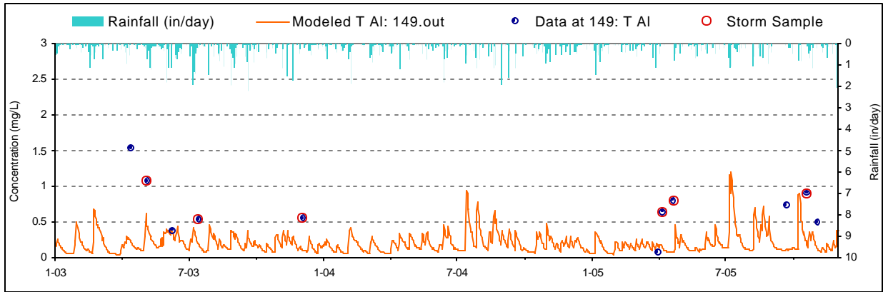
Figure F-25. Aluminum Validation plot for UT to Glade Run (UGB0002/BM913)
