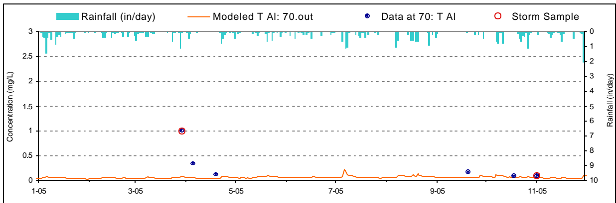
Figure F-5. Aluminum Calibration plot for Muddy Creek (MYC0018/WM-17)
