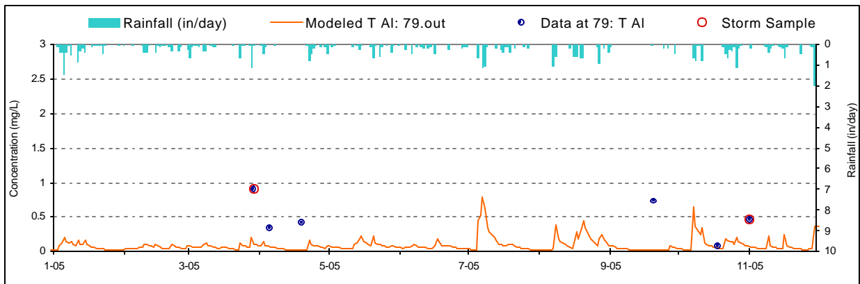
Figure F-19. Aluminum Validation plot for Millers Run (MLR0001/WM-12)
