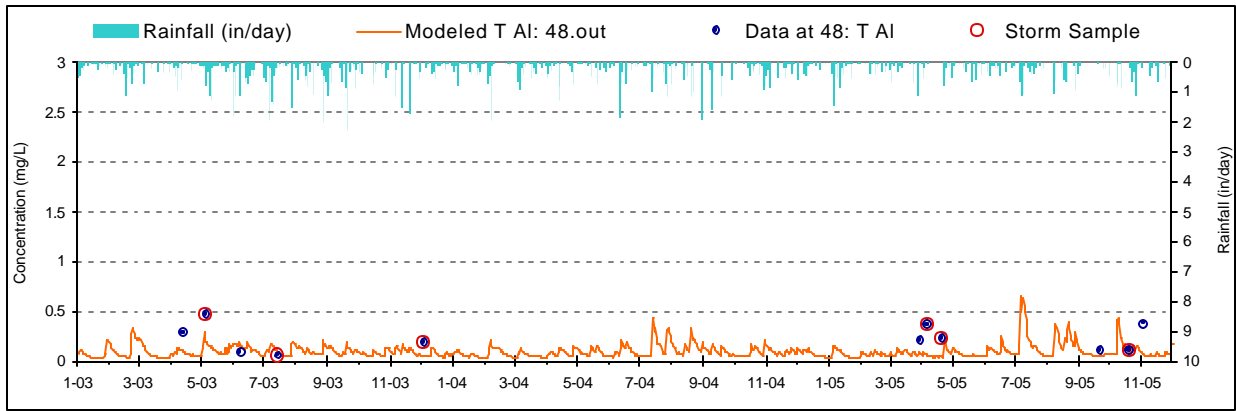
Figure F-7. Aluminum Calibration plot for Toliver Run (TOL001/WM-14)
