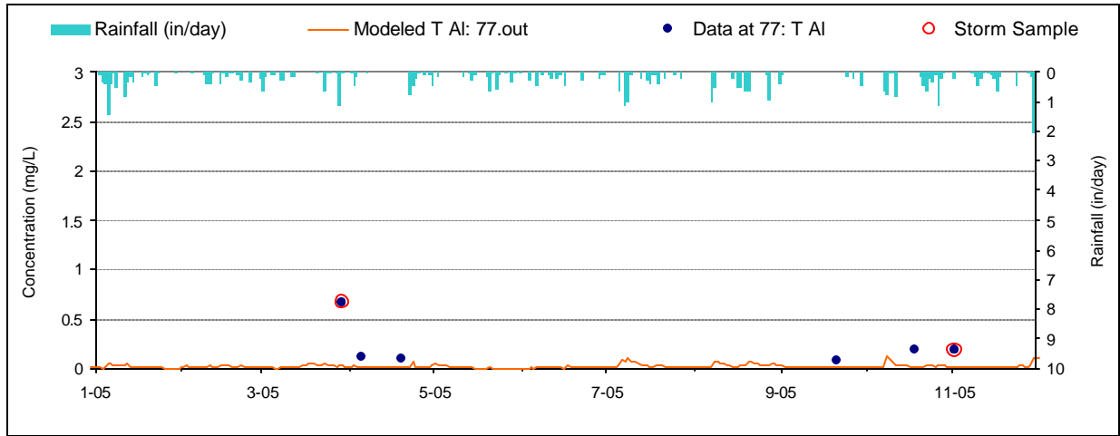
Figure F-1. Aluminum Calibration plot for Herrington Creek (HER0014/WM-8)
