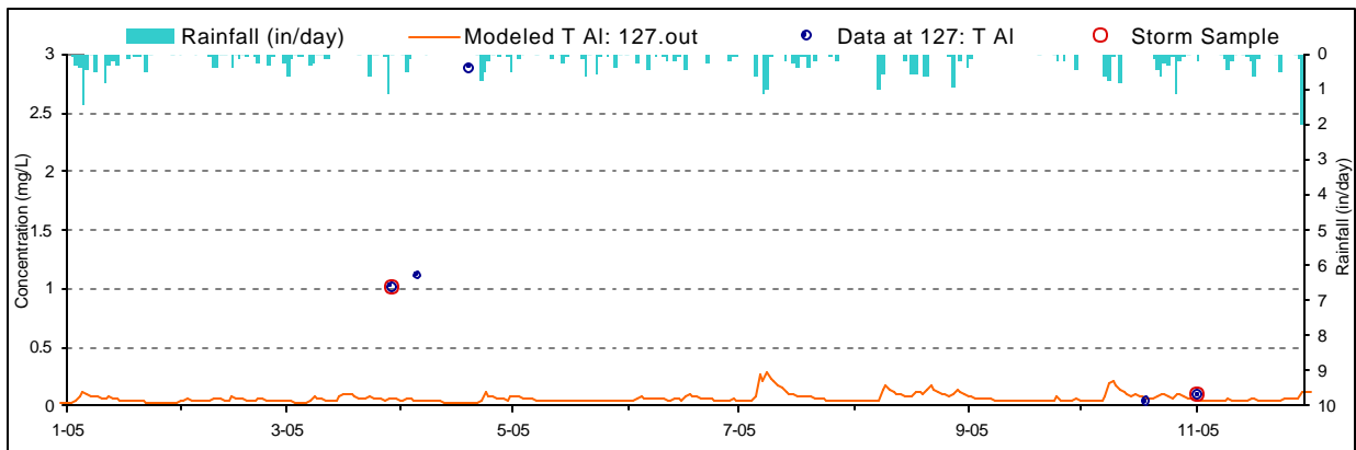
Figure F-15. Aluminum Validation plot for Bull Glade Run (BUG0013/WM-10)
