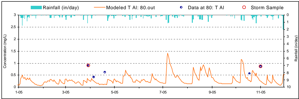
Figure F-23. Aluminum Validation plot for UT to Bull Glade Run (UBL0000/WM-11)
