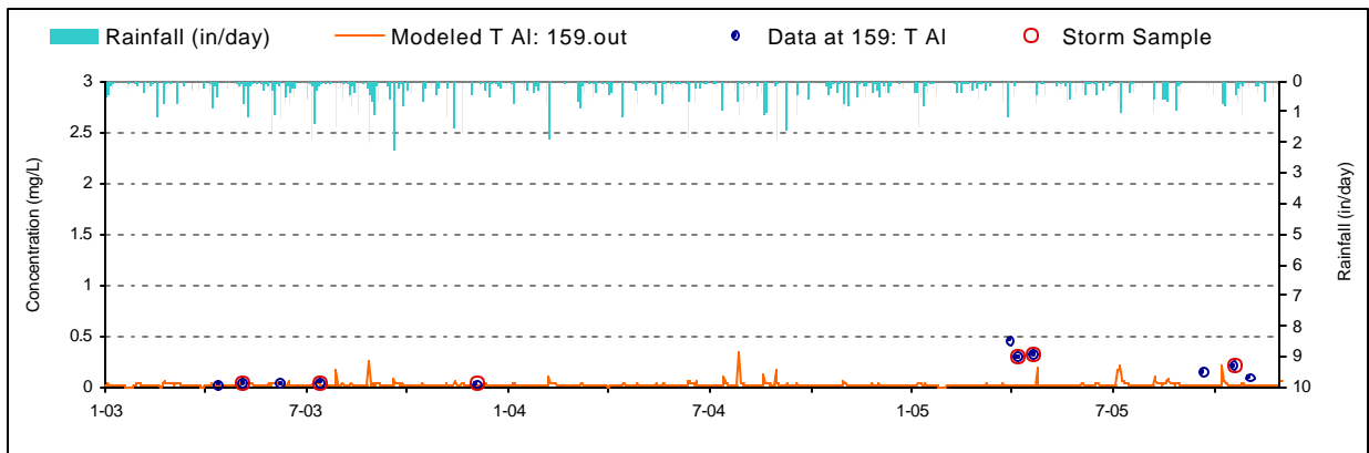
Figure F-13. Aluminum Calibration plot for White Rock Run (WRR0008/BM931)
