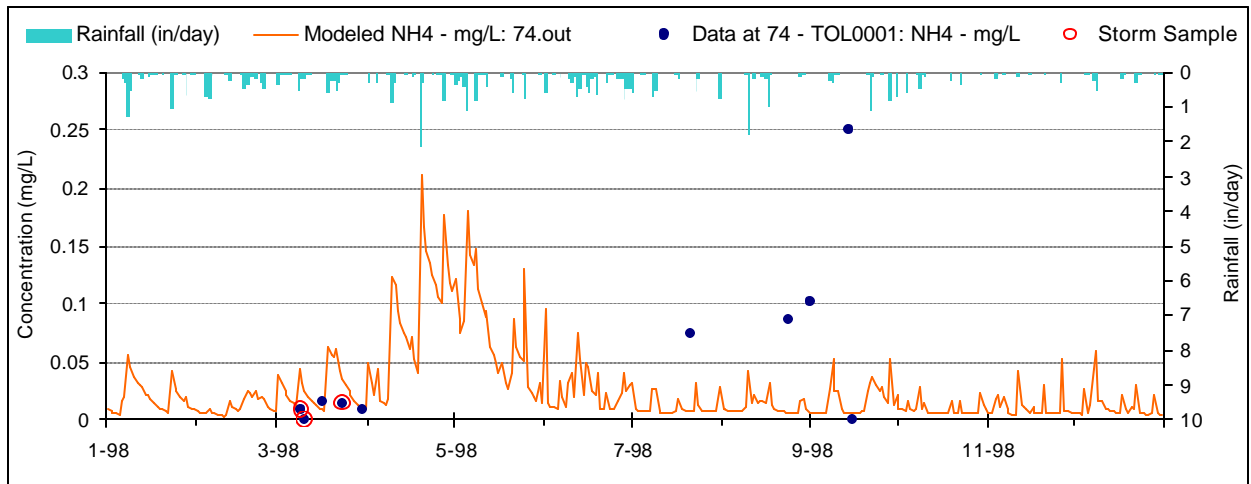
Figure I-2. Ammonium Calibration plot for Tolver Run (TOL0001/WM-14)
