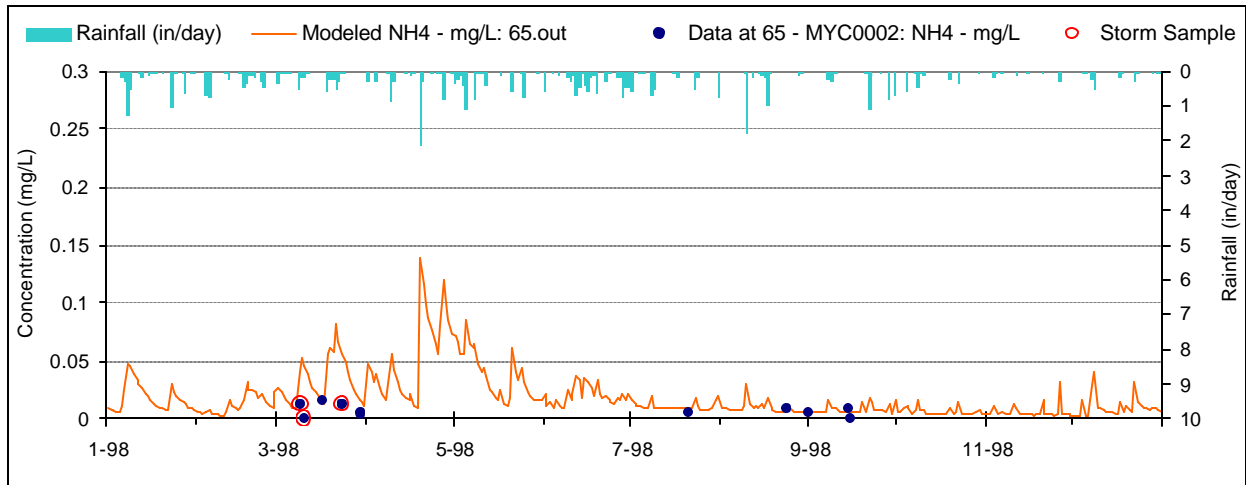
Figure I-1. Ammonium Calibration plot for Muddy Creek (MYC0002/WM-1)
