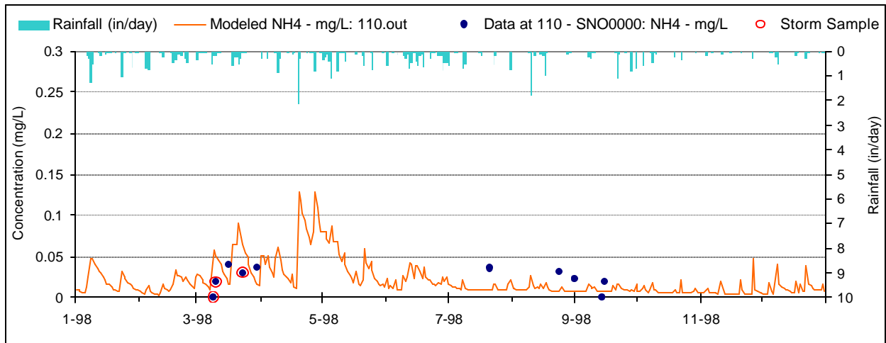
Figure I-3. Ammonium Validation plot for Snowy Creek (SNO0000/WM-2)
