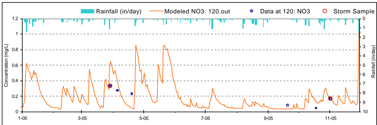
Figure H-17. Nitrate Validation plot for Herrington Creek (HER0028/WM-4)
