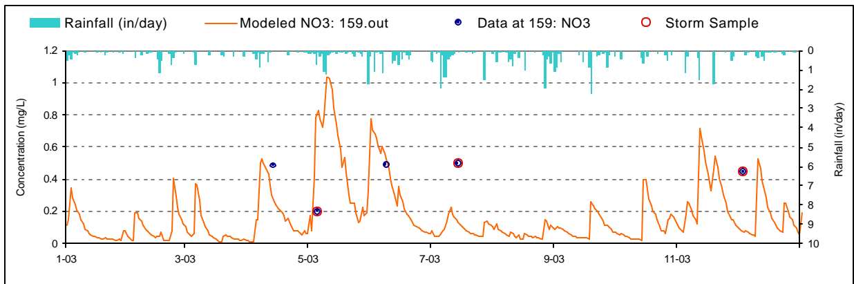
Figure H-13. Nitrate Calibration plot for White Rock Run (WRR008/BM931)
