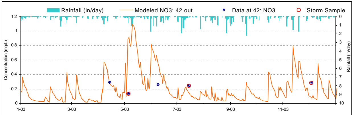
Figure H-1. Nitrate Calibration plot for Herrington Creek (HER0014/WM-8)
