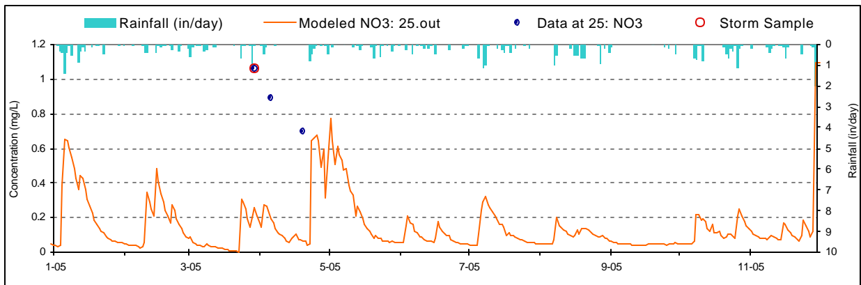
Figure H-9. Nitrate Calibration plot for UT to Bear Creek (ZWI0000/WM-21)
