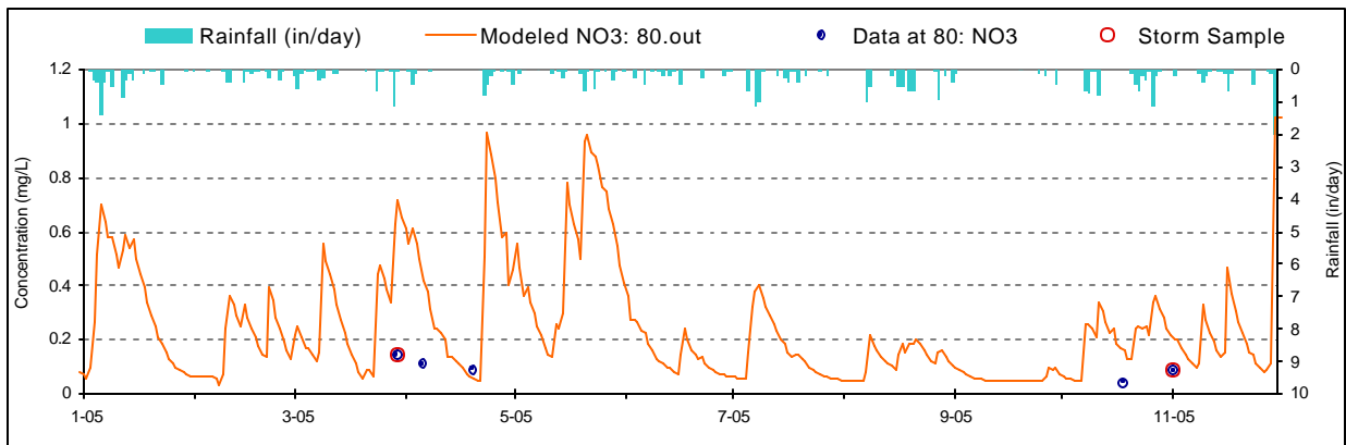
Figure H-23. Nitrate Validation plot for UT to Bull Glade Run (UBL0000/WM-11)
