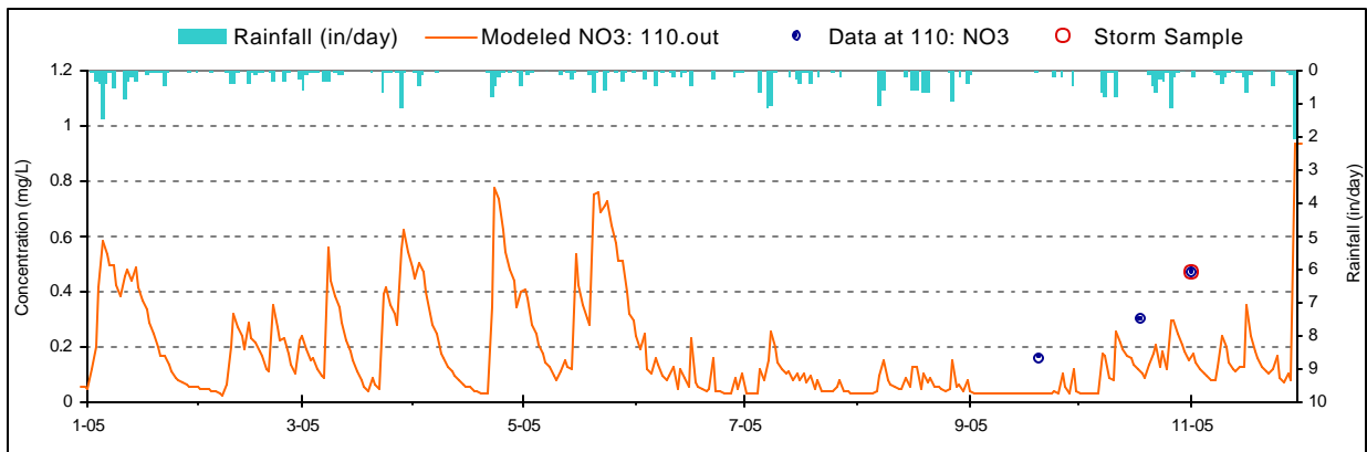
Figure H-21. Nitrate Validation plot for North Branch Laurel Run (NXB0003/BM915)
