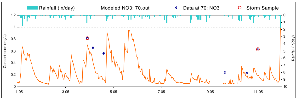
Figure H-5. Nitrate Calibration plot for Muddy Creek (MYC0018/WM-17)
