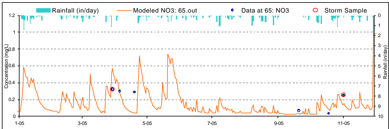
Figure H-3. Nitrate Calibration plot for Laurel Run (LRL0034/BM929)
