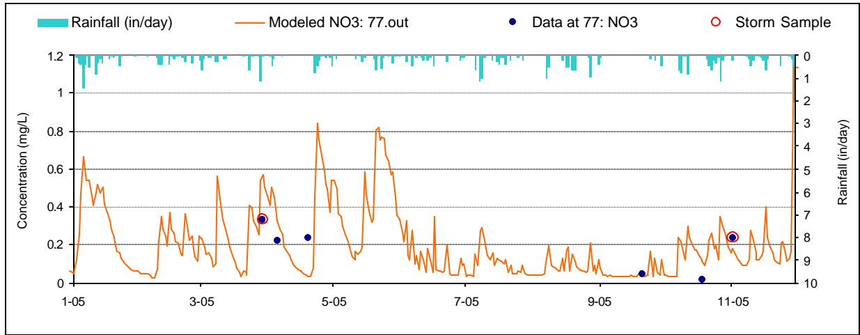
Figure H-1. Nitrate Calibration plot for Herrington Creek (HER0014/WM-8)
