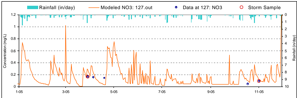
Figure H-15. Nitrate Validation plot for Bull Glade Run (BUG0013/WM-10)
