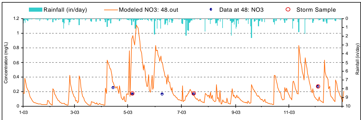
Figure H-7. Nitrate Calibration plot for Toliver Run (TOL0001/WM-14)
