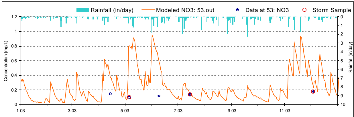
Figure H-11. Nitrate Calibration plot for UT to Mill Run (ZWH0000/WM-26)
