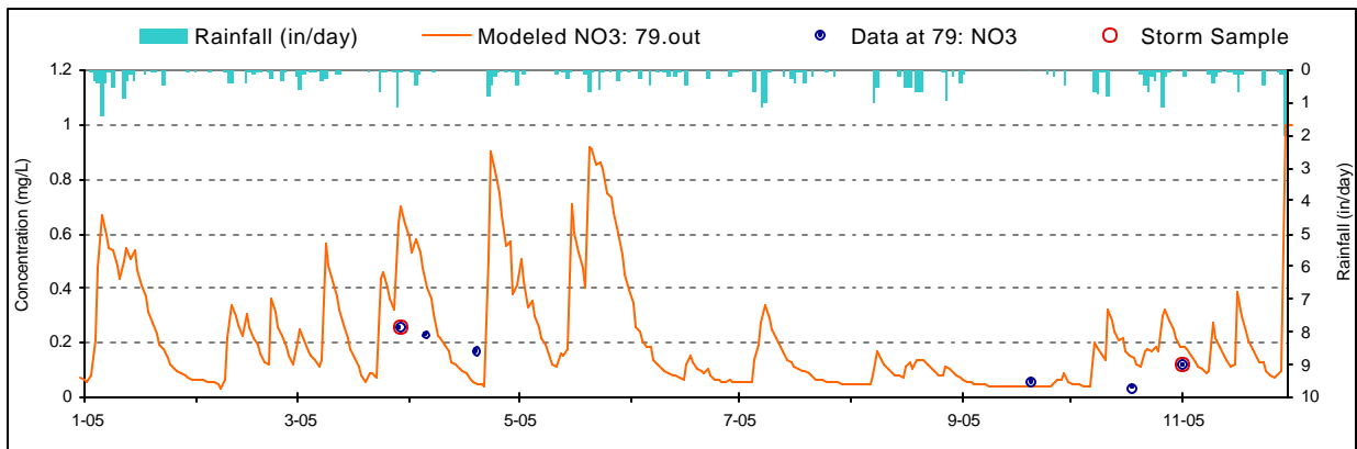
Figure H-19. Nitrate Validation plot for Millers Run (MLR0001/WM-12)
