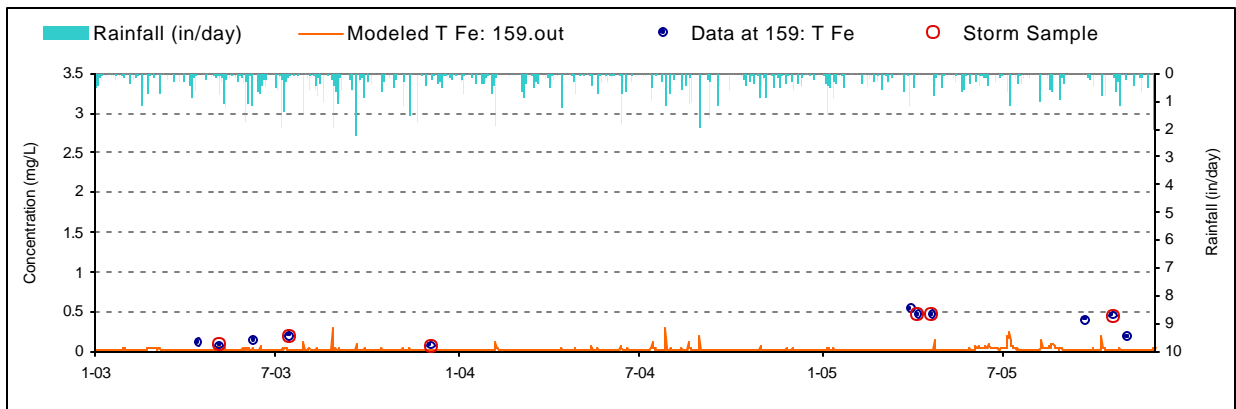
Figure E-13. Iron Calibration plot for White Rock Run (WRR0008/BM931)
