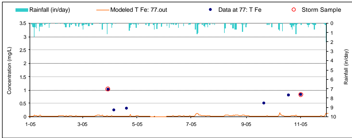
Figure E-1. Iron Calibration plot for Herrington Creek (HER0014/WM-8)
