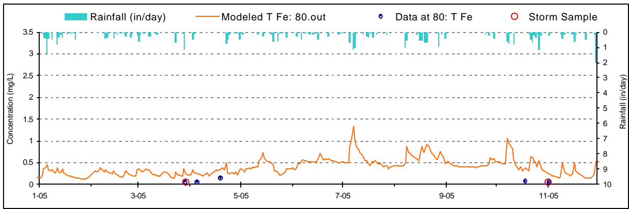
Figure E-23. Iron Validation plot for UT to Bull Glade Run (UBL0000/WM-11)
