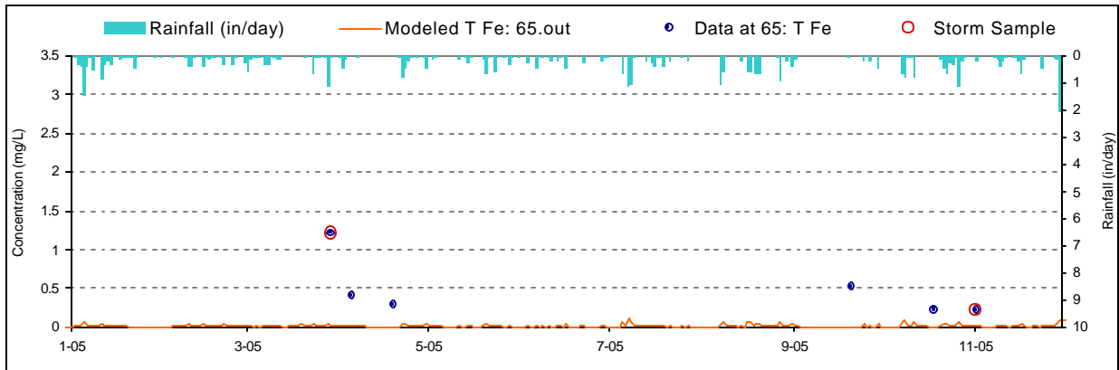
Figure E-3. Iron Calibration plot for Laurel Run (LRL0034/BM929)
