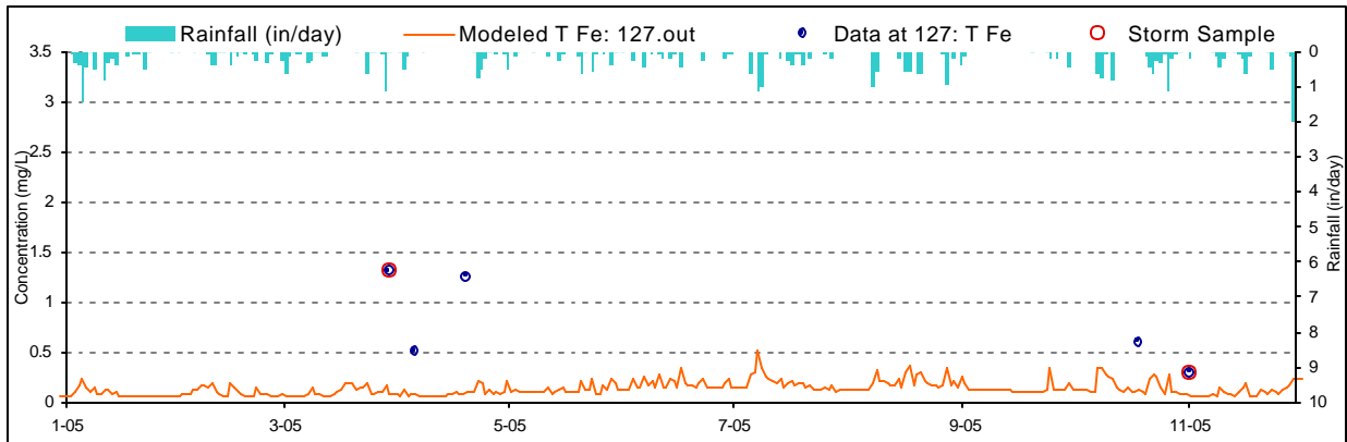
Figure E-15. Iron Validation plot for Bull Glade Run (BUG0013/WM-10)
