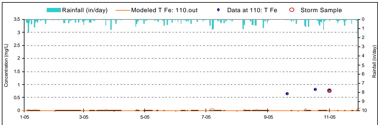
Figure E-21. Iron Validation plot for North Branch Laurel Run (NXB0003/BM915)
