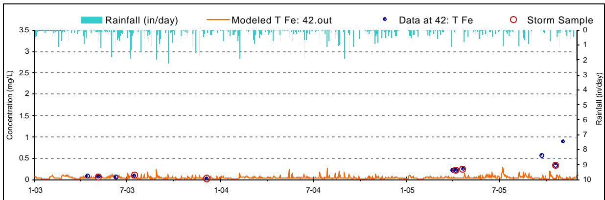
Figure E-1. Iron Calibration plot for Herrington Creek (HER0014/WM-8)
