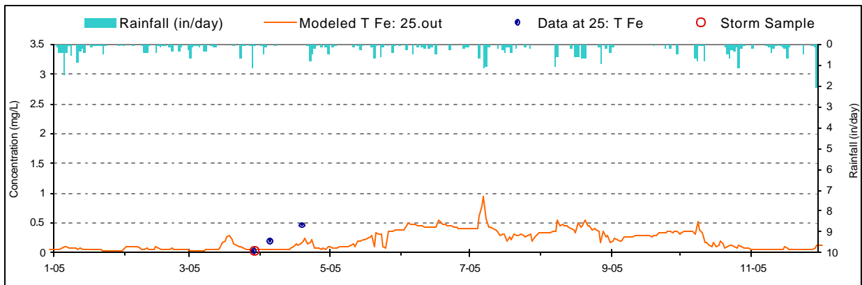
Figure E-9. Iron Calibration plot for UT to Bear Creek (ZWI0000/WM-21)
