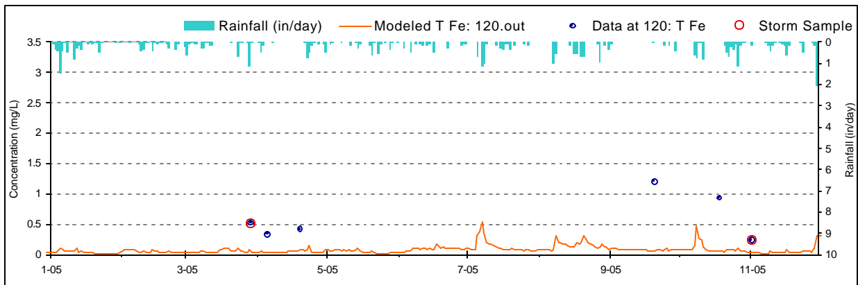
Figure E-17. Iron Validation plot for Herrington Creek (HER0028/WM-4)
