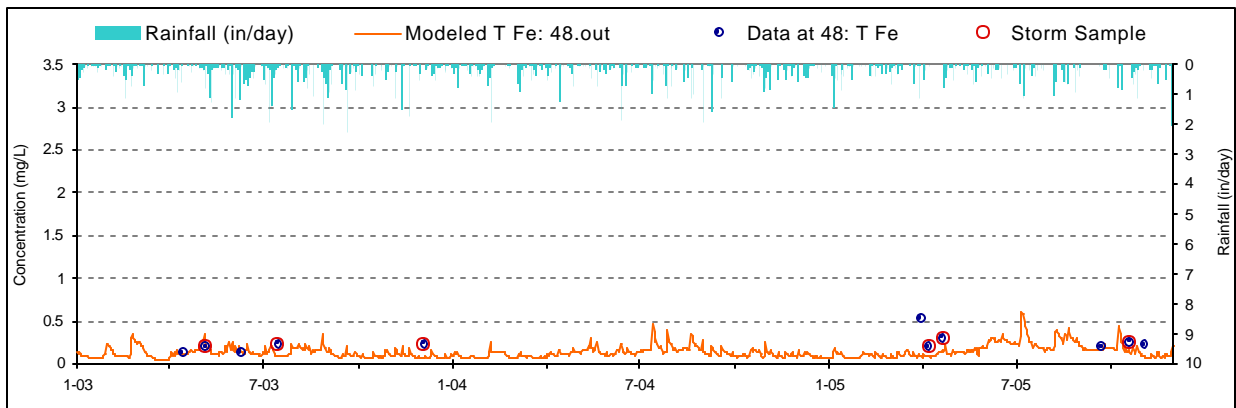
Figure E-7. Iron Calibration plot for Toliver Run (TOL0001/WM-14)
