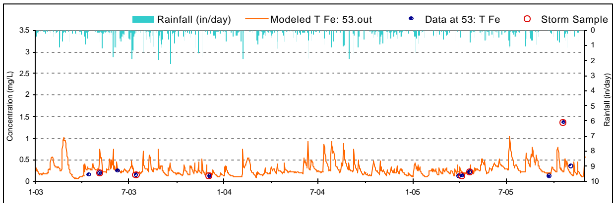
Figure E-11. Iron Calibration plot for UT to Mill Run (ZWH0000/WM-26)
