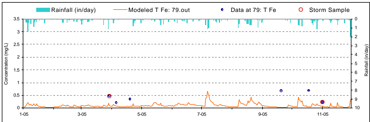
Figure E-19. Iron Validation plot for Millers Run (MLR0001/WM-12)
