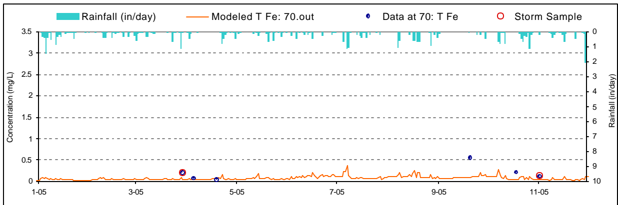
Figure E-5. Iron Calibration plot for Muddy Creek (MYC0018/WM-17)
