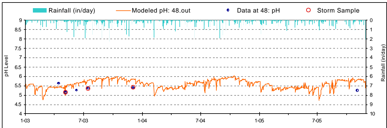
Figure D-8. pH Calibration plot for Trap Run (TRR007/BM930)
