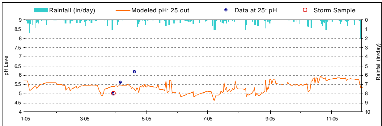
Figure D-10. pH Calibration plot for UT to Little Bear Creek (ZWL0005/WM-22)
