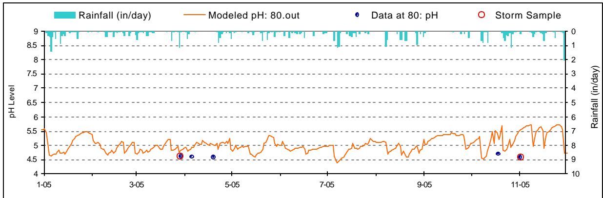
Figure D-23. pH Validation plot for UT to Bull Glade Run (UBL0000/WM-11)
