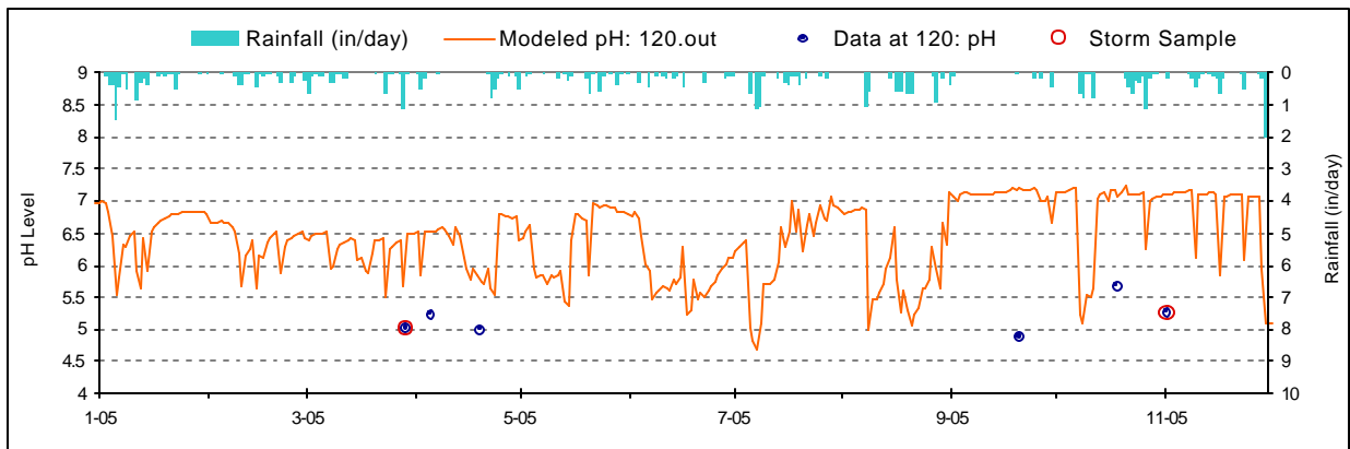
Figure D-17. pH Validation plot for Herrington Creek (HER0028/WM-4)
