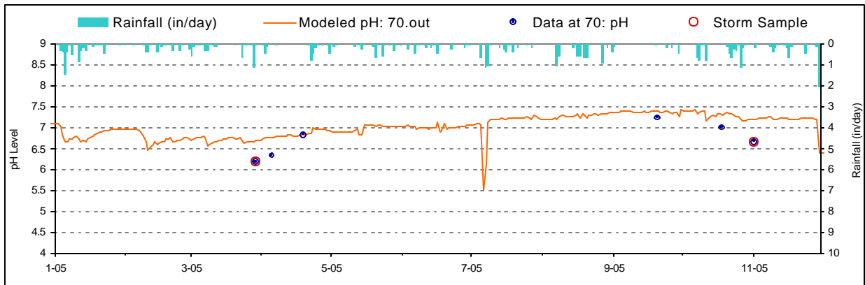
Figure D-5. pH Calibration plot for Muddy Creek (MYC0018/WM-17)
