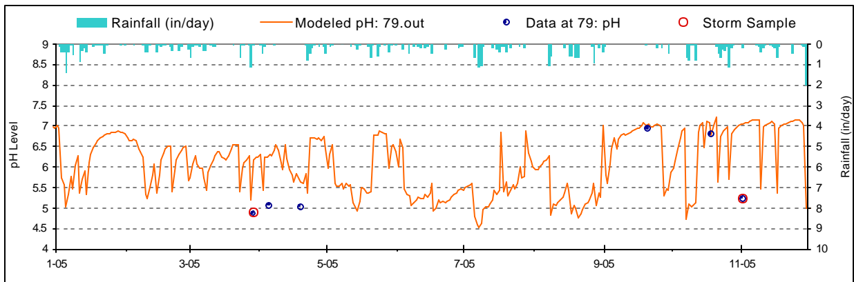
Figure D-19. pH Validation plot for Millers Run (MLR0001/WM-12)
