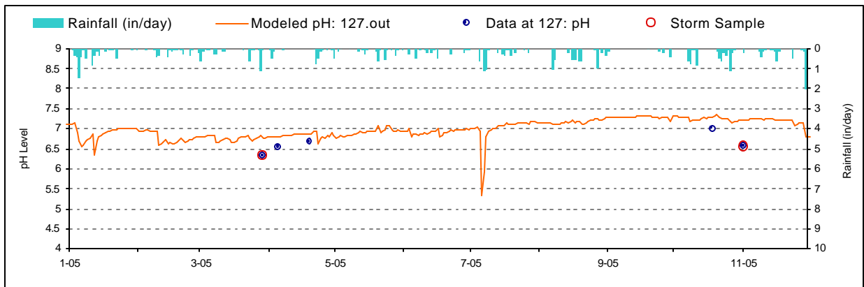
Figure D-15. pH Validation plot for Bull Glade Run (BUG0013/WM-10)
