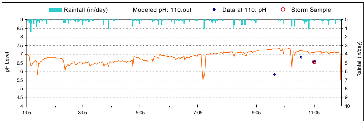
Figure D-21. pH Validation plot for North Branch Laurel Run (NXB0003/BM915)
