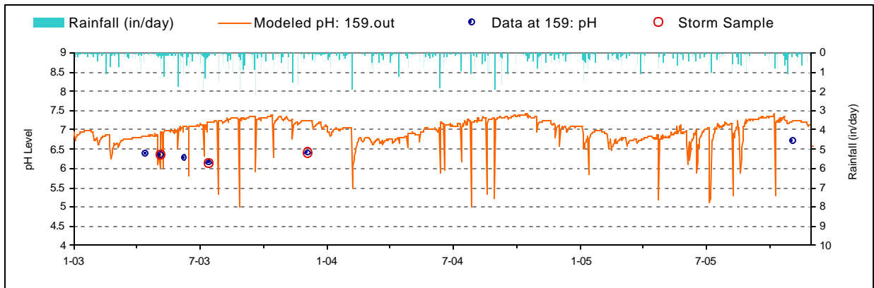
Figure D-13. pH Calibration plot for White Rock Run (WRR0008/BM931)
