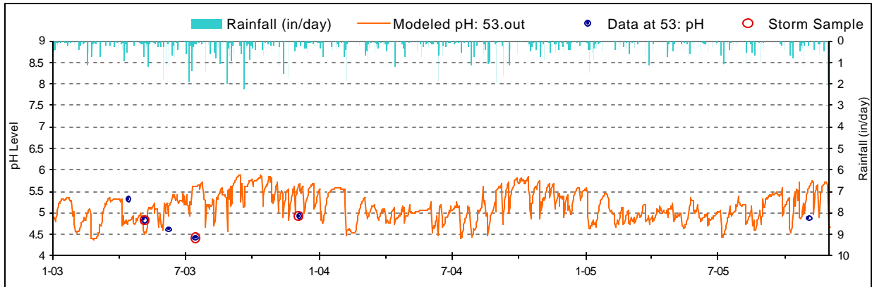
Figure D-11. pH Calibration plot for UT to Mill Run (ZWH0000/WM-26)
