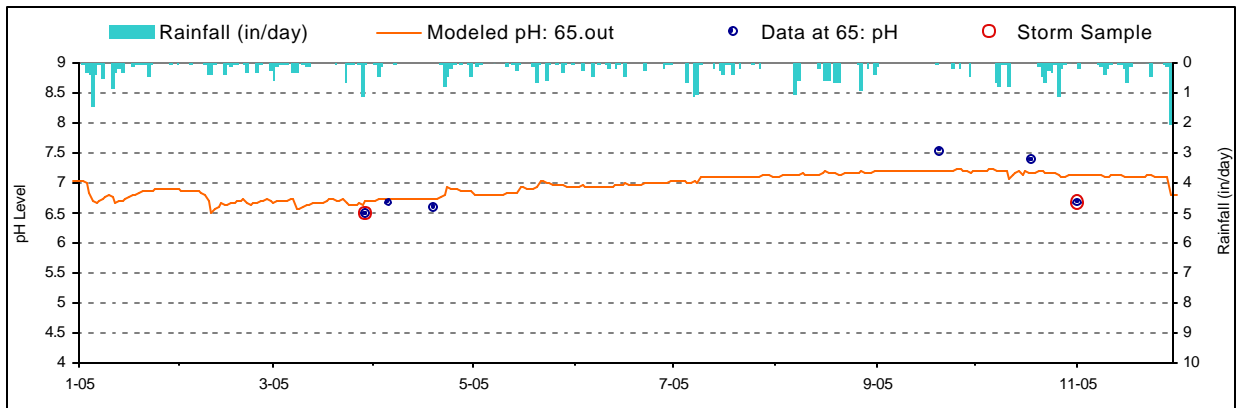
Figure D-3. pH Calibration plot for Laurel Run (LRL0034/BM929)
