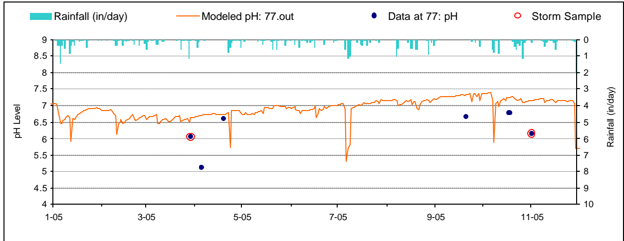
Figure D-1. pH Calibration plot for Herrington Creek (HER0014/WM-8)
