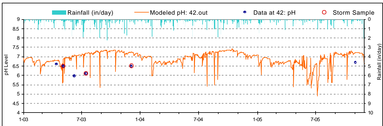
Figure D-1. pH Calibration plot for Herrington Creek (HER0014/WM-8)
