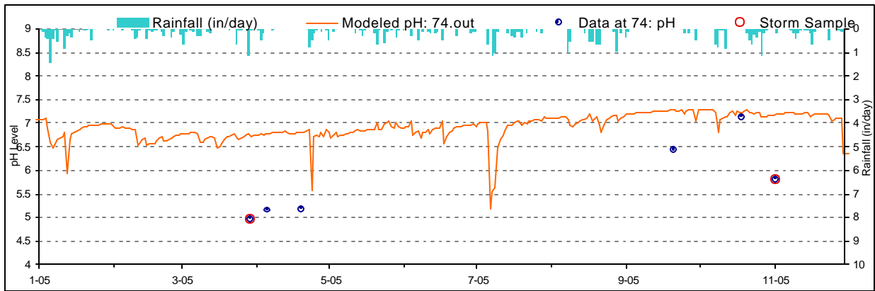
Figure D-7. pH Calibration plot for Toliver Run (TOL001/WM-14)
