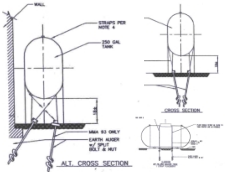
Diagrams showing proper tank anchoring methods
