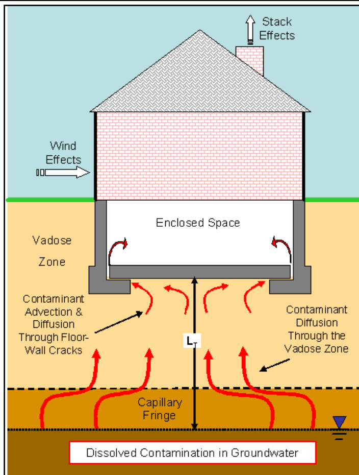
Conceptual Diagram of Vapor Intrusion into Building
