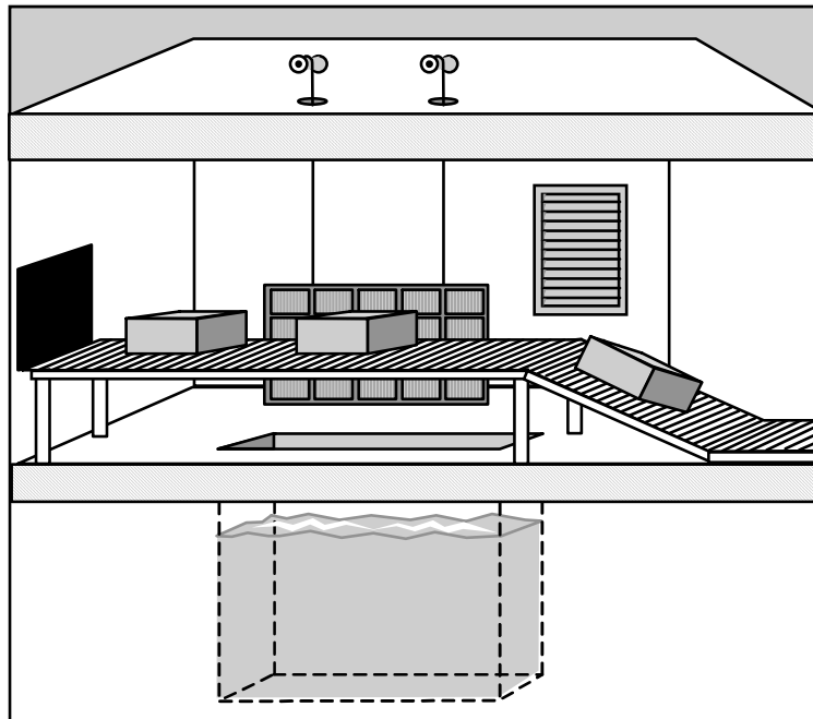
Figure 1.3 Commercial Wet-Source-Storage Irradiator. The sealed sources are stored in water and raised into the air to irradiate a product that may be moved into the irradiation room on a conveyor system. This is an example of a panoramic wet-source-storage irradiator.
