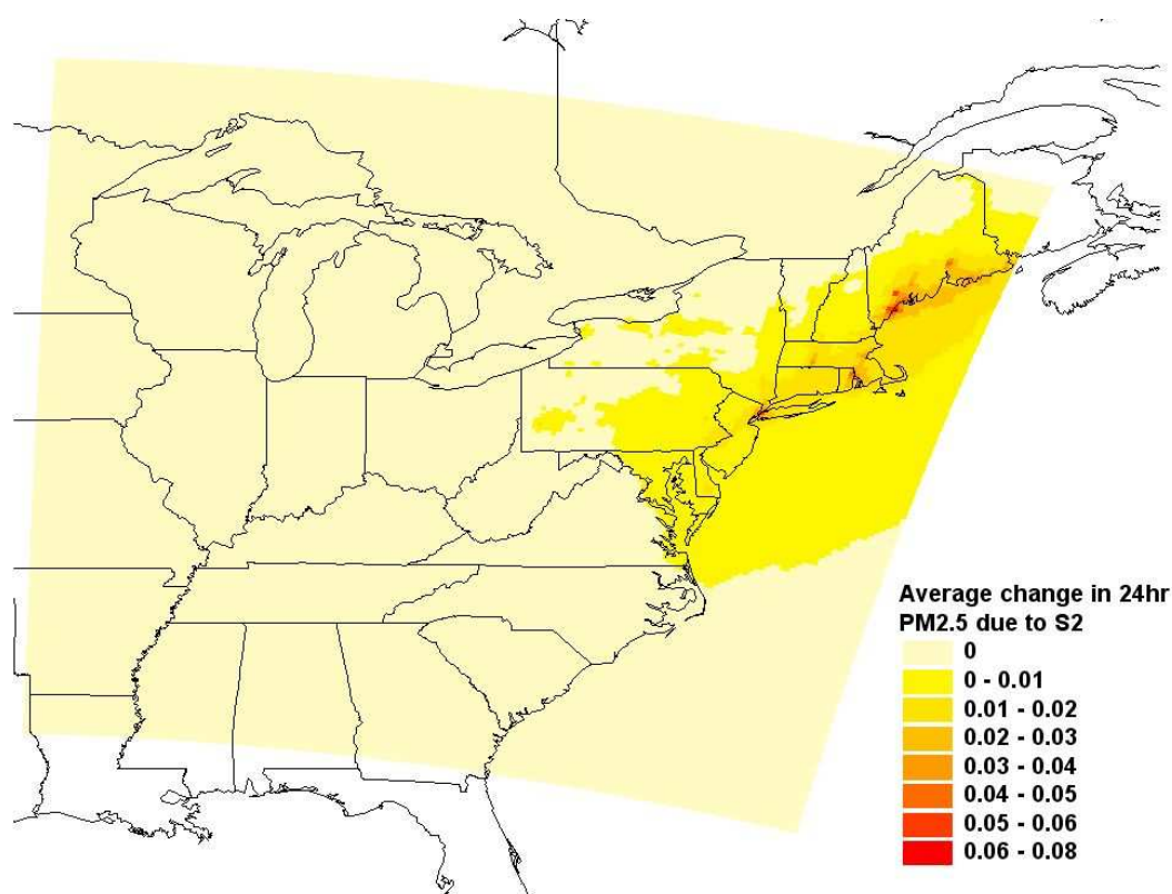
Figure 5-2. Average change in 24-hr PM 2.5 due to S2 emission reductions, relative to S1 ( \mu\text{g}/\text{m}^3 )
