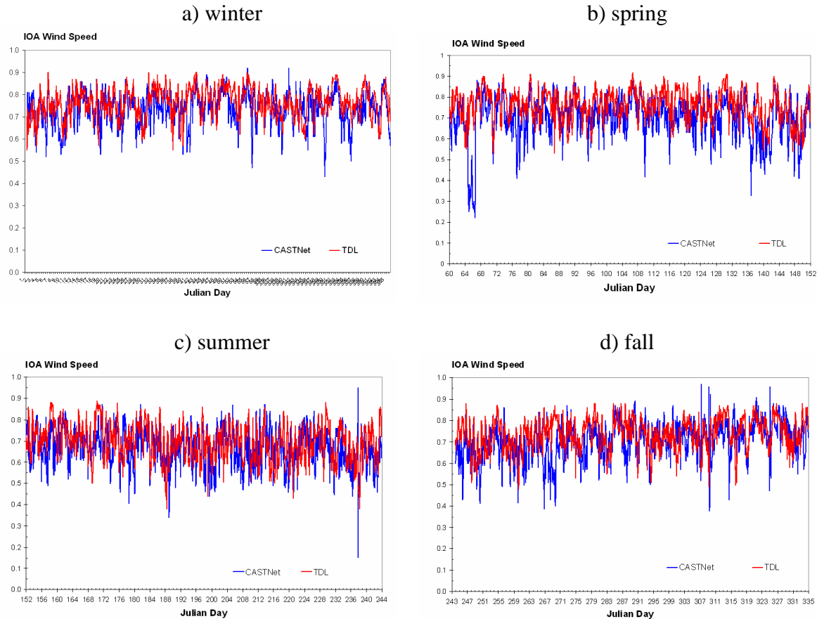
Figure 2-2. 2002 seasonal hourly average index of agreement for wind speed
