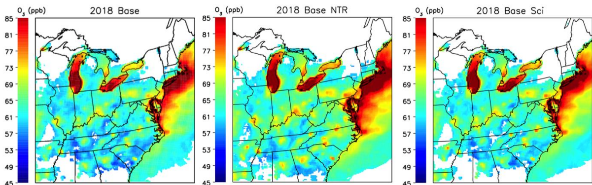
Figure 3.4. Same as Figure 3.3 except all simulations are for July 2018,
