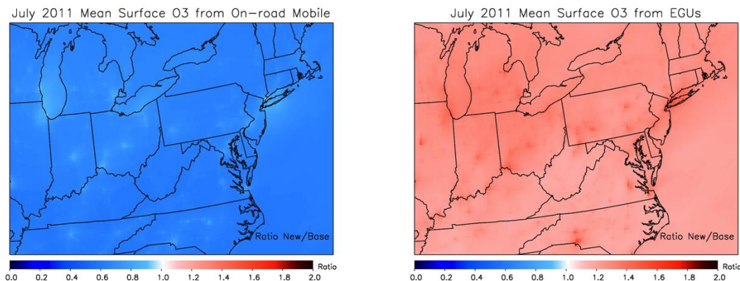
Figure 3b.6. The fractional change in surface ozone from on-road mobile sources (left) and Electricity Generation Units [EGUs] (right) during July 2011 due to the change from the baseline model to the updated "Beta" model. Cool (warm) colors show where the change led to a decrease (increase) in the importance of each source.
