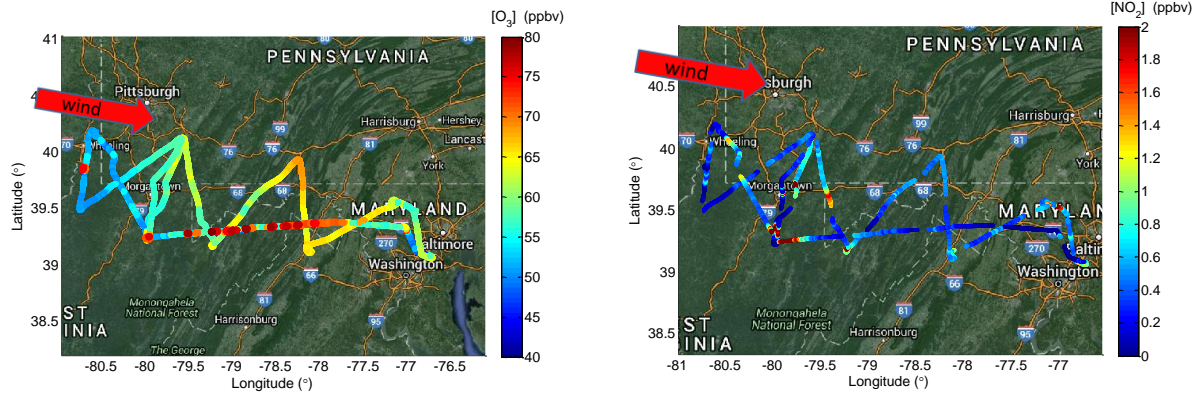
Figure 4.7. Ozone (left) and NO_2 (right) mixing ratios observed along the flight path during a fracking flight on September 14, 2015.
