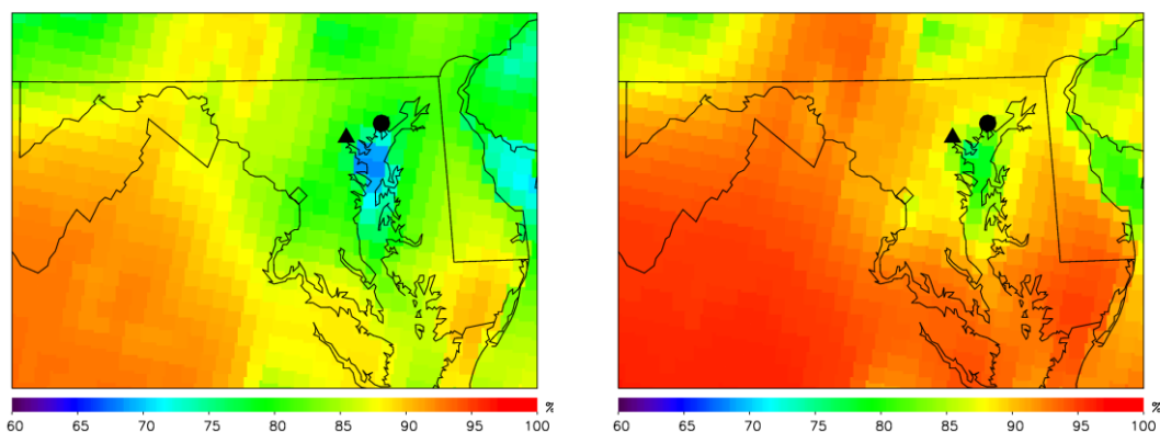
Figure 3b.7. Percentage of ozone formed in a \text{NO}_x -limited production regime during July 2011 daytime mean (8 AM – 8 PM local time) at each model grid point in the (left) baseline simulation and (right) updated chemistry and emissions scenario.
