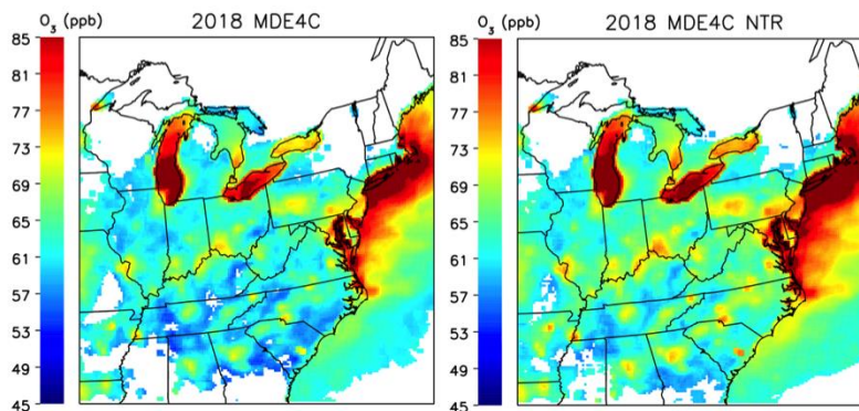
Figure 3.7: Same as Figure 3.4 except baseline and NTR simulations are for Scenario 4C
