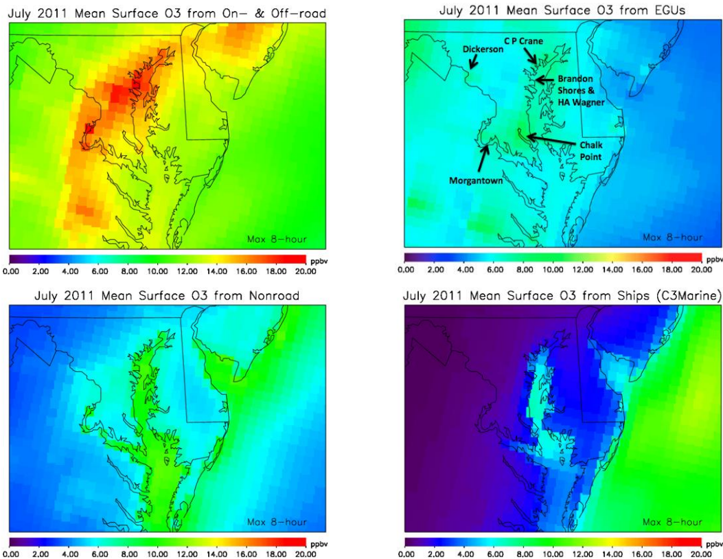
Figure 3b.3. APCA source attribution from the baseline simulation for mean 8-hour maximum ozone during July 2011 for the following source sectors: (top left) on- and off-road mobile sources, (top right) electricity generating units, (bottom left) nonroad mobile sources, and (bottom right) large marine vessels.
