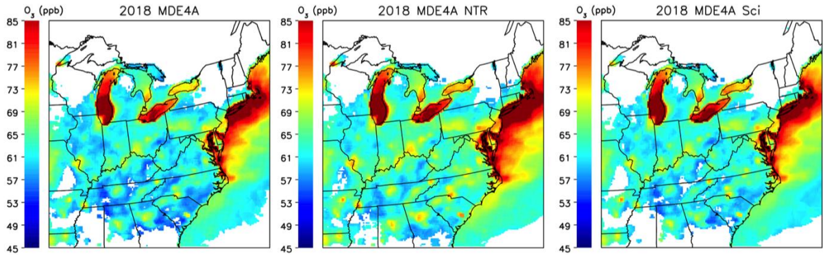
Figure 3.5: Same as Figure 3.4 except all simulations are for July 2018, Scenario 4A
