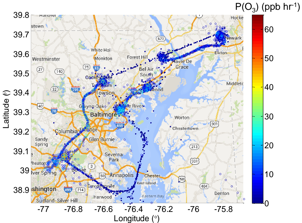
Figure 4.2. P(O_3) : Net ozone production rate, net P(O_3) calculated using the box model results along the P-3B flight track during DISCOVER-AQ in Maryland in 2011. The size of dots is proportional to P(O_3) .
