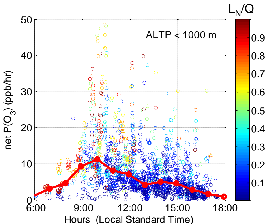
Figure 4.3. Diurnal variation of ozone production rate colored with the indicator L_N/Q on ten flight days during DISCOVER-AQ in Maryland in 2011. The solid red circles represent the median values in hourly bins of P(O_3) . Data are limited with the pressure altitude less than 1000 m to represent the lowest layer of the atmosphere.
