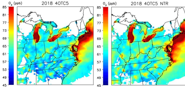
Figure 3.15. Same as Figure 3.7 except baseline and NTR simulations are for Scenario 4OTC5
