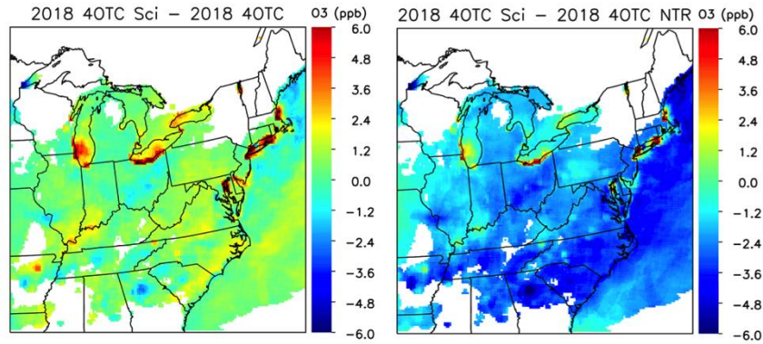
Figure 3.10. Difference between 40TC Science and 40TC baseline model runs (Left). Difference between 40TC Science and 40TC NTR model runs (Right).
