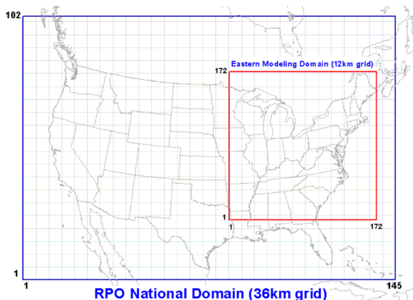
Figure 2: Weight of Evidence Modeling Domain
