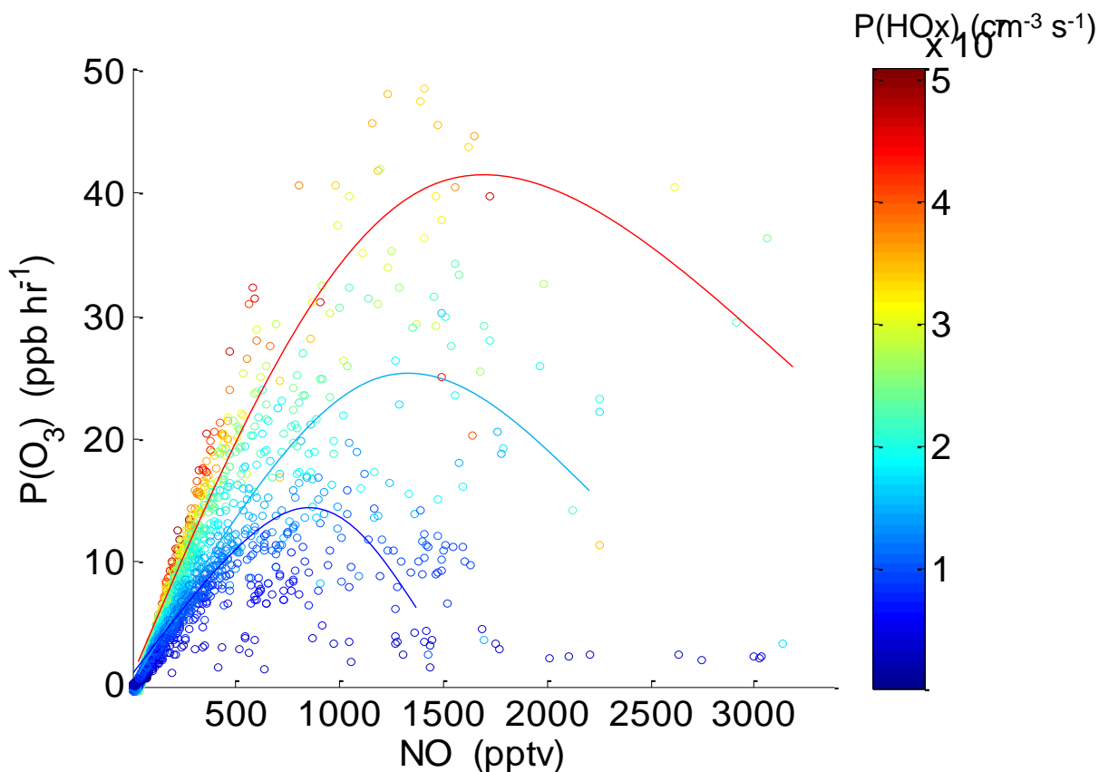
Figure 4.4. Ozone production as a function of NO mixing ratio. Individual data points are the 1-minute averages and are colored with the production rate of HOx (= OH + HO 2 ) during DISCOVER-AQ in Maryland in 2011. The colored lines represent the dependence of P(O 3 ) as function of NO at different P(HOx) levels.
