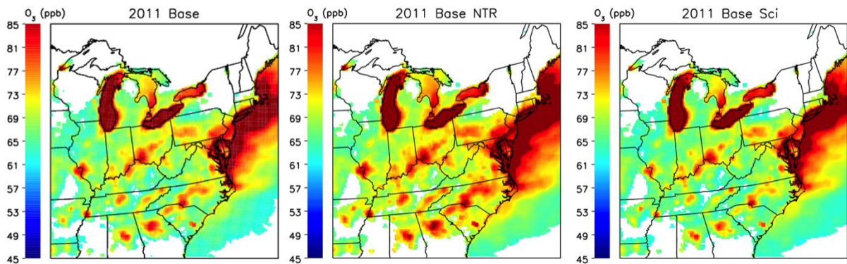
Figure 3.3. Average maximum 8hr O 3 for July 2011 baseline model simulation (left panel); simulation where the lifetime of NTR has been decreased (middle panel), NTR lifetime is decreased and onroad mobile NO x has been decreased by 50%.
