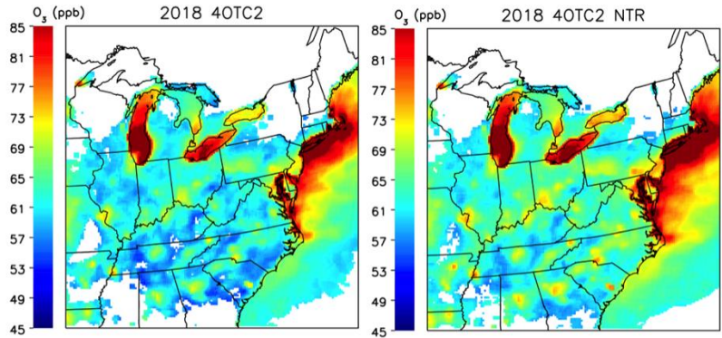
Figure 3.12. Same as Figure 3.7 except baseline and NTR simulations are for Scenario 40TC2
