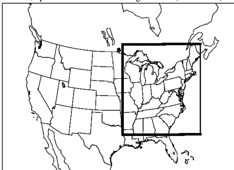
Figure 3b.1. CAMx v6.10 model domain as denoted by the dark black line, 12 km horizontal resolution
