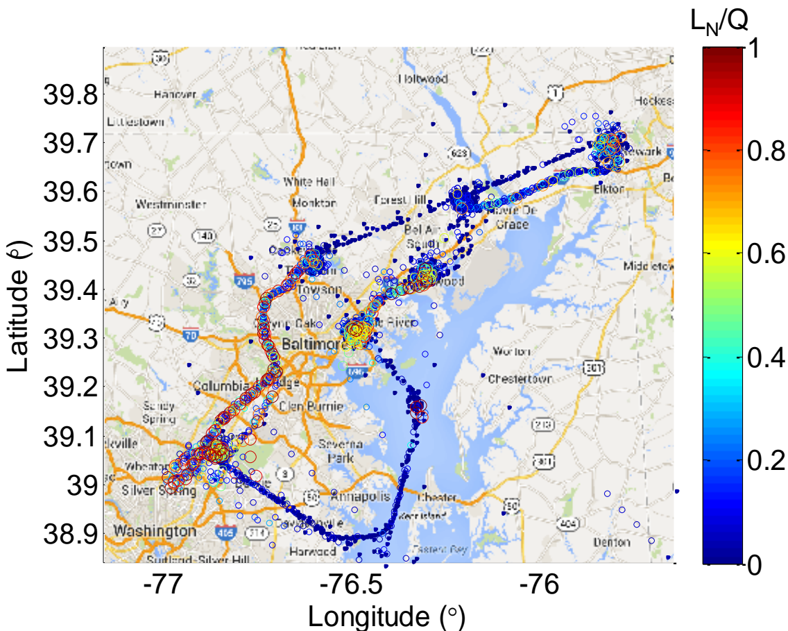
Figure 4.5. Ozone production sensitivity indicator, L_N/Q , along the P-3B flight track during DISCOVER-AQ in Maryland in 2011. P(O_3) is VOC-sensitive when L_N/Q > 0.5 , and NO_x -sensitive when L_N/Q < 0.5 .
