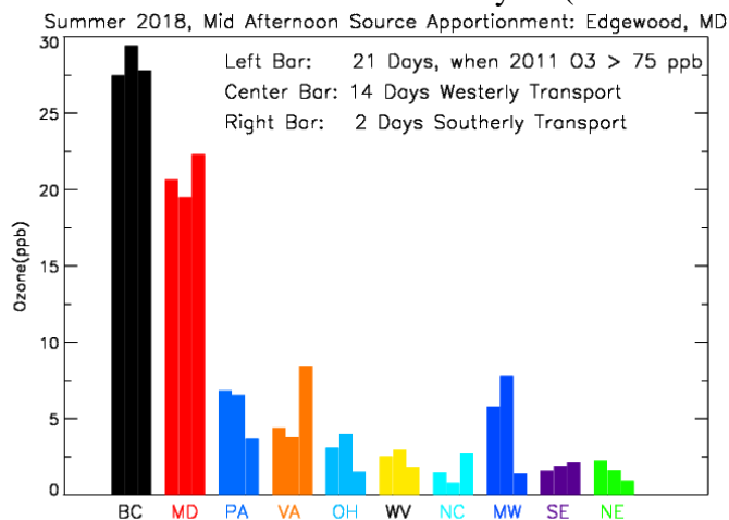
Figure 3b.4. Mid-afternoon source apportionment for ozone at Edgewood, MD from CAMxv6.10 for days when 2011 ozone exceeded 75 ppbv. The left bars show the average of all 21 days, the center bars show the average of 14 days with westerly transport, and the right bars show the average of 2 days with southerly transport.
