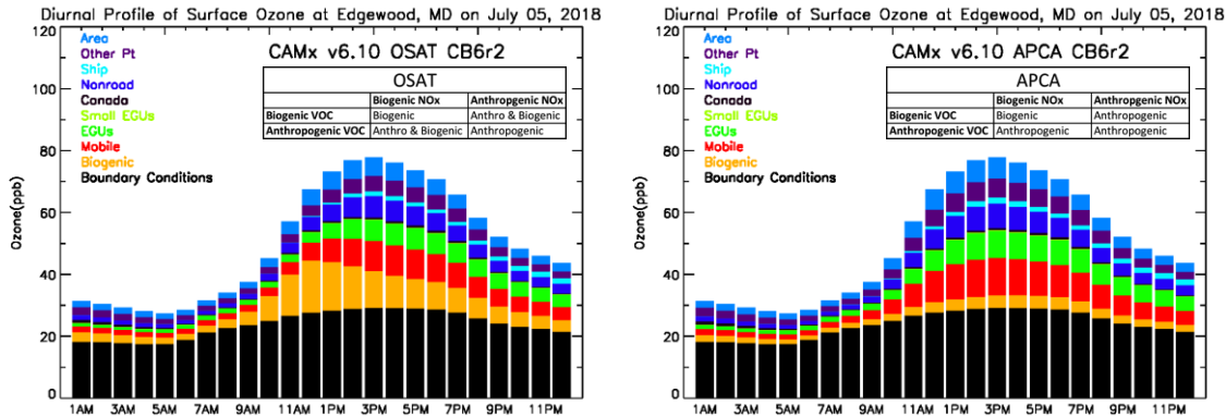
Figure 3b.2. Diurnal pattern of ozone source attribution at the Edgewood, MD site for the July 5, 2018 projected scenario using (left) OSAT and (right) APCA.
