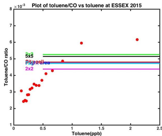
Figure 4.5.1: Plot of toluene to CO ratio as a function of toluene concentration. The red dots show observed concentrations from ESSEX in 2015. The various colored lines denote the modeled ratio from SMOKE across grid cells of varying sizes. For high toluene concentrations, the observed concentration asymptotically approaches (within 20%) the modeled ratios indicating that toluene emissions in SMOKE are reasonable.
