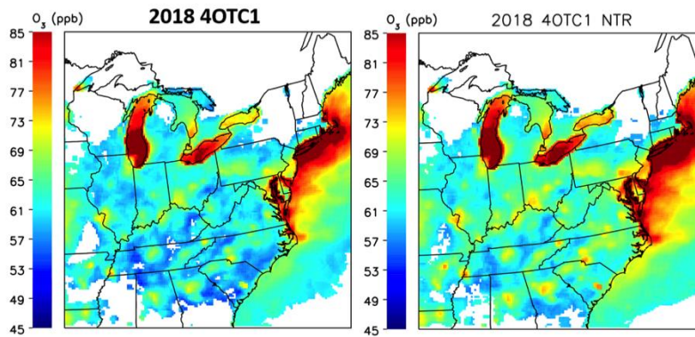
Figure 3.11. Same as Figure 3.7 except baseline and NTR simulations are for Scenario 40TC1
