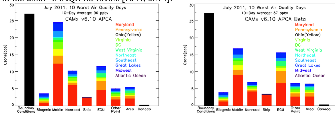
Figure 3b.5. Ozone attributed to source sectors separated by state during the ten worst air quality days in July 2011 at 2 PM local time at the Edgewood, MD monitoring site which is located 30 km east-northeast of Baltimore for the (left) baseline simulation and (right) updated chemistry and emissions scenario.
