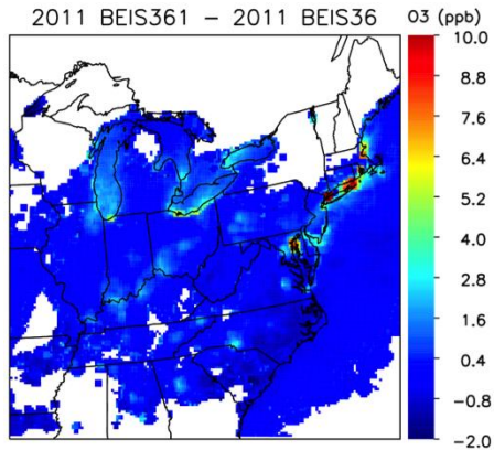
Figure 3.22. The difference in averaged maximum 8hr ozone for July 2011 between two baseline model simulations where biogenic emissions were calculate using either BEIS 3.6 or BEIS 3.61.
