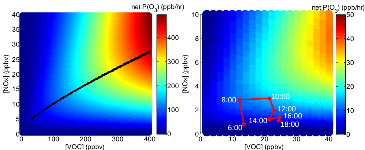
Figure 4.1. Left: ozone production empirical kinetic modeling approach (EKMA) diagram using a box model results with NO x levels varying from 0-40 ppbv and VOC levels from 0-400 ppbv while the mean concentrations of other species and the speciation of NO x and VOCs observed during DISCOVER-AQ in Maryland in 2011 were used to constrain the box model. This diagram clearly shows the sensitivity of ozone production to NO x and VOCs in Maryland. The black line shows the maximum P(O 3 ) at given [NO x ] and [VOC]. Right: a zoom-in P(O 3 ) EKMA diagram with NO x levels varying from 0-10 ppbv and VOC levels from 0-40 ppbv. The red linked dots shows the NO x and VOC levels measured on the NASA P-3B during DISCOVER-AQ 2011 at different times (local standard time) of day.
