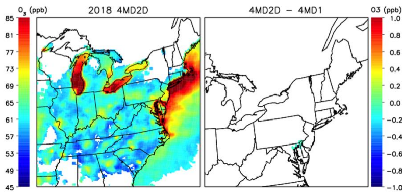
Figure 3.19. Average maximum 8hr O 3 for July 2011 for the 4MD2D attainment CMAQ run (left panel). The expected difference in O 3 between the 4MD2D and 4MD1 runs at the location of surface monitoring sites.
