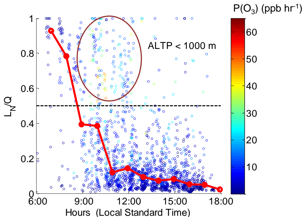
Figure 4.6. Diurnal variations of the indicator L_N/Q of ozone production rate sensitivity colored with ozone production rate and median hourly bins of L_N/Q shown in solid red circles below 1000 m during DISCOVER-AQ in Maryland in 2011.
