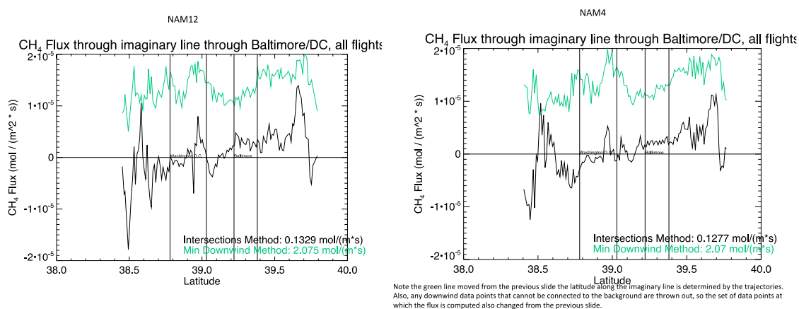
Figure 2B1. Showing 4-km and 12-km estimates of the CH 4 flux from the upwind and wings methods.
