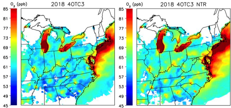
Figure 3.13. Same as Figure 3.7 except baseline and NTR simulations are for Scenario 40TC3
