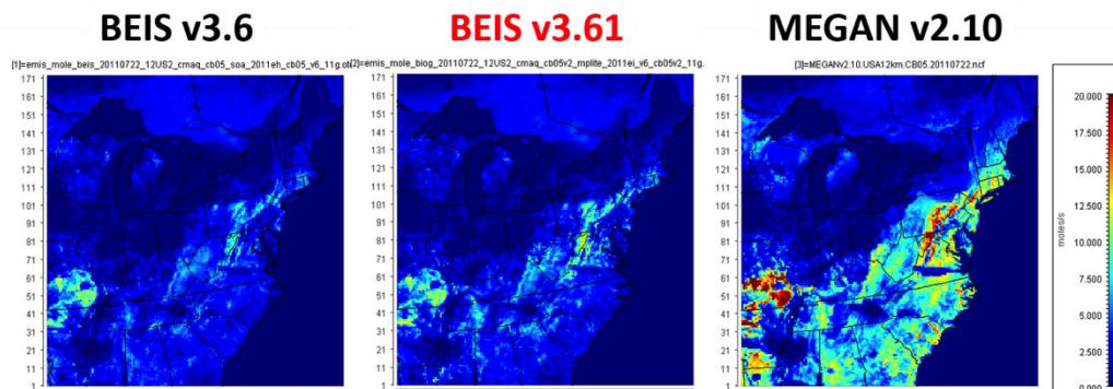
Figure 3.21 Surface isoprene emissions for July 22, 2011 as generated by the BEIS v3.6 (left panel), BEIS v3.61 (center panel), and MEGAN v2.10 (right panel).
