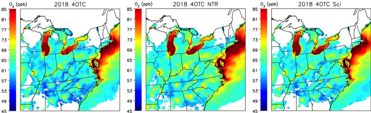
Figure 3.9. Same as Figure 3.4 except all simulations are for July 2018, Scenario 4OTC
