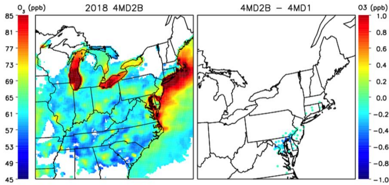
Figure 3.18. Average maximum 8hr O 3 for July 2011 for the 4MD2B attainment CMAQ run (left panel). The expected difference in O 3 between the 4MD2B and 4MD1 runs at the location of surface monitoring sites.
