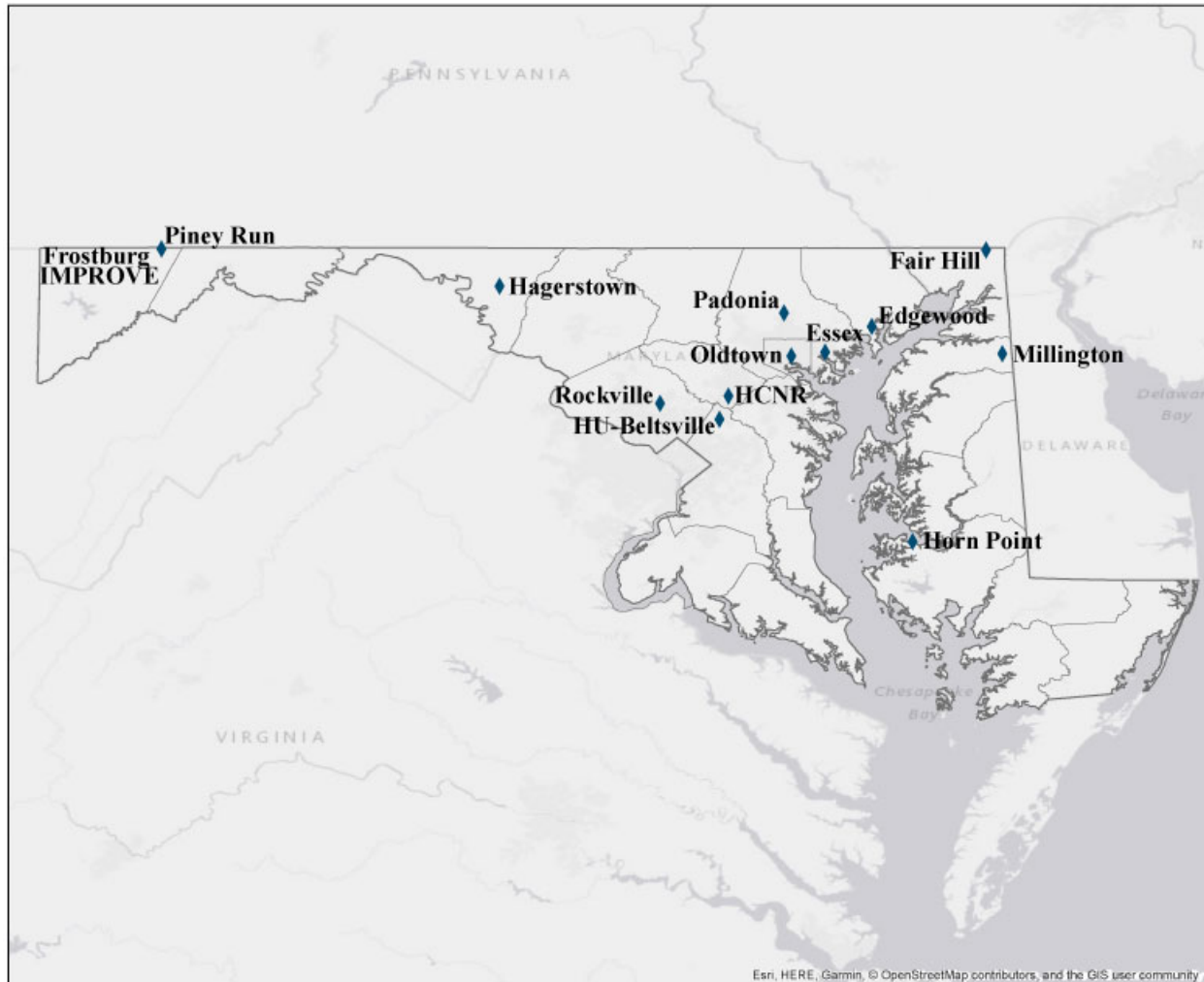
Figure 4-5 Maryland's PM 2.5 monitoring network.
