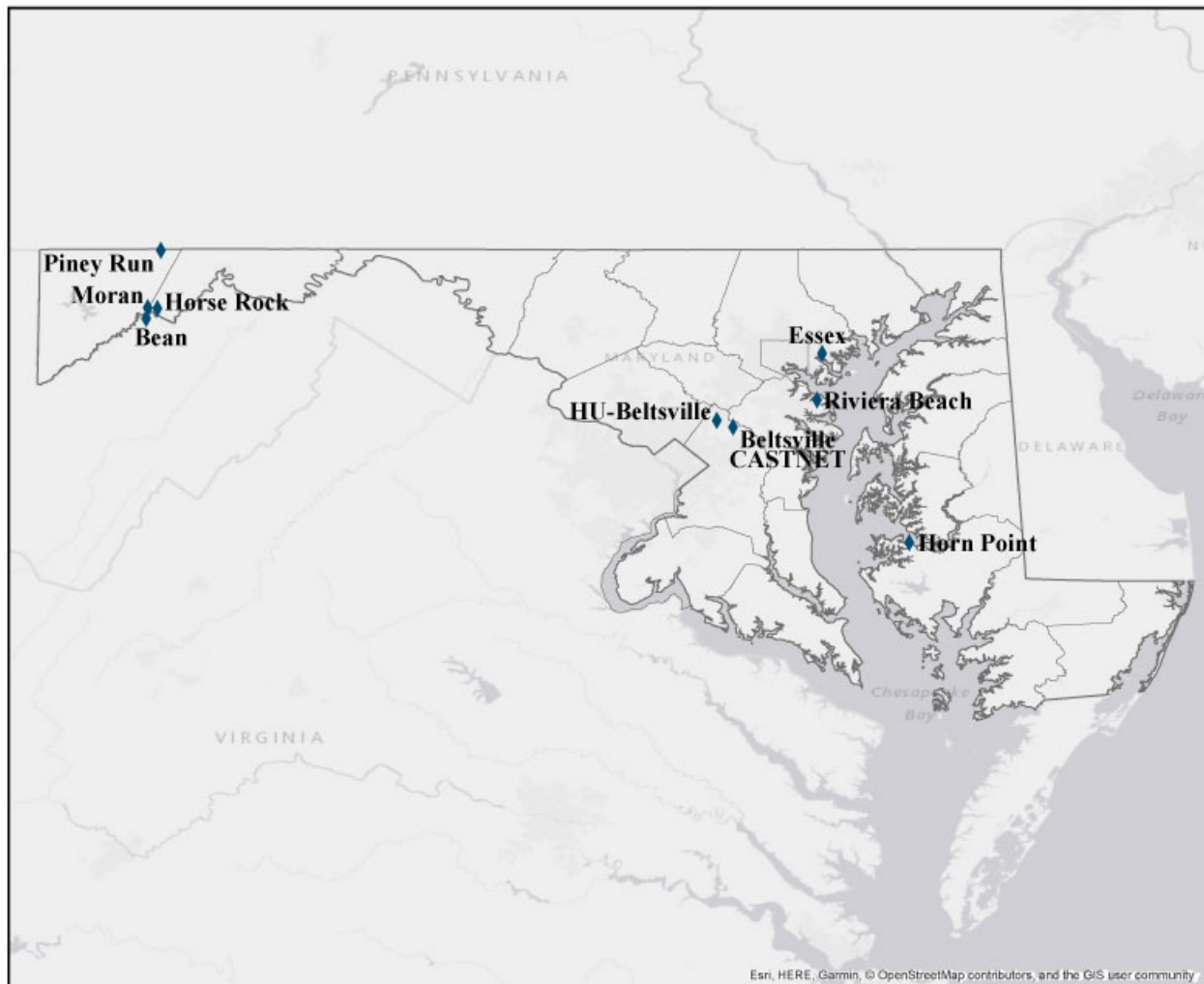
Figure 4-6 Maryland's SO 2 monitoring network.
