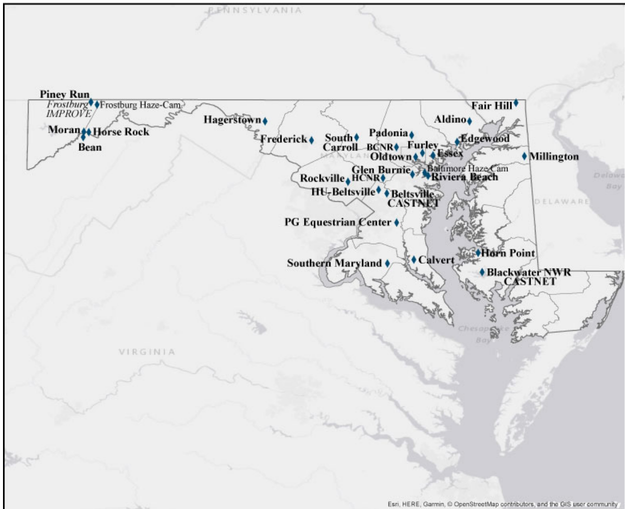
Figure 3-1 Maryland's current air monitoring network map
