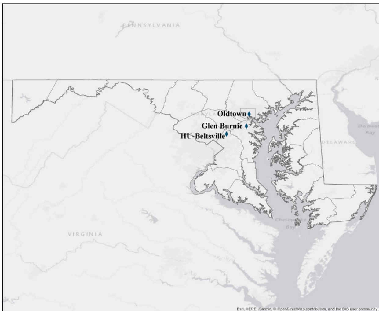
Figure 4-4 Maryland's PM 10 monitoring network.
