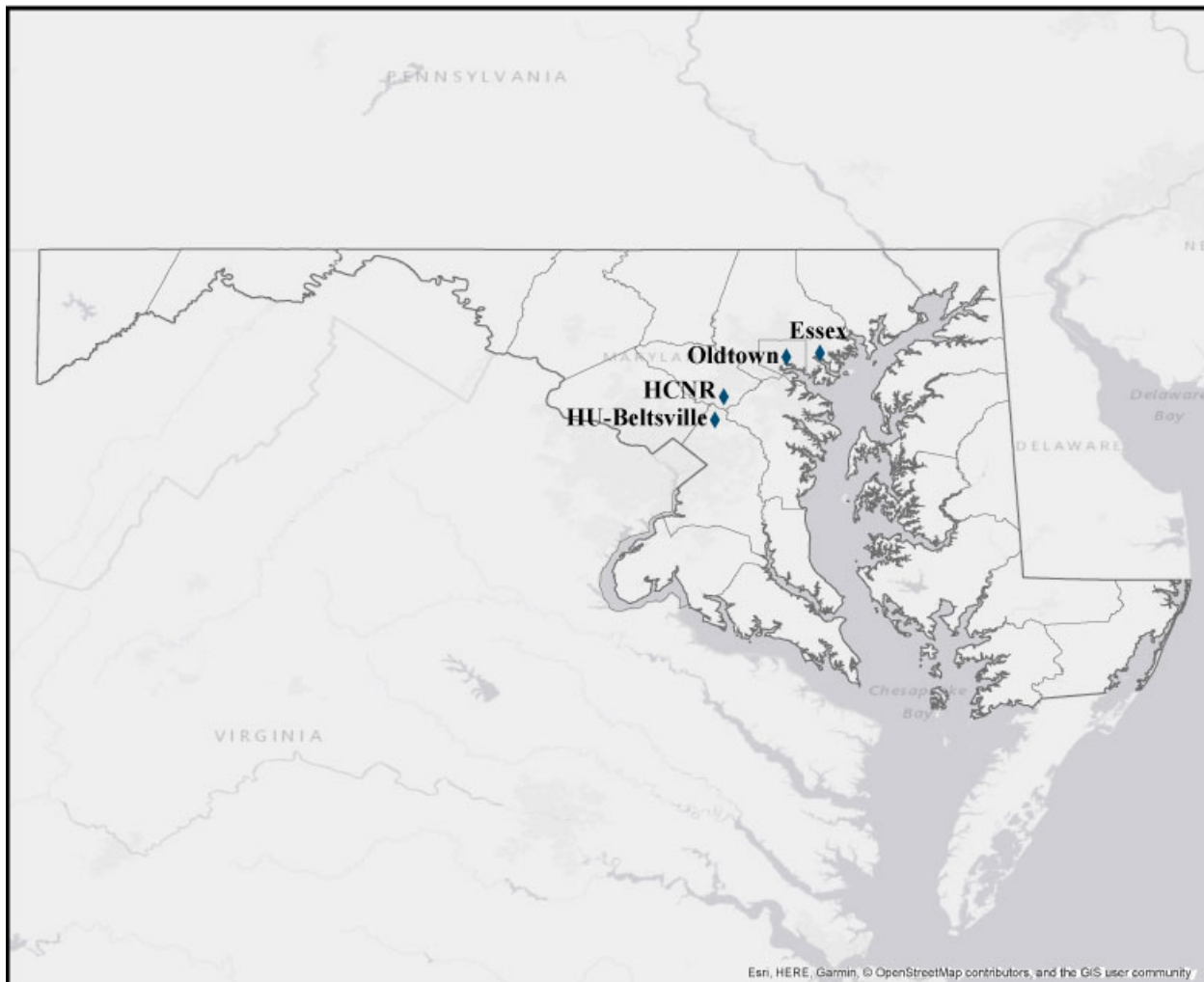
Figure 4-8 Maryland's Air Toxics monitoring network.
