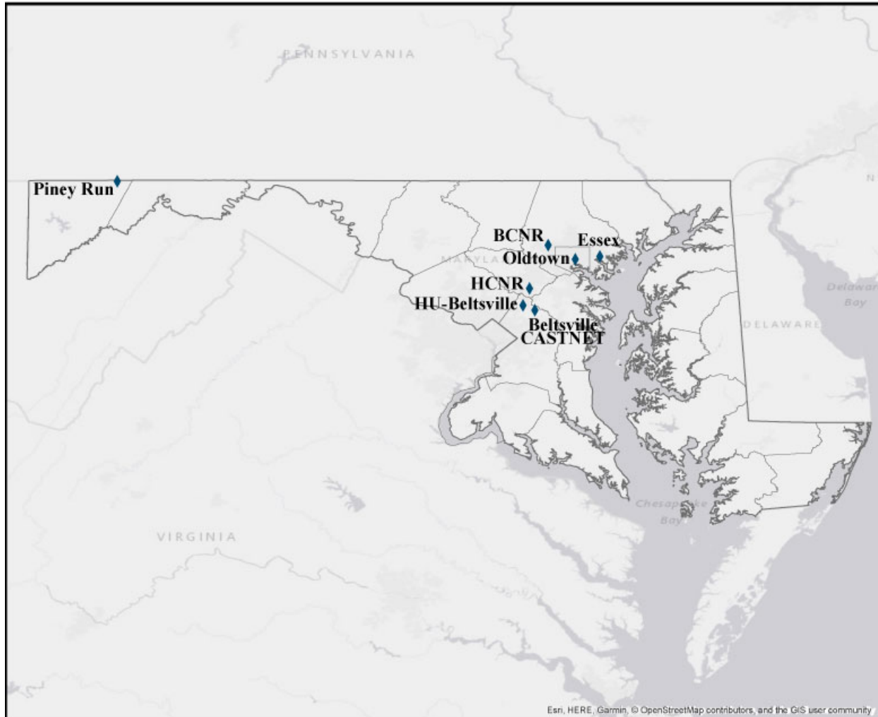
Figure 4-2 Maryland's NO 2 monitoring network.
