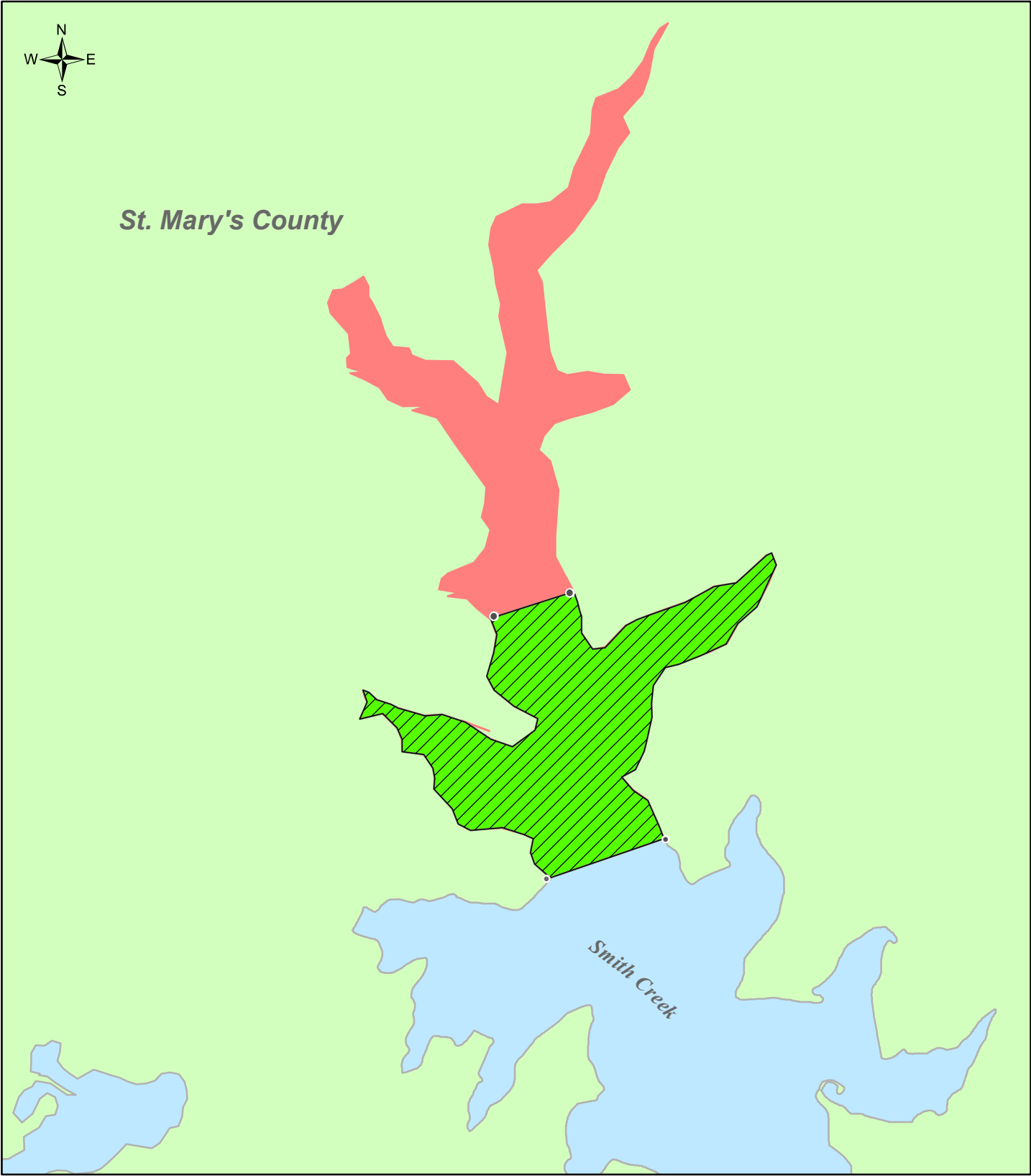
Smith Creek, St. Mary's County Prohibited Shellfish Area Map 4aP May 2022
