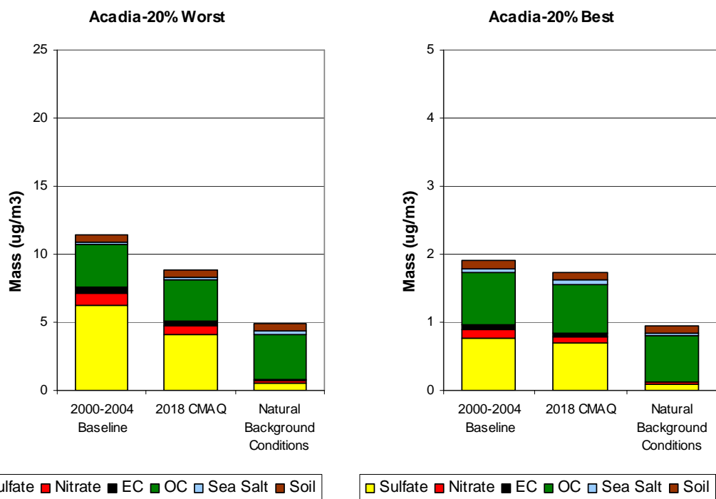
Figure 4-1A-G. Observed Baseline, CMAQ-projected*, and Estimated Natural Speciated PM 2.5 Mass Values for MANE-VU Class I Sites.
